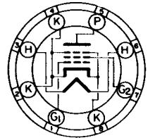
BOTTOM VIEW SUBMINIATURE BUTTON 8 FLEXIBLE LEADS BDL
