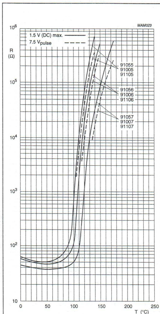
Fig.5 Typical resistance/temperature characteristic for 2322 671 91055/005/105, 91056/006/106 and 91057/007/107.
