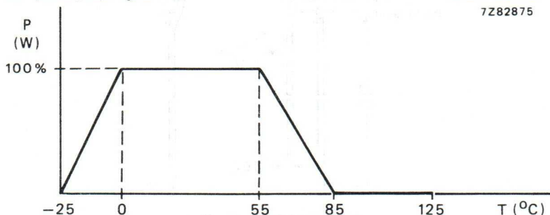
Fig. 2 Derating curve.
