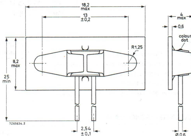
Fig.2 Type 2322 640 98004 with metal strip for mounting.
