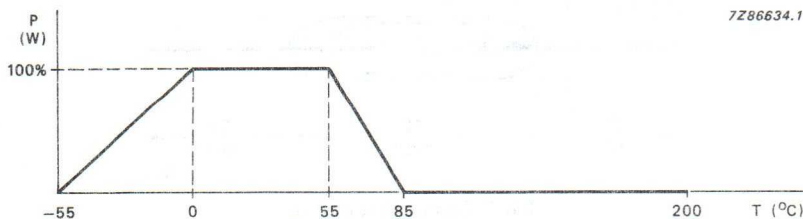
Fig.2 Derating curve.
