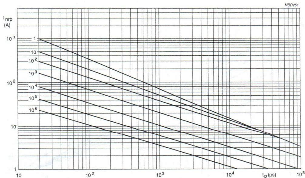
Fig.29 Maximum applicable transient current as a function of pulse duration, 14 V to 40 V (RMS); 2322 595 series.
