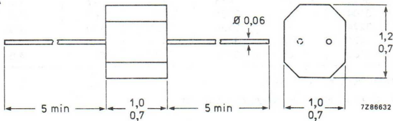
Fig.1 version 2322 633 0.... (axial leads).
