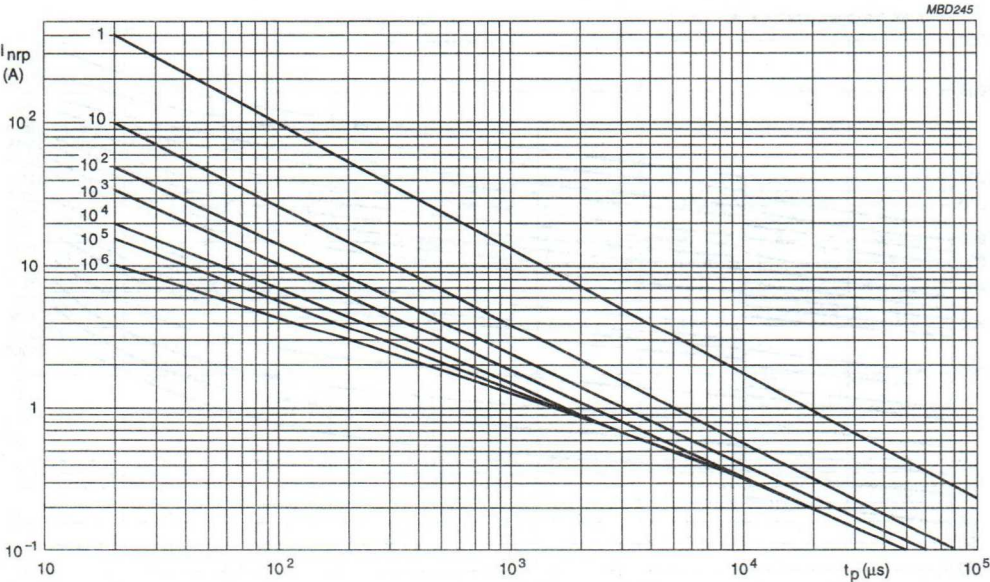
Fig.23 Maximum applicable transient current as a function of pulse duration, 50 V to 460 V (RMS); 2322 592 series.
