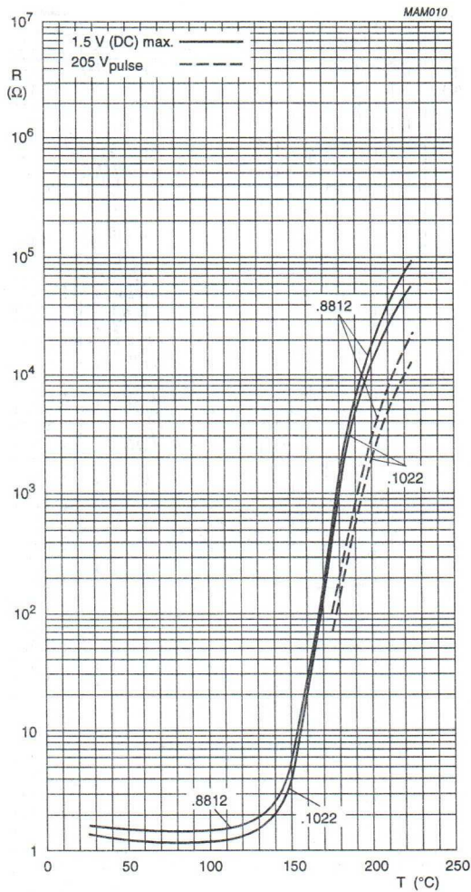
Fig.21 Typical resistance/temperature characteristic for 2322 664 .8812/.1022.
