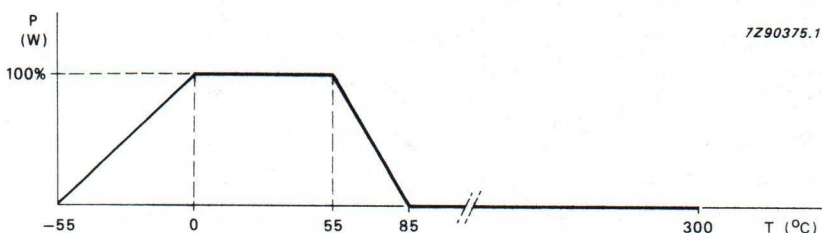
Fig.2 Derating curve.
