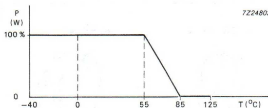
Fig.2 Tolerance curve.
