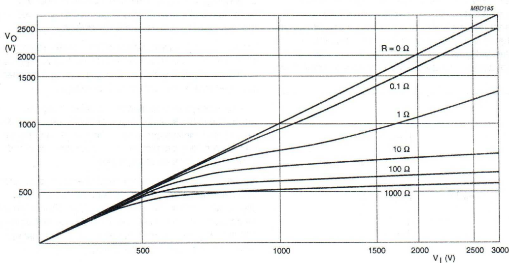
Fig.10 Influence of a series resistance on the varistor.
