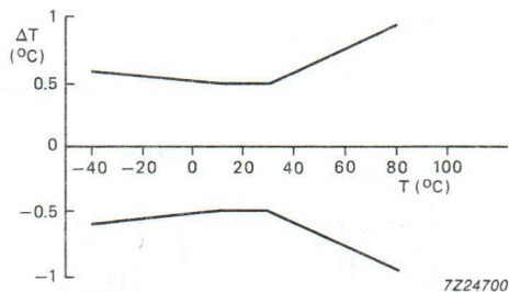
Fig.2 Tolerance curve.
