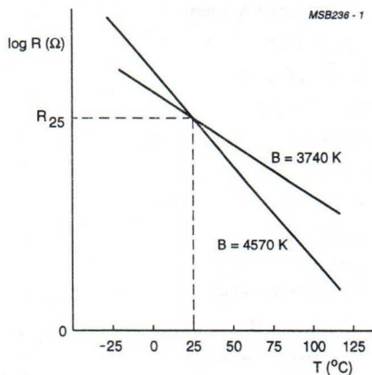
Fig.6 Typical plot of resistance as a function of temperature for an NTC temperature sensor.
