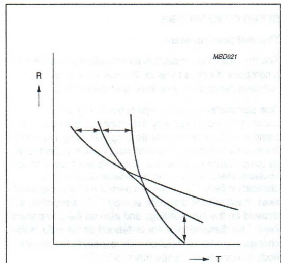
Fig.3 Effect of variations of mechanical dimensions on the resistance as a function of temperature.
