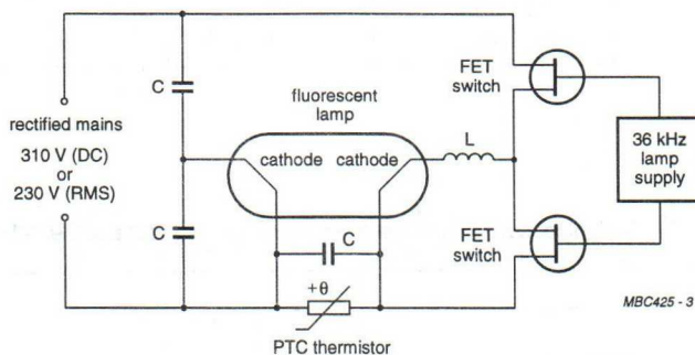
Fig.4 Typical electronic ballast circuit.
