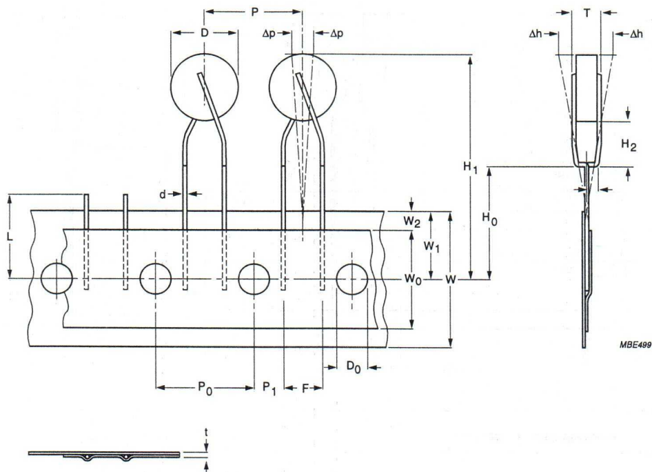
Fig.2 Thermistors with \varnothing D < 12\text{ mm} on tape for 2322 66. 6...0/1/3.
