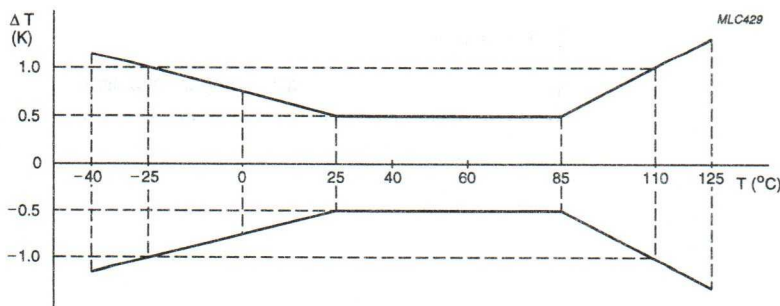
Fig.2 Tolerance curve.
