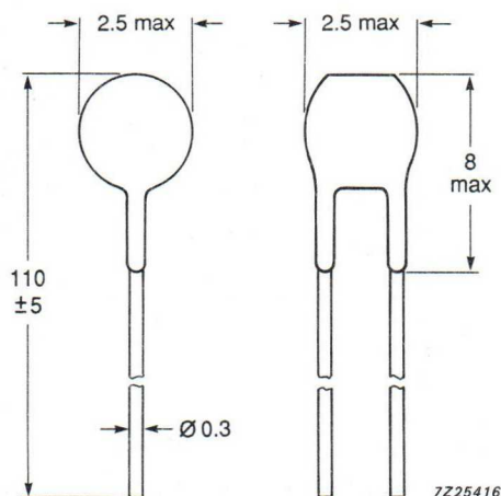
Fig.1 Component outline.
