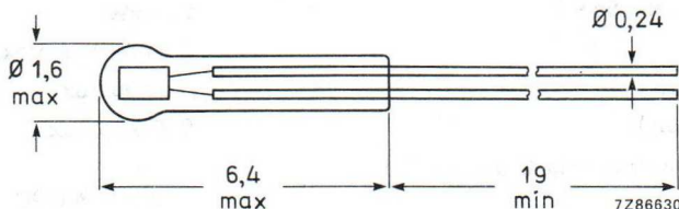
Fig.1 Component outline.
