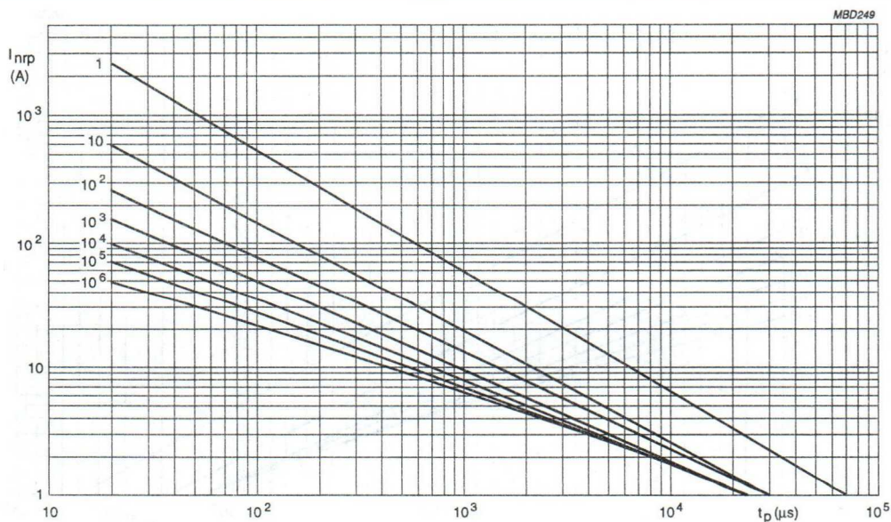
Fig.27 Maximum applicable transient current as a function of pulse duration, 50 V to 320 V (RMS); 2322 594 series.
