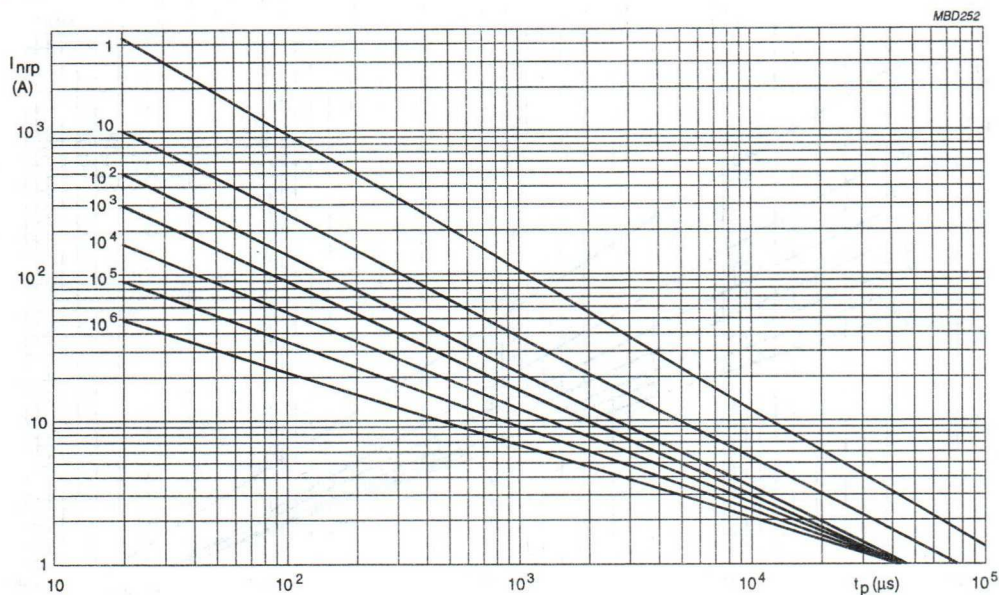
Fig.30 Maximum applicable transient current as a function of pulse duration, 50 V to 320 V (RMS); 2322 595 series.
