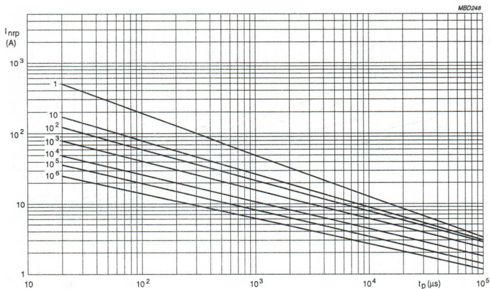
Fig.26 Maximum applicable transient current as a function of pulse duration, 14 V to 40 V (RMS); 2322 594 series.
