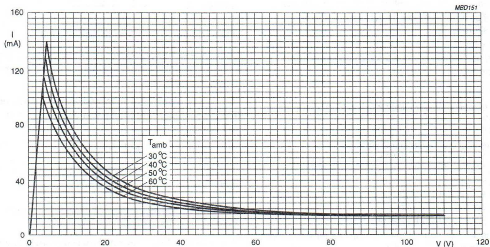
Fig.2 Current/voltage characteristics of a PTC thermistor plotted on a linear scale and using ambient temperature as the parameter.
