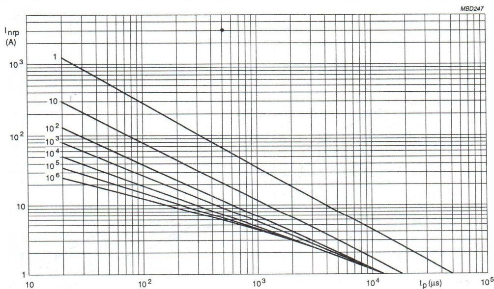
Fig.25 Maximum applicable transient current as a function of pulse duration, 50 V to 460 V (RMS); 2322 593 series.
