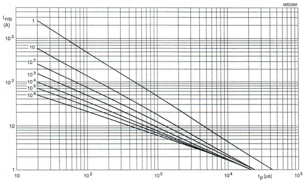
Fig.28 Maximum applicable transient current as a function of pulse duration, 385 V to 550 V (RMS); 2322 594 series.
