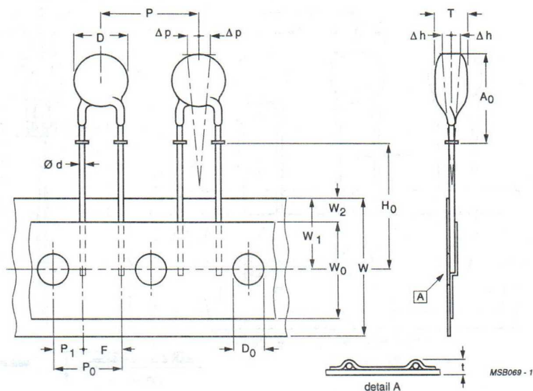
Fig. 7 Taped version with flanged leads (only for 2322 592 and 2322 593 series).
