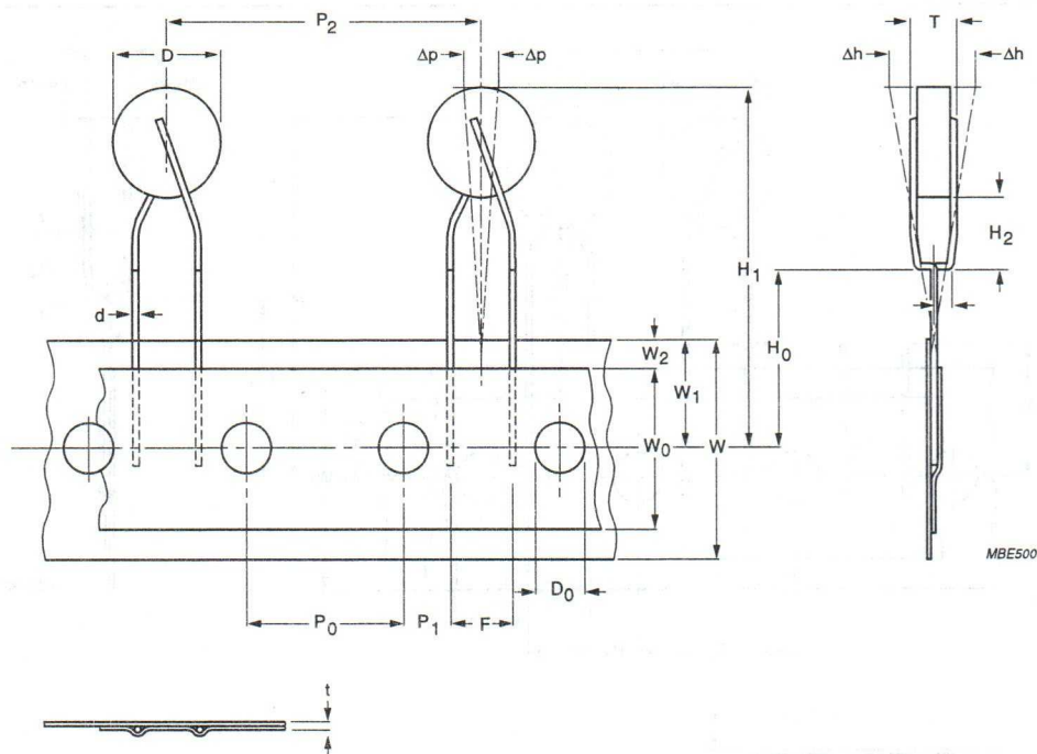
Fig.3 Thermistors with \varnothing D \geq 12\text{ mm} on tape for 2322 66. 6...0/1/3.
