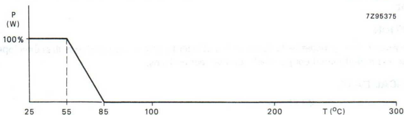
Fig. 2 Derating curve.
