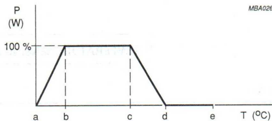
Fig.2 Derating curve; see Table 1 for curve values.
