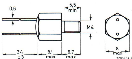
Fig.1 Component outline.
