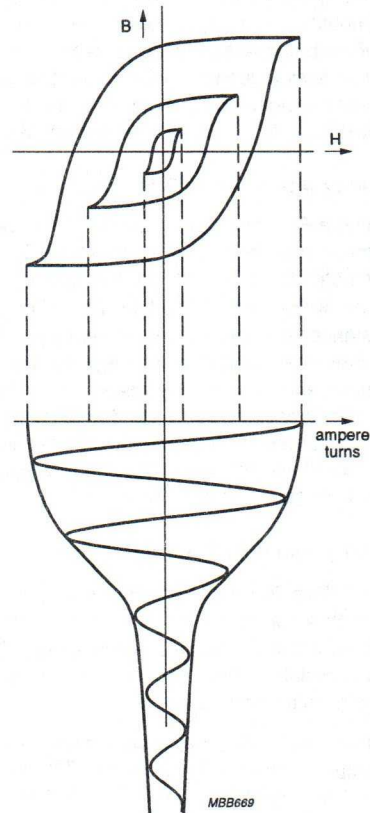
Fig.1 Typical BH curve of shadow mask and corresponding ampere-turns in the degaussing coil.
