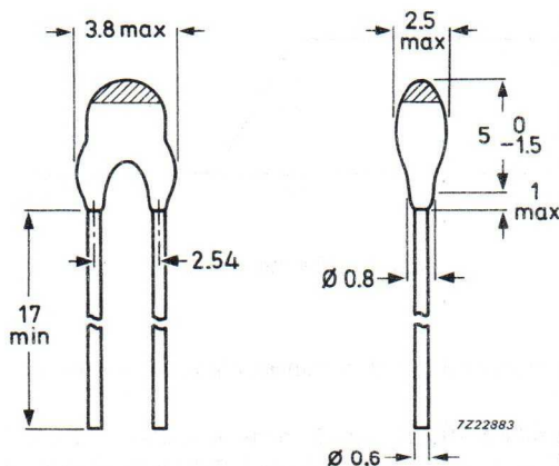
Fig.1 Component outline.
