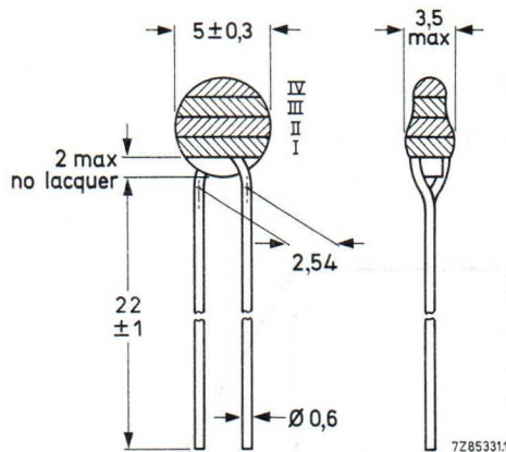
Fig.1 Component outline.
