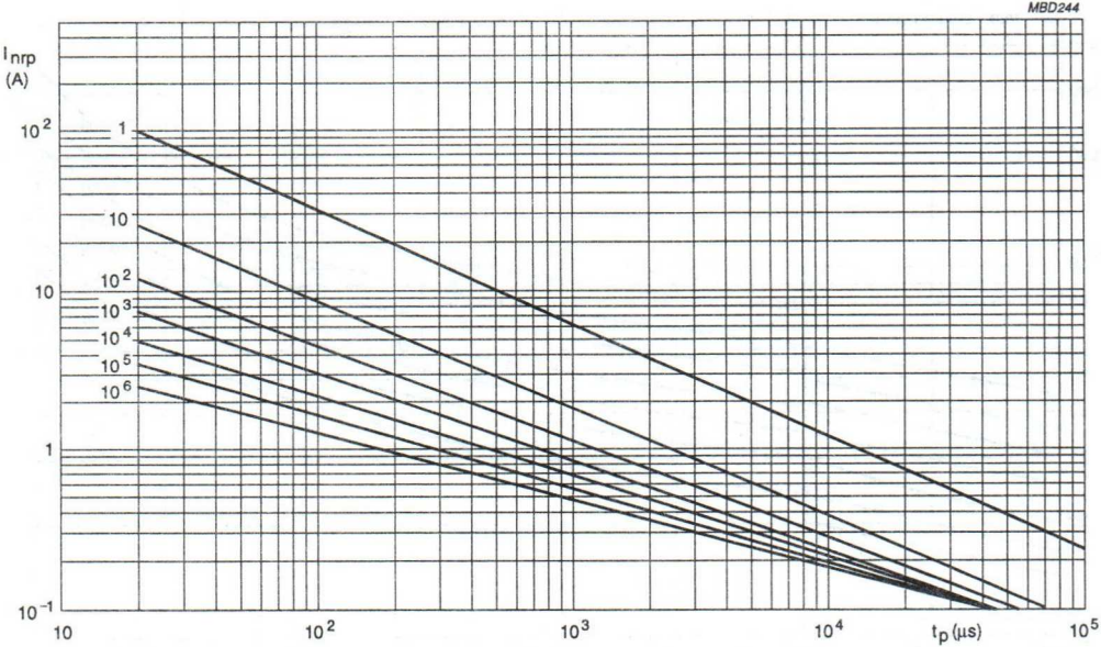
Fig.22 Maximum applicable transient current as a function of pulse duration, 14 V to 40 V (RMS); 2322 592 series.
