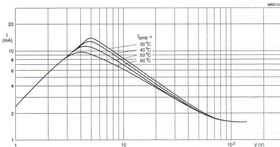
Fig.3 Current/voltage characteristics of a PTC thermistor plotted on a logarithmic scale, using ambient temperature as the parameter.
