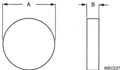
Fig.1 Component outline; see Table 1 for dimensions.
