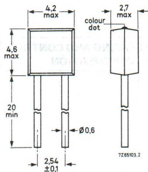
Fig.1 Type 2322 640 98005.
