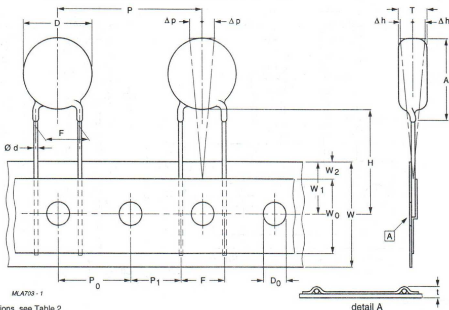
Fig. 6 Taped version with straight leads (only for 2322 594 and 2322 595 series).
