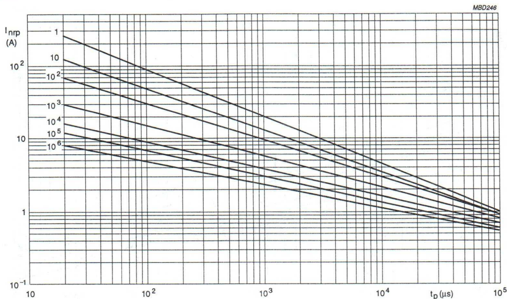
Fig.24 Maximum applicable transient current as a function of pulse duration, 14 V to 40 V (RMS); 2322 593 series.
