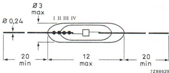
Fig.1 Component outline.
