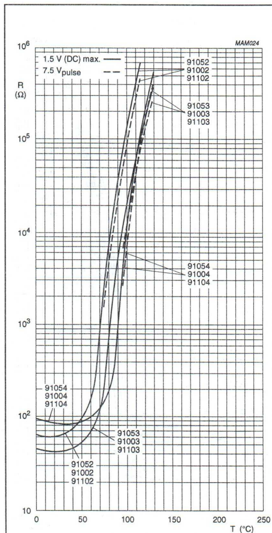
Fig.4 Typical resistance/temperature characteristic for 2322 671 91052/002/102, 91053/003/103 and 91054/004/104.
