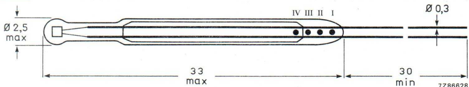
Fig.1 Component outline.
