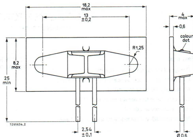
Fig.2 Type 2322 640 98005 with metal strip for mounting.
