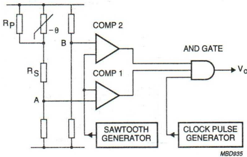
Fig.20 Temperature sensing bridge with 0 °C offset and ADC. Due to R_P and R_S the voltage at A varies linearly with the NTC thermistor temperature. The voltage at B is equal to that at A when the NTC thermistor temperature is 0 °C. Both voltages are fed to the comparator circuit. See also Fig.21.
