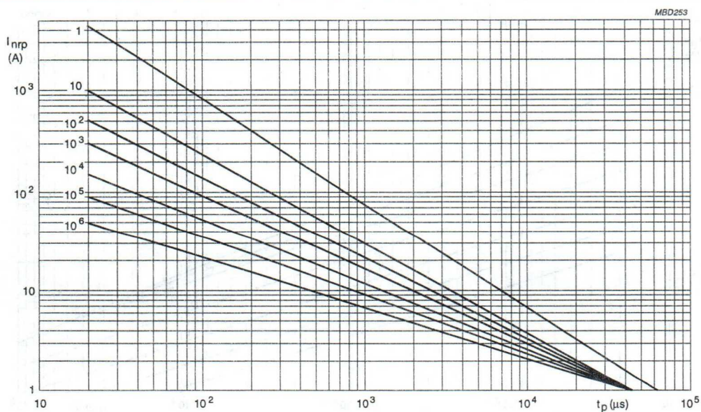
Fig.31 Maximum applicable transient current as a function of pulse duration, 385 V to 550 V (RMS); 2322 595 series.
