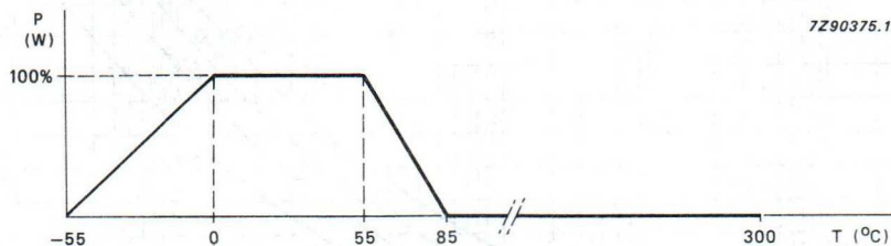
Fig.2 Derating curve.
