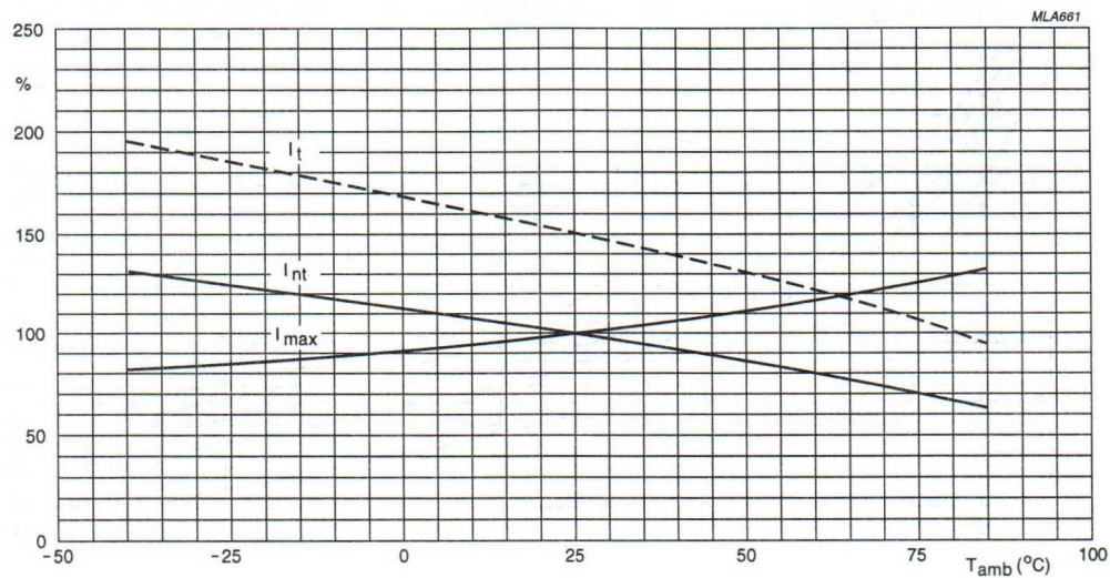
Fig.7 Current deviation as a function of the ambient temperature.
