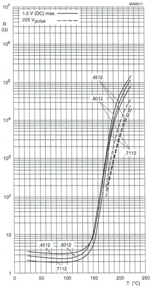
Fig.20 Typical resistance/temperature characteristic for 2322 662 .4512 and 663 .6012/.7112.
