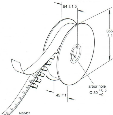
Fig.4 Reel with capacitors on tape.
