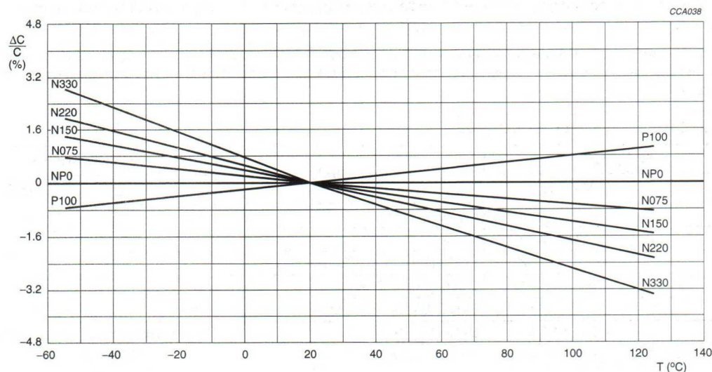
Fig.1 Capacitance change as a function of temperature.
