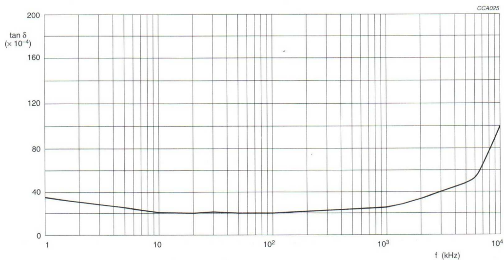
Fig.6 Typical \tan \delta as a function of frequency.
