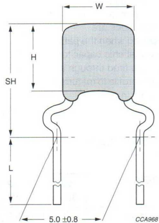
Fig.5 Component outline for lead spacing 5.0 \pm 0.8 mm (outside kink wires).
