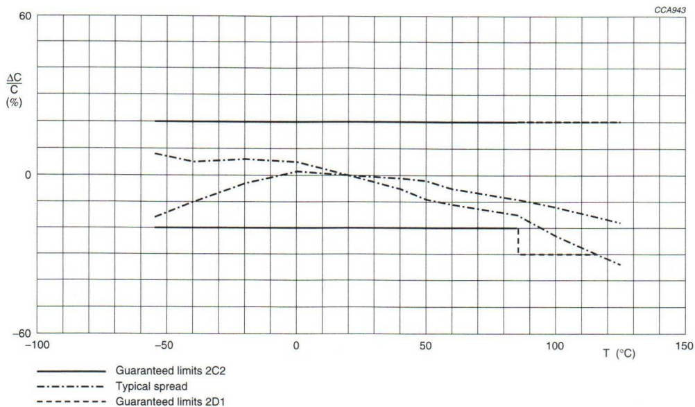
Fig.5 Typical capacitance change with respect to capacitance value at 20 °C as a function of temperature.
