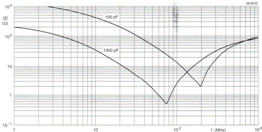
Fig.6 Typical impedance |Z| as a function of frequency.
