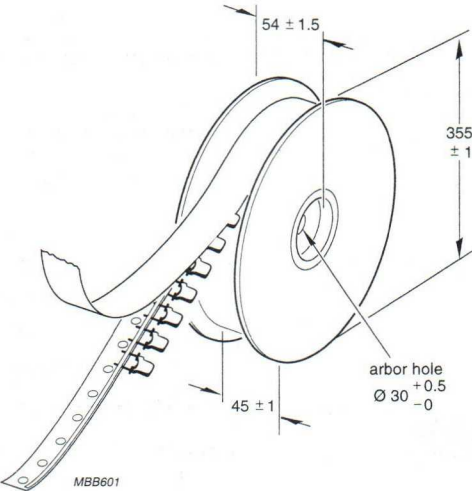
Fig.9 Reel with capacitors on tape.
