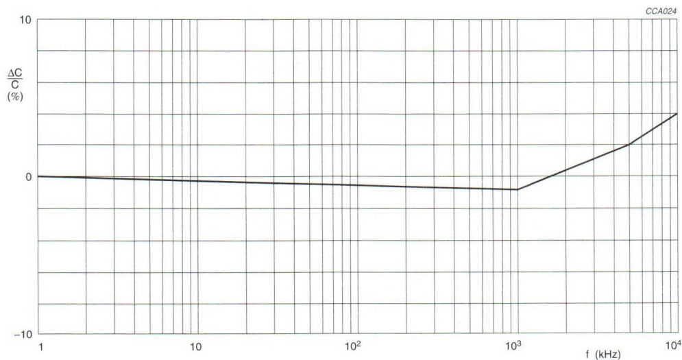
Fig.5 Typical capacitance change as a function of frequency.
