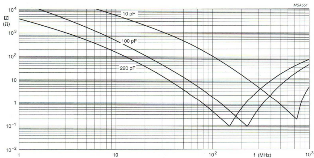
Fig.7 Typical impedance |Z| as a function of frequency.
