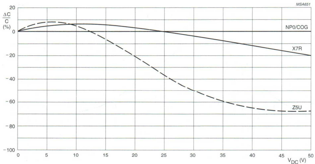
Fig.9 Typical capacitance change as a function of DC voltage.
