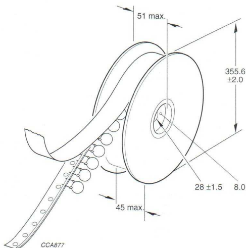
Fig.4 Reel with capacitors on tape.
