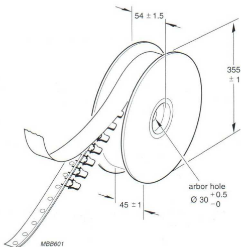
Fig.5 Reel with capacitors on tape.
