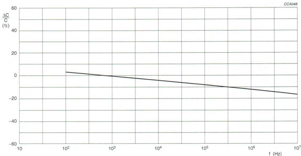
Fig.5 Typical capacitance change with respect to the capacitance at 1 kHz as a function of frequency.
