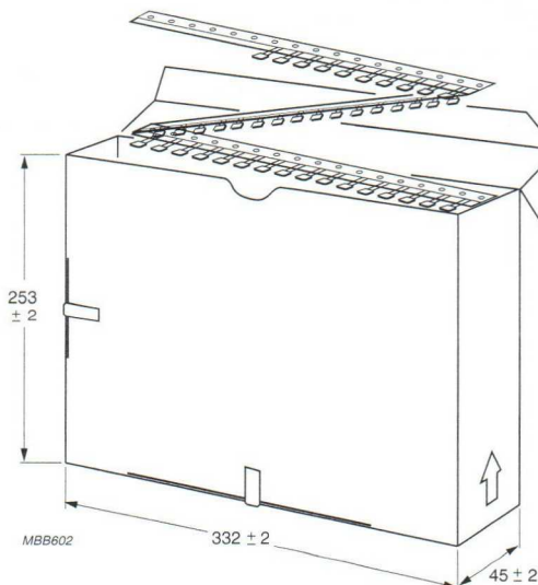
Fig.5 Ammpack with capacitors on tape.
