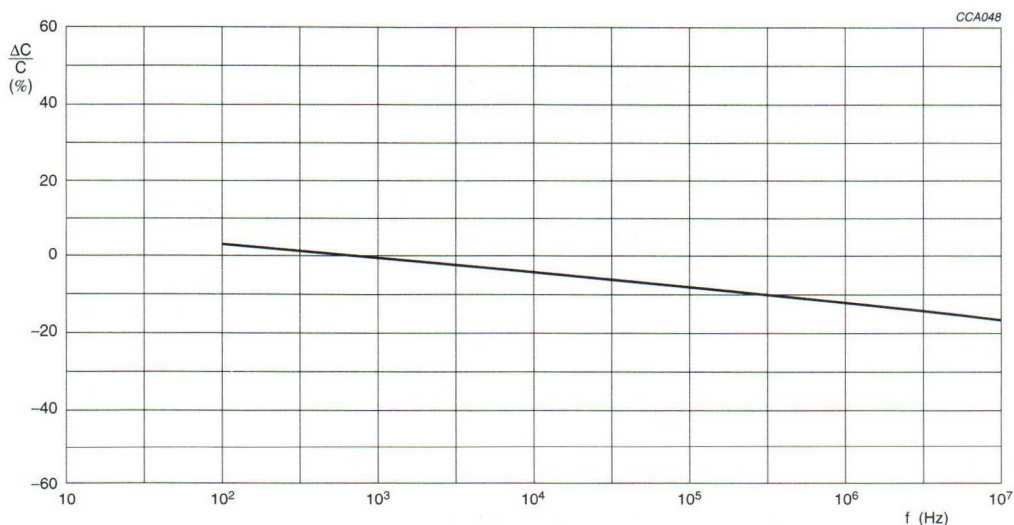
Fig.6 Typical capacitance change with respect to the capacitance value at 1 kHz as a function of frequency.
