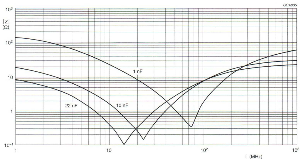
Fig.20 Typical impedance |Z| as a function of frequency.
