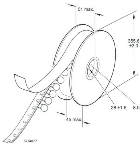
Fig.8 Reel with capacitors on tape.
