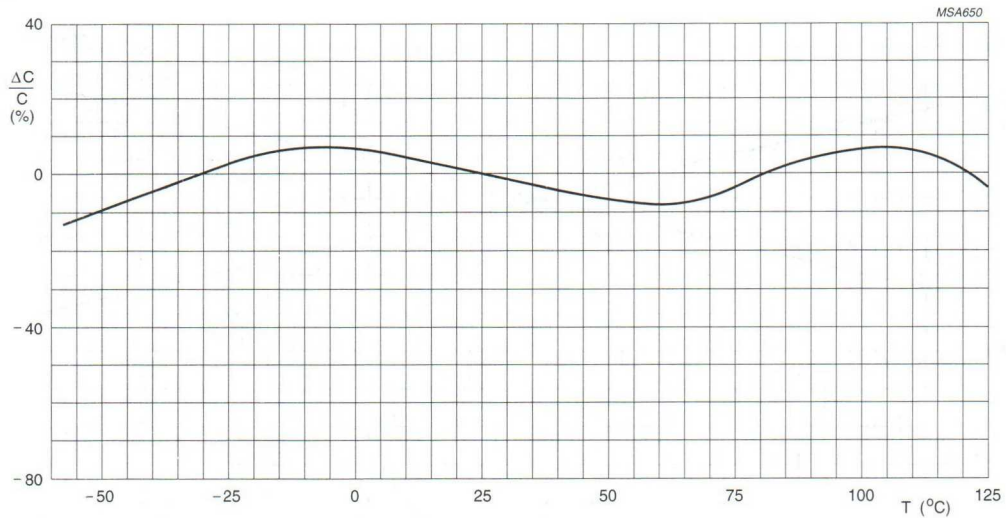
Fig.8 Typical capacitance change as a function of temperature.
