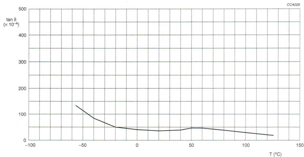
Fig.7 Typical \tan \delta as a function of temperature.
