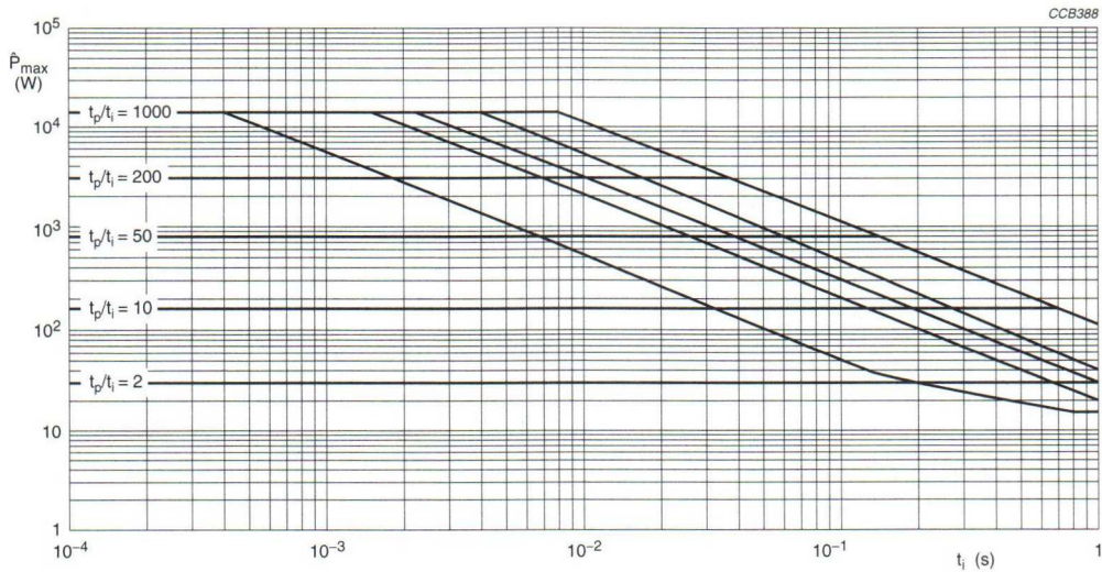
Fig.20 Pulse on a regular basis; maximum permissible peak pulse power ( \hat{P}_{max} ) as a function of pulse duration ( t_i ).
