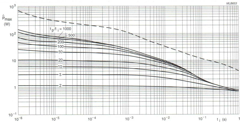
Fig.6 Pulse on a regular basis; maximum permissible peak pulse power ( \hat{P}_{max} ) as a function of pulse duration ( t_i ).
