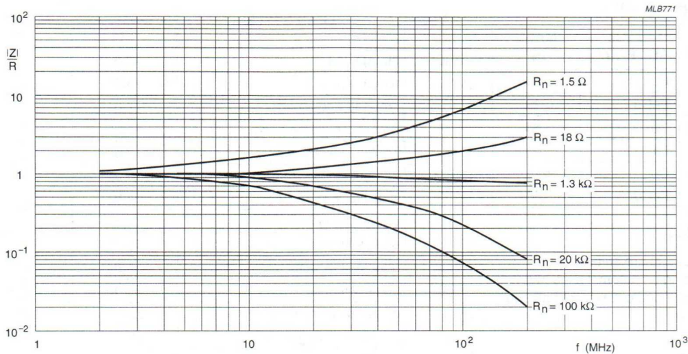
Fig.38 Impedance as a function of applied frequency.
