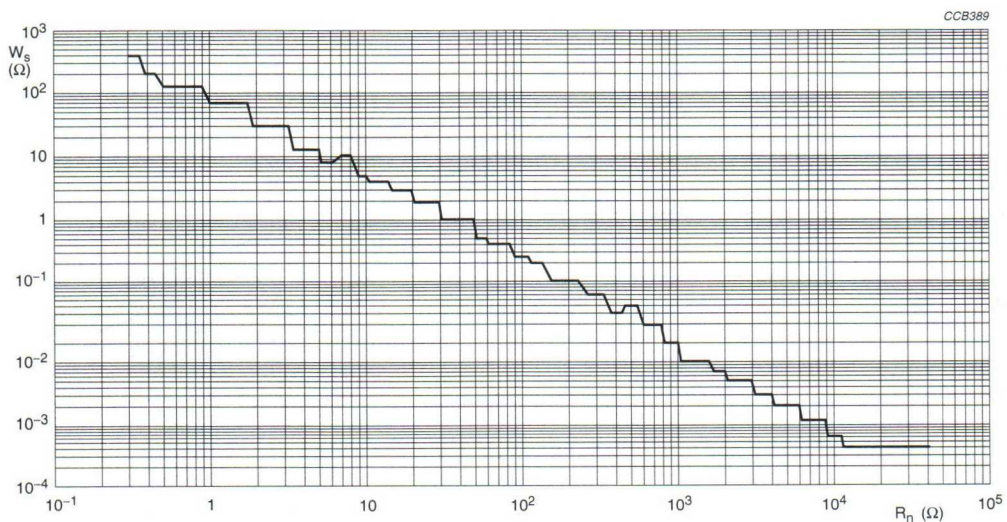
Fig.21 Pulse capability; W_s as a function of R_n .
