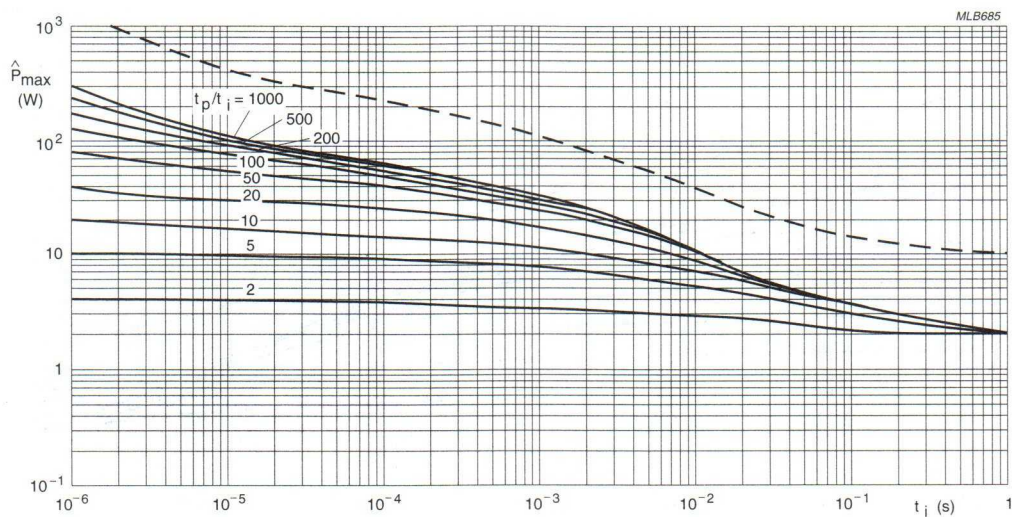
Fig.7 Pulse on a regular basis; maximum permissible peak pulse power ( \hat{P}_{max} ) as a function of pulse duration ( t_i ).
