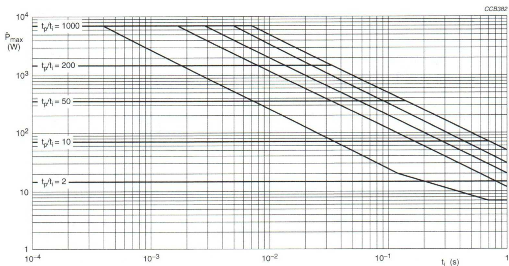
Fig.14 Pulse on a regular basis; maximum permissible peak pulse power ( \dot{P}_{\max} ) as a function of pulse duration ( t_i ).
