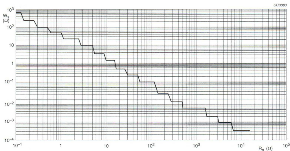
Fig.15 Pulse capacity; W_s as a function of R_n .
