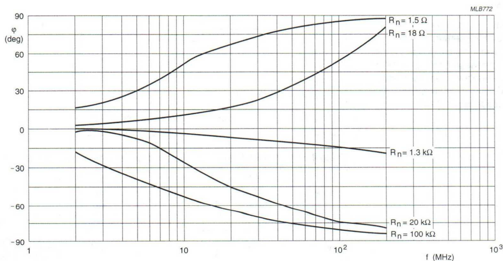
Fig.39 Phase angle as a function of applied frequency.
