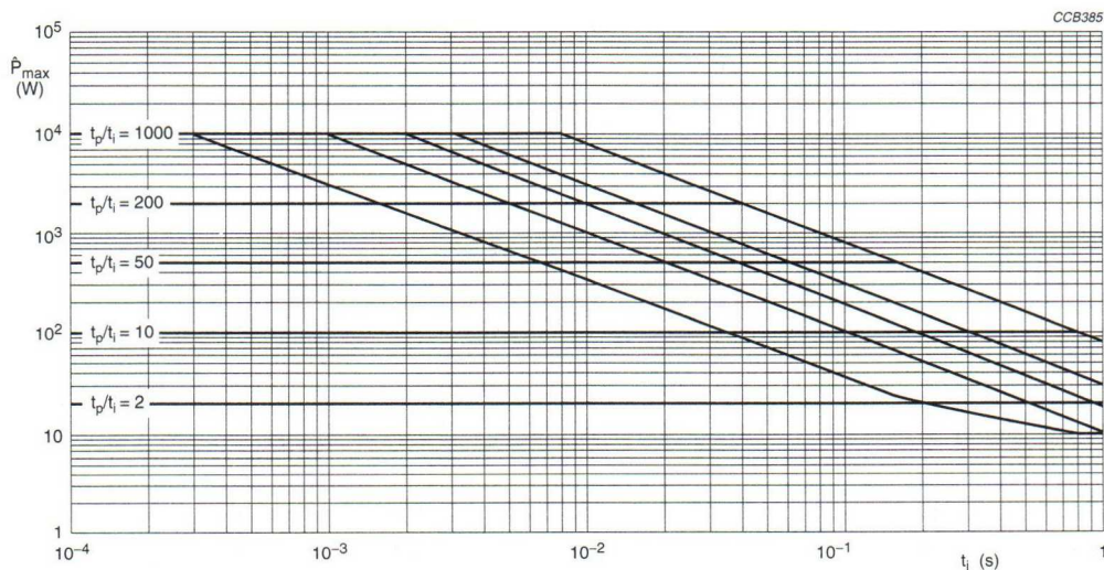
Fig. 17 Pulse on a regular basis; maximum permissible peak pulse power ( \hat{P}_{\max} ) as a function of pulse duration ( t_i ).
