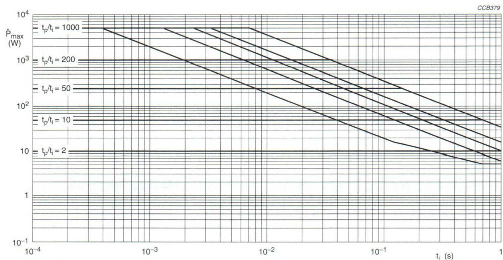
Fig.11 Pulse on a regular basis; maximum permissible peak pulse power ( \hat{P}_{\max} ) as a function of pulse duration ( t_i ).
