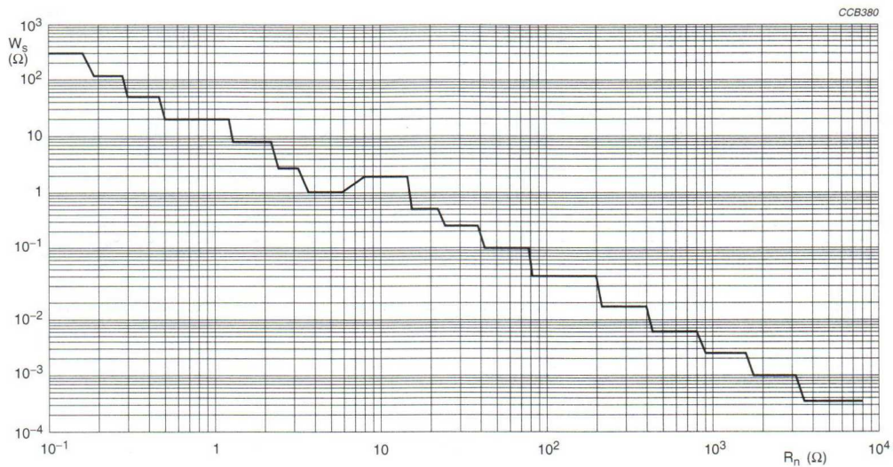
Fig.12 Pulse capacity; W_s as a function of R_n .
