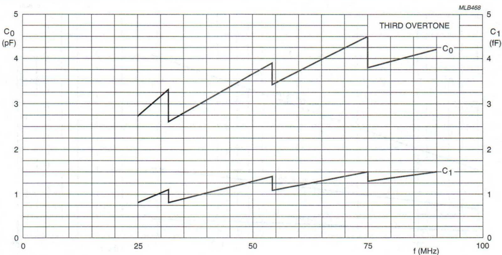
Fig.12 Motional capacitance C_1 and parallel capacitance C_0 as a function of resonance frequency, for HC-45/U crystals in 8 mm product height (involving large quartz blanks).
