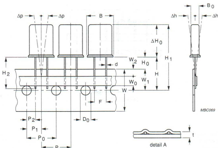
Fig.3 Style 2a and 2b: HC-49/L and HC-49/S on tape.
