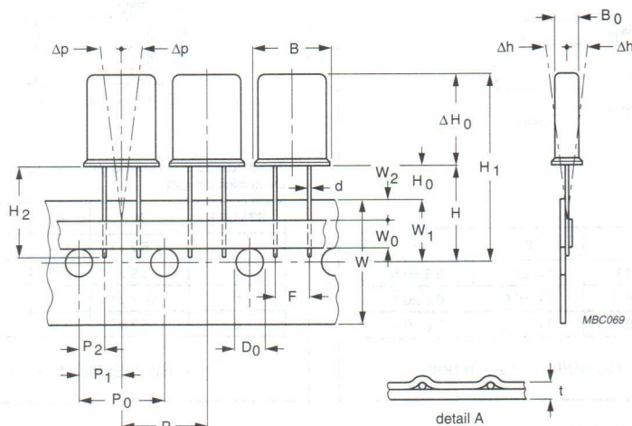
Fig.9 Style 2: HC-49/U on tape.
