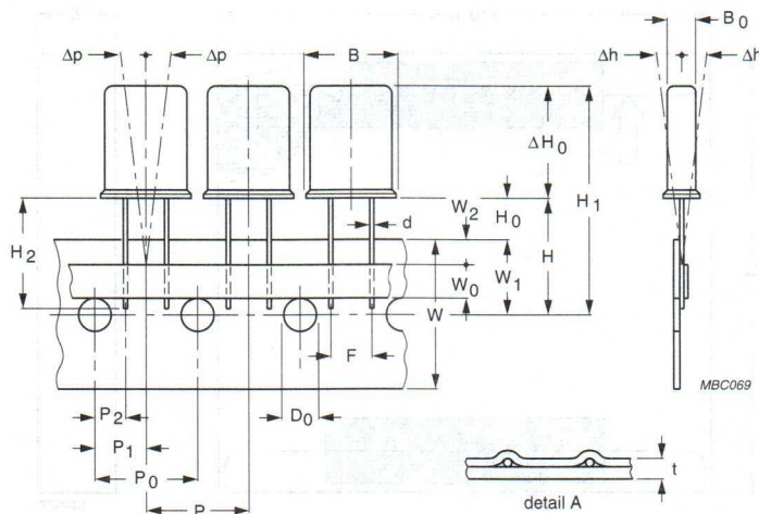
Fig.3 Style 2a and 2b: HC-45/U on tape.
