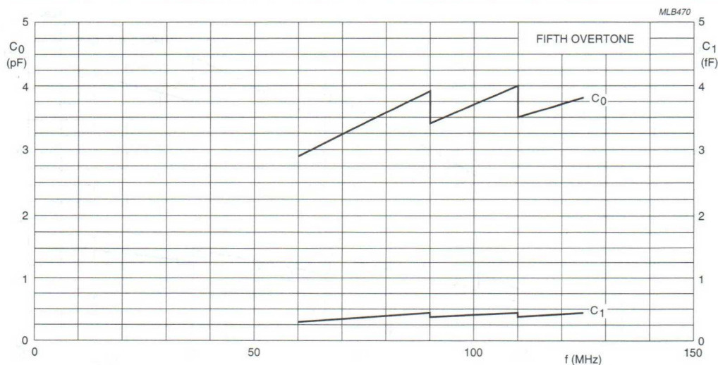
Fig.13 Motional capacitance C_1 and parallel capacitance C_0 as a function of resonance frequency, for HC-45/U crystals in 8 mm product height (involving large quartz blanks).
