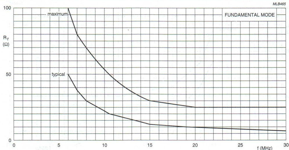
Fig.6 Resonance resistance R_r as a function of resonance frequency, for HC-45/U crystals in 12 mm product length (involving large quartz blanks).
