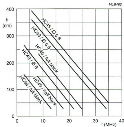
Fig.16 Typical height of fall values (3× on hard wood) for various quartz blank and holder combinations. 'Full' and 'half' blanks refer to rectangular quartz designs; 'Ø' designates circular quartz designs and the appropriate diameter.
