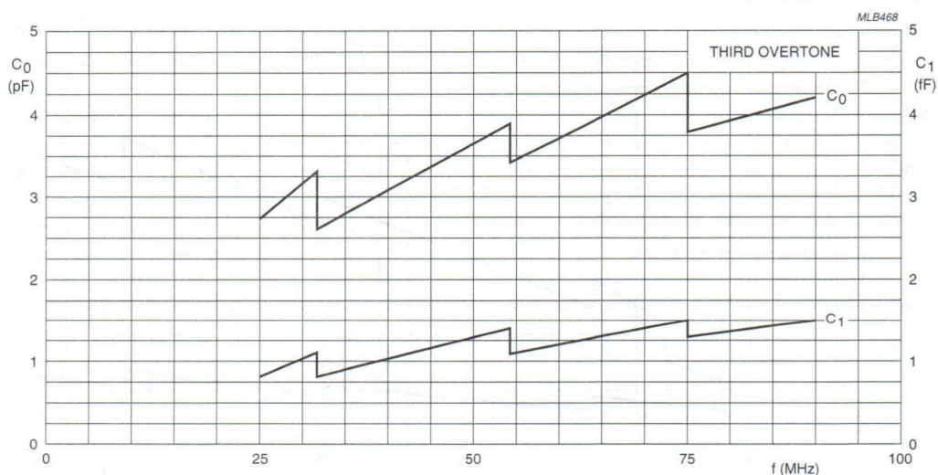
Fig.9 Motional capacitance C_1 and parallel capacitance C_0 as a function of resonance frequency, for HC-45/U crystals in 12 mm product length (involving large quartz blanks).
