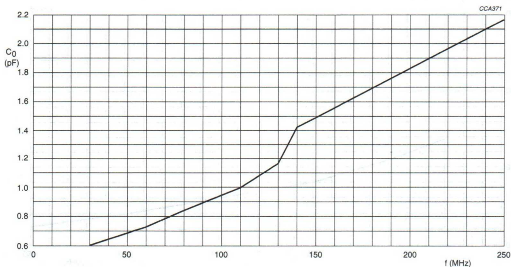
Fig. 4 Typical parallel capacitance C 0 as a function of frequency.
