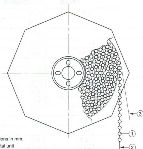
Fig.4 Style 2a and 3a units on tape in ammpack.
