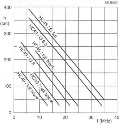
Fig.13 Typical height of fall values (3× on hard wood) for various quartz blank and holder combinations. 'Full' and 'half' blanks refer to rectangular quartz designs; 'Ø' designates circular quartz designs and the appropriate diameter.
