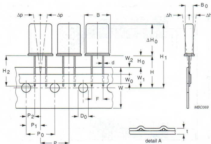
Fig.6 Style 2a and 2b: HC-49/U on tape.
