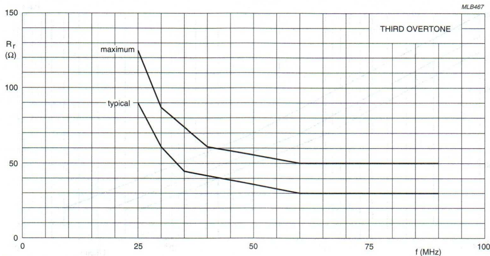
Fig.12 Resonance resistance R_r as a function of resonance frequency, for HC-45/U crystals in 8 mm product height (involving large quartz blanks).
