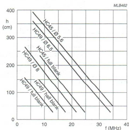
Fig.10 Typical height of fall values (3x on hard wood) for various quartz blank and holder combinations. 'Full' and 'half' blanks refer to rectangular quartz designs; 'Ø' designates circular quartz designs and the appropriate diameter.
