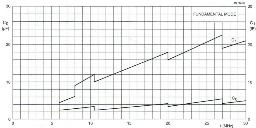
Fig.7 Motional capacitance C_1 and parallel capacitance C_0 as a function of resonance frequency, for HC-45/U crystals in 12 mm product length (involving large quartz blanks).
