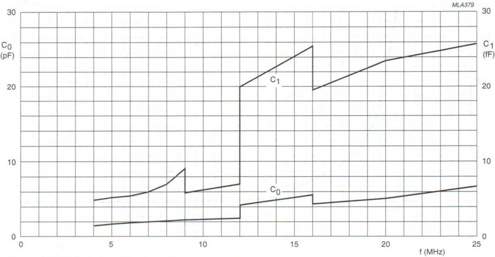
HC-26/U and HC-29/U in the fundamental mode (for other modes see Table 3). Typical values at 25 °C. Other values available on request.
