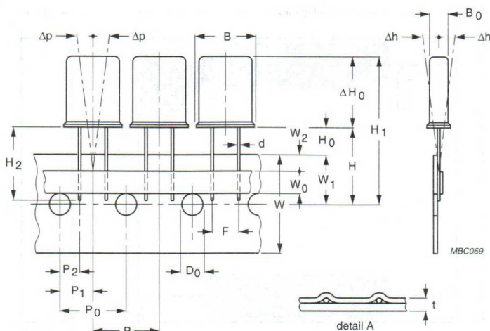
Fig.2 Style 2a and 2b: HC-45/U on tape.
