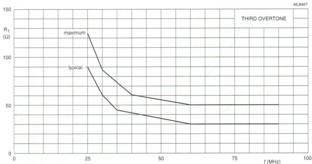
Fig.8 Resonance resistance R_r as a function of resonance frequency, for HC-45/U crystals in 12 mm product length (involving large quartz blanks).
