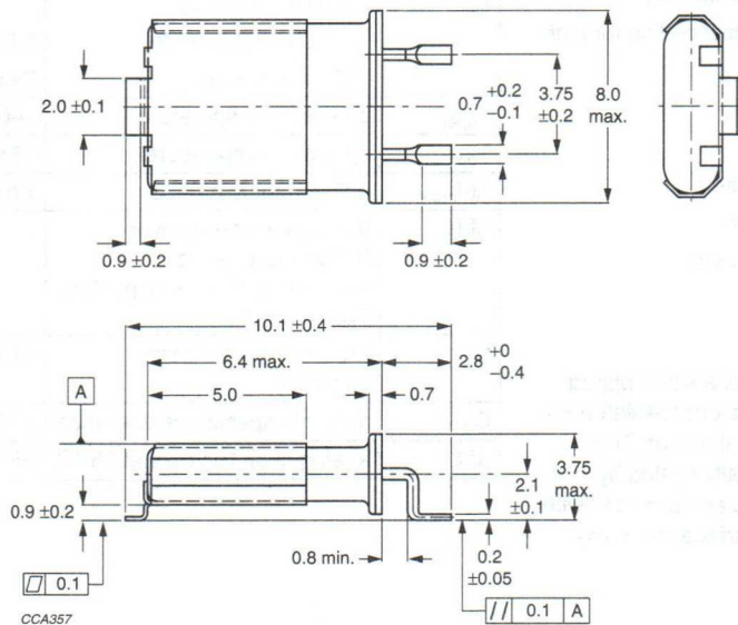
Fig.1 Style 1: HC-45/U10-SMD/Clip I.
