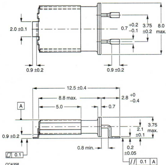
Fig.2 Style 2: HC-45/U12-SMD/Clip I.
