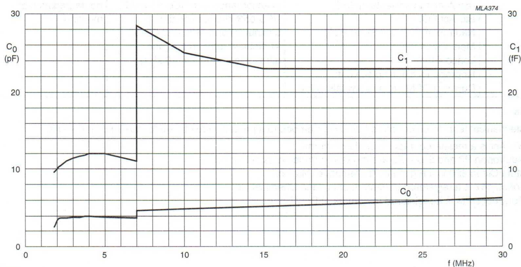
Fig.3 Motional capacitance C_1 and parallel capacitance C_0 as a function of resonance frequency.
