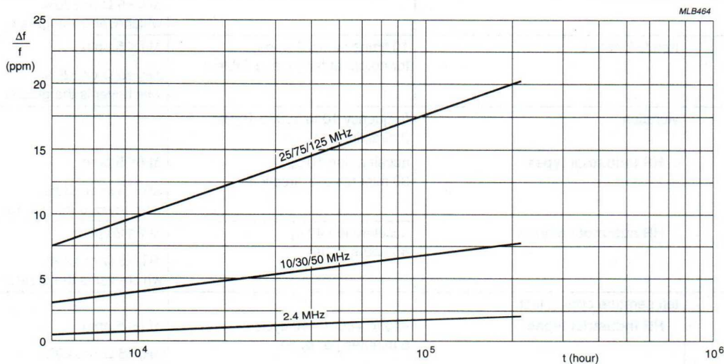
Fig.10 Time/temperature relation at which ageing is approximately equivalent.
