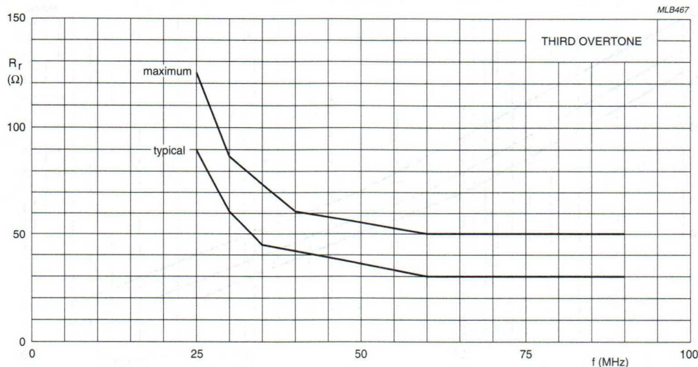
Fig.8 Resonance resistance R_r as a function of resonance frequency, for crystals in 12 mm product length (involving large quartz blanks).
