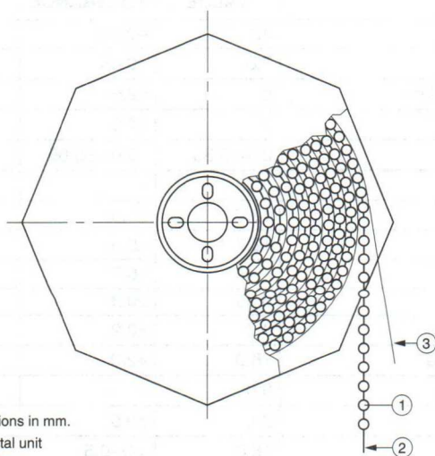
Fig.5 Style 2a, and 3a units on tape in ammpack.
