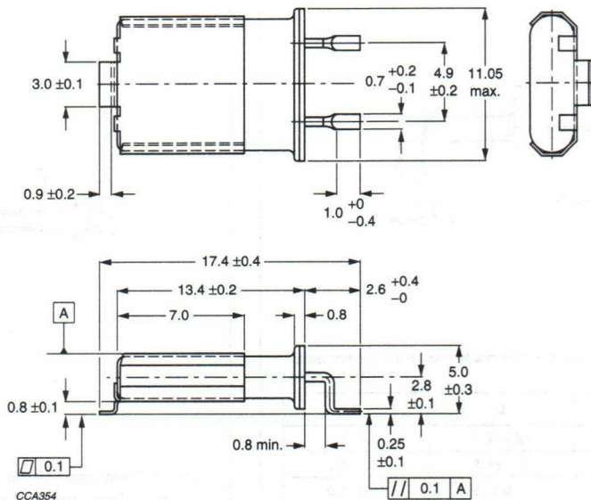
Fig.19 Style 1: HC-49/U17-SMD/Clip I.
