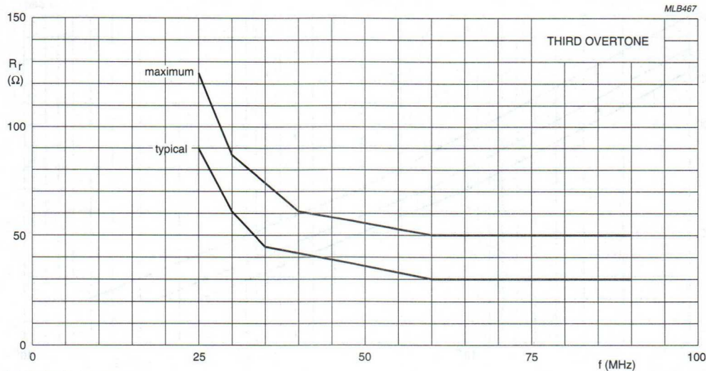
Fig.11 Resonance resistance R_r as a function of resonance frequency, for HC-45/U crystals in 8 mm product height (involving large quartz blanks).
