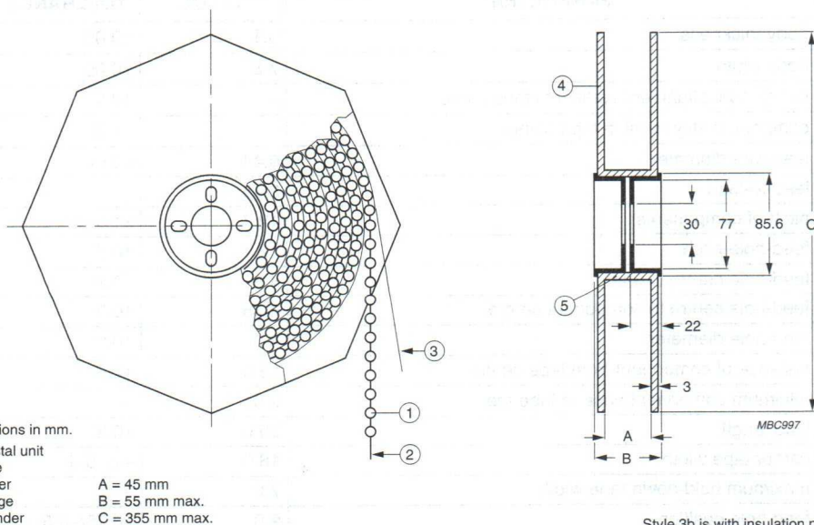
Fig.4 Style 2b and 3b units on tape on reel.
