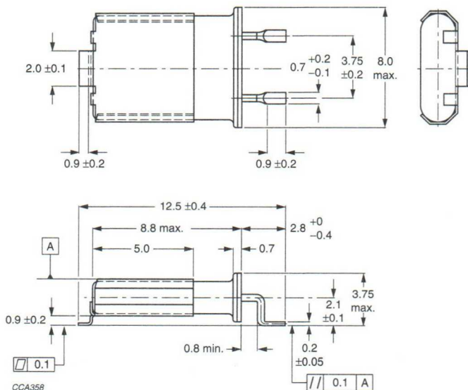
Fig.2 Style 2: HC-45/U12-SMD/Clip I.
