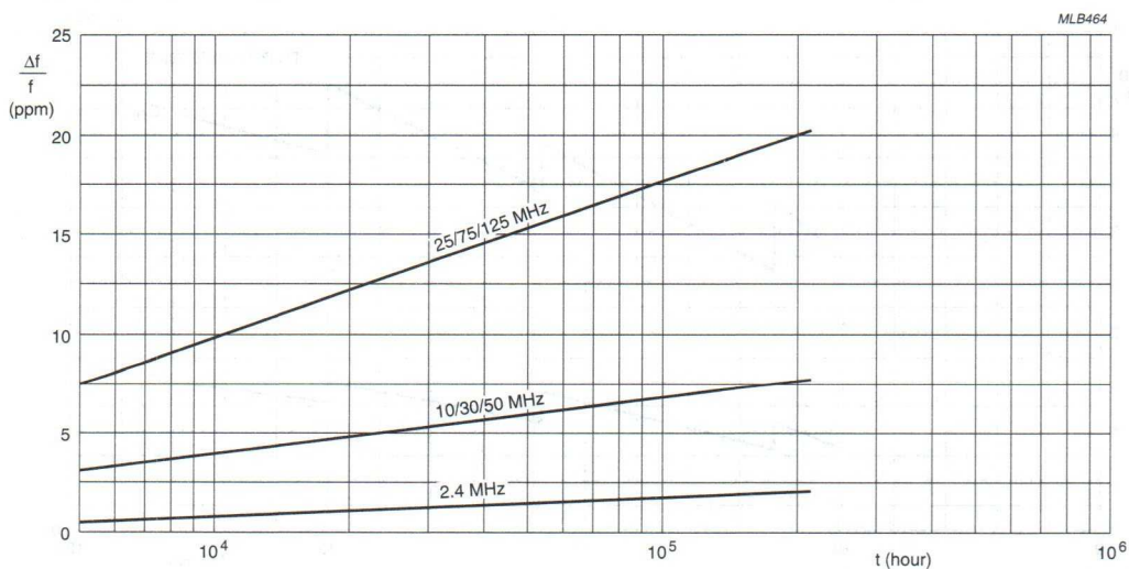
Fig.14 Time/temperature relation at which ageing is approximately equivalent.
