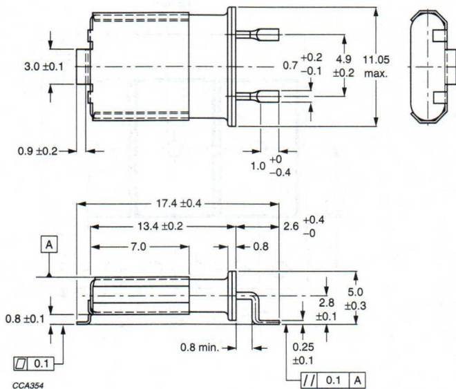
Fig.1 Style 1: HC-49/U17-SMD/Clip I.
