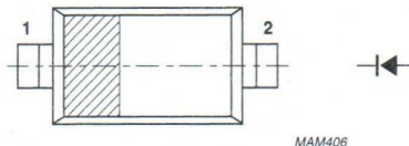
Fig.1 Simplified outline (SOD323) and symbol.
