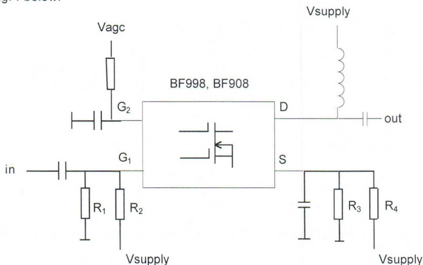
Fig. 1: Principle of the bias circuit for Mosfets without integrated bias.
