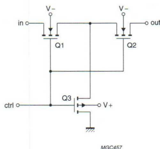
Fig.10 MOS-FET analog switch with low cross talk performance.
