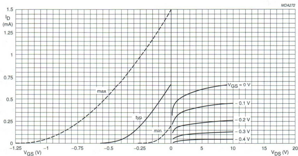
Fig.3 Typical values. V_{DS} = 10 V; T_j = 25 ^{\circ}\text{C} .
