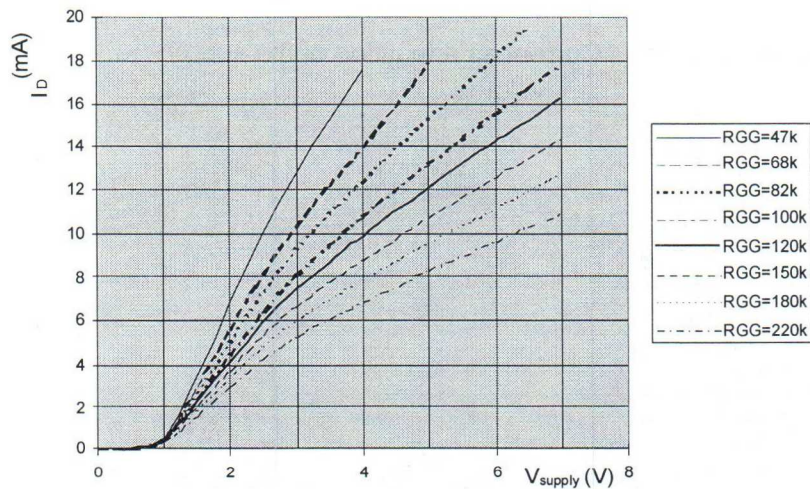
BF1101: Bias current as a function of supply voltage and Gate1 resistor
