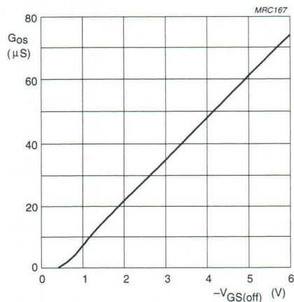
Fig.4 Common source output conductance as a function of gate-source cut-off voltage.
