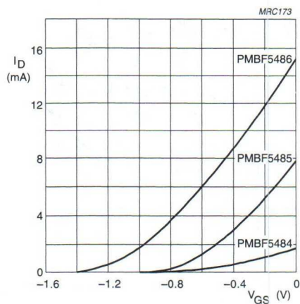
Fig.8 Typical input characteristics.
