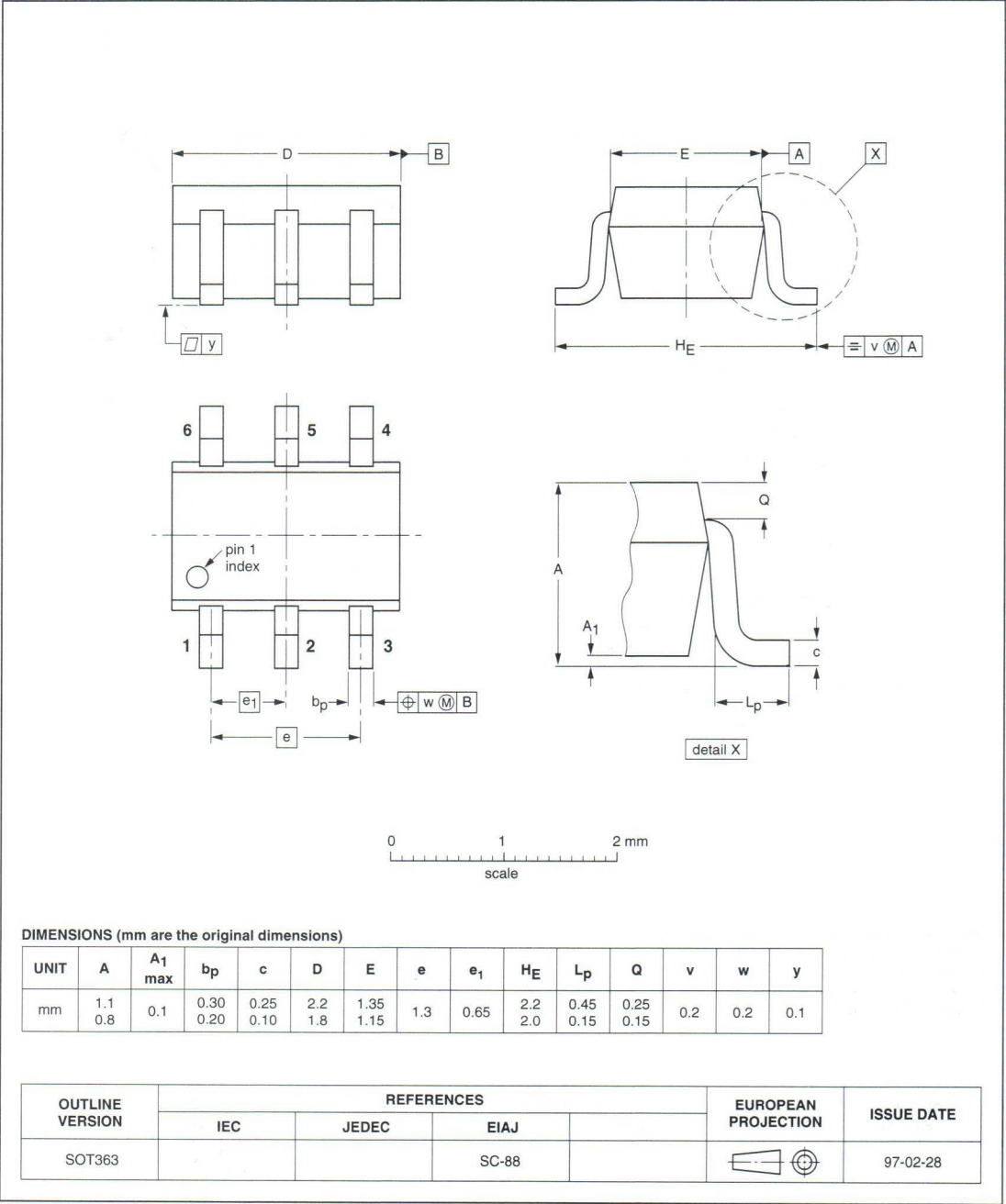
Plastic surface mounted package; 6 leads
