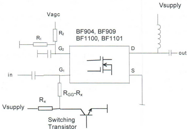
Fig. 10: Switching with open collector n.p.n. transistor at Gate1 of the Mosfets BF904, BF909, BF1100, and BF1101
