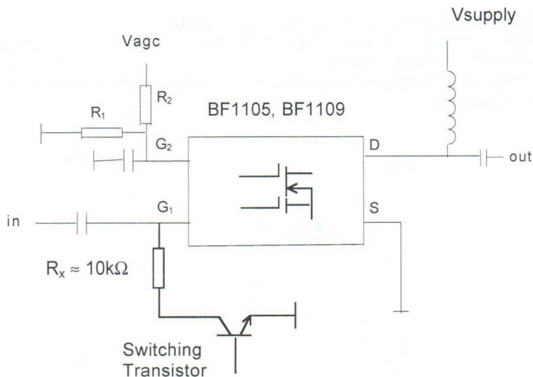
Fig.11: Switching with open collector n.p.n. transistor at Gate1 of the Mosfets BF1105 and BF1109
