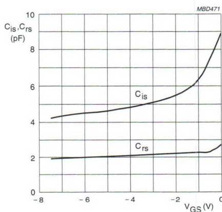
V_{DS} = 8 V. f = 1 MHz.
