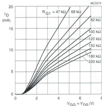
Fig.14 Drain current as a function of gate 1 ( = V_{GG} ) and drain supply voltage; typical values.
