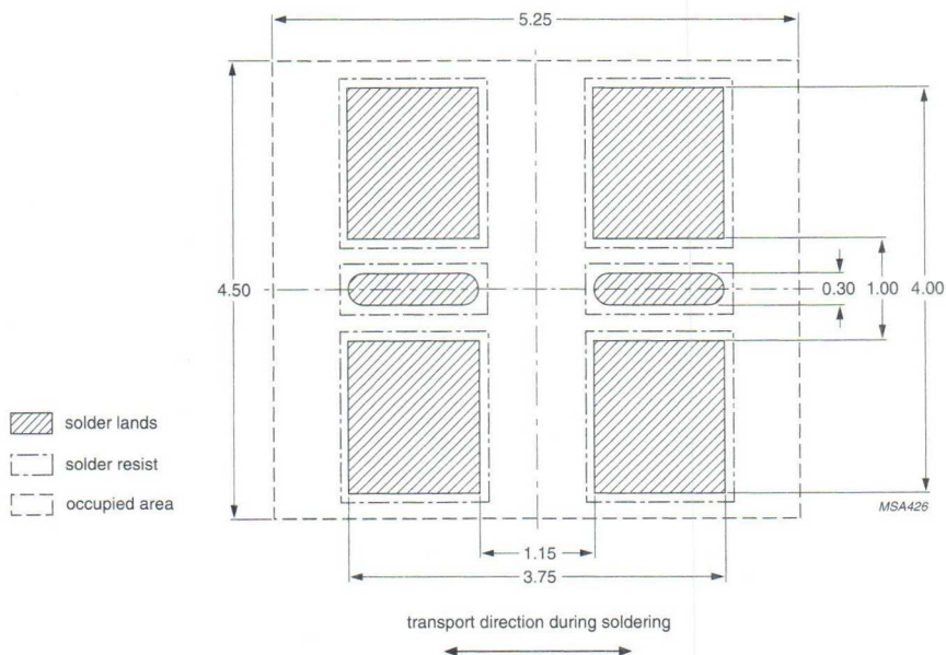
Fig.21 Wave soldering footprint for SOT363; typical dimensions.
