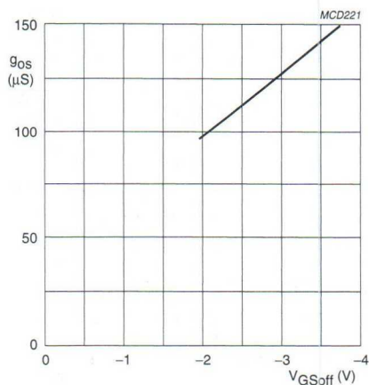
Fig.5 Common-source output conductance as a function of gate-source cut-off voltage; typical values.
