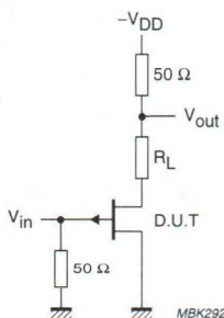
Fig.2 Switching times test circuit.
