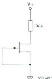
Fig.1 Simple JFET current source.
