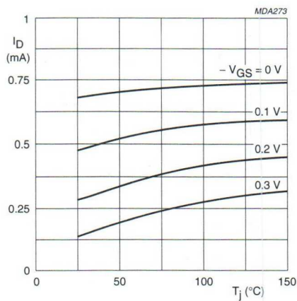
Fig.4 Typical values. V_{DS} = 10\text{ V} .
