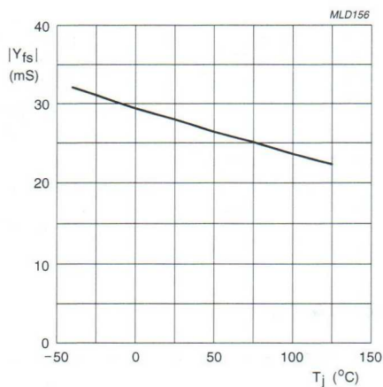
Fig.4 Forward transfer admittance as a function of junction temperature; typical values.
