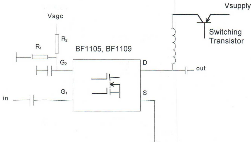
Fig.6: Switching in the Drain of the Mosfets BF1105 and BF1109
