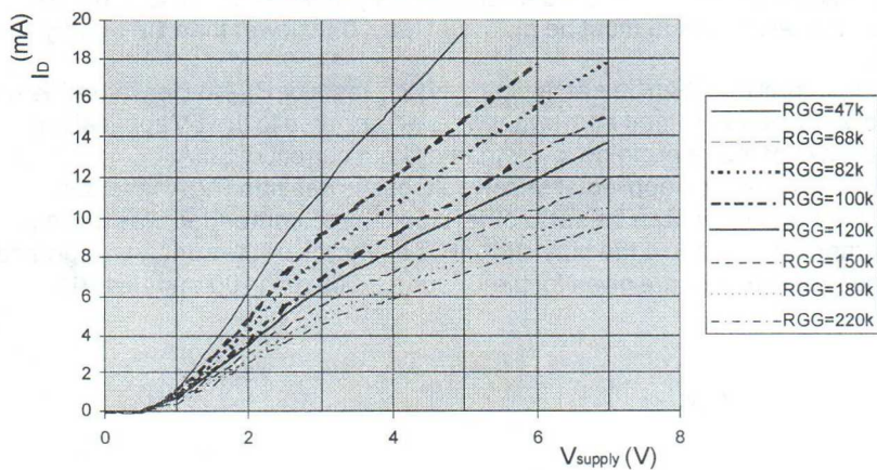
BF904: Bias current as a function of supply voltage and Gate1 resistor
