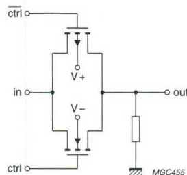
Fig.9 Paralleled complementary MOS-FET switches.
