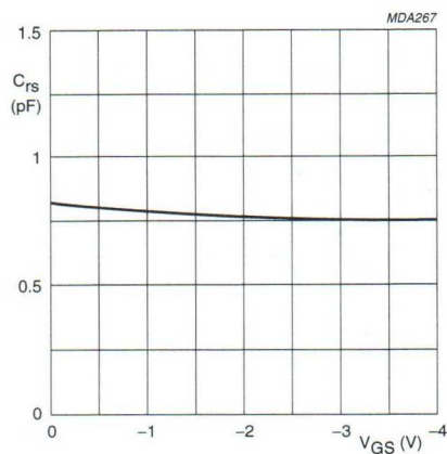
Fig.10 Typical values. V_{DS} = 10 V, T_{amb} = 25 °C.
