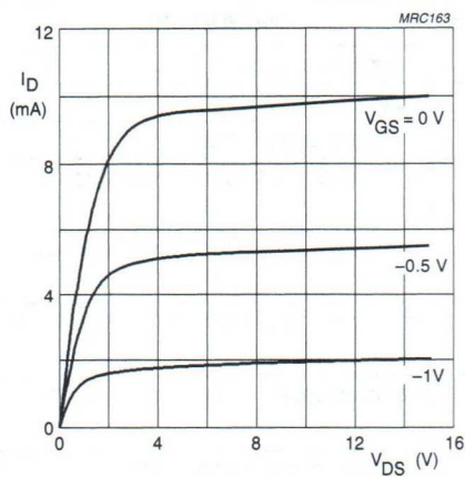
Fig.5 Typical output characteristics.
