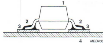
Heat radiates from the package '1' to ambient. Heat conducts via leads '2', solder joints '3' to the substrate '4'.
