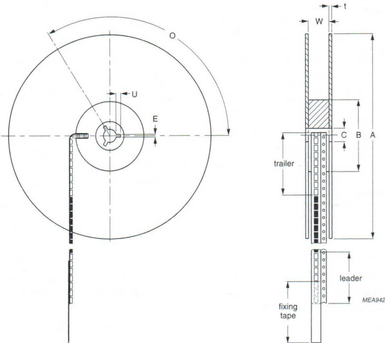
Fig.7 Reel specification.
