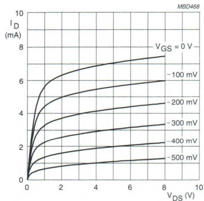
BF861B V_{DS} = 8 \text{ V.}
