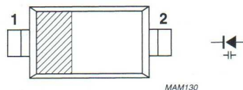
Fig.1 Simplified outline (SOD323) and symbol.
