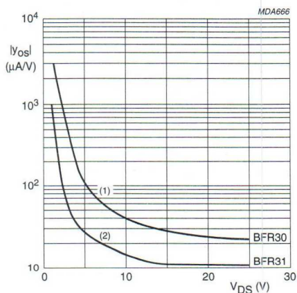
Fig.13 Common source output admittance as a function of drain-source voltage; typical values.
