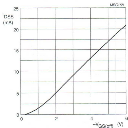
Fig.2 Drain current as a function of gate-source cut-off voltage.
