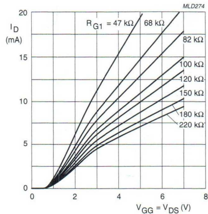
Fig. 16 Drain current as a function of gate 1 ( = V_{GG} ) and drain supply voltage; typical values; see Fig.23.
