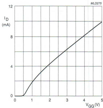
Fig. 15 Drain current as a function of gate 1 supply voltage ( = V_{GG} ); typical values; see Fig.23.
