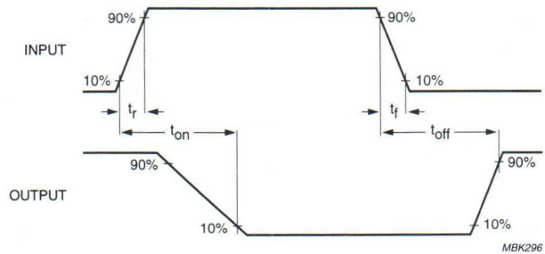
Fig.2 Switching times test circuit and input and output waveforms.
