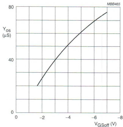
Fig.5 Common-source output admittance as a function of gate-source cut-off voltage; typical values.
