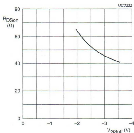
Fig.6 Drain-source on-state resistance as a function of gate-source cut-off voltage; typical values.
