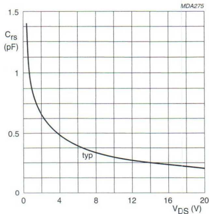
Fig.2 V_{GS} = 0 for BF510 and BF511; I_D = 5\text{ mA} for BF512 and BF513; f = 1\text{ MHz} ; T_{amb} = 25\text{ }^{\circ}\text{C} .
