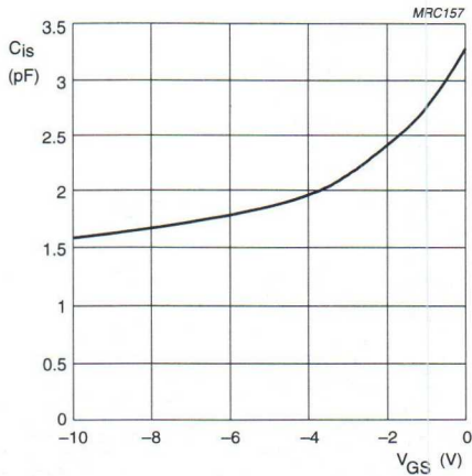
Fig.8 Typical input capacitance.
