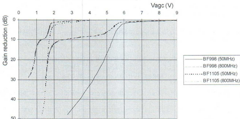
Gain reduction as a function of the AGC voltage (50MHz and 800MHz)
