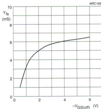
Fig.3 Common source transfer admittance as a function of gate-source cut-off voltage.
