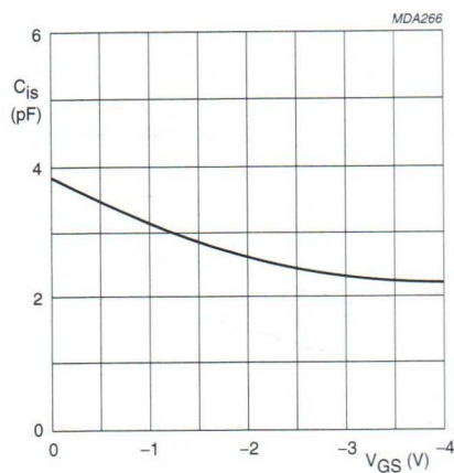
Fig.9 Typical values. V_{DS} = 10 V; T_{amb} = 25 °C.
