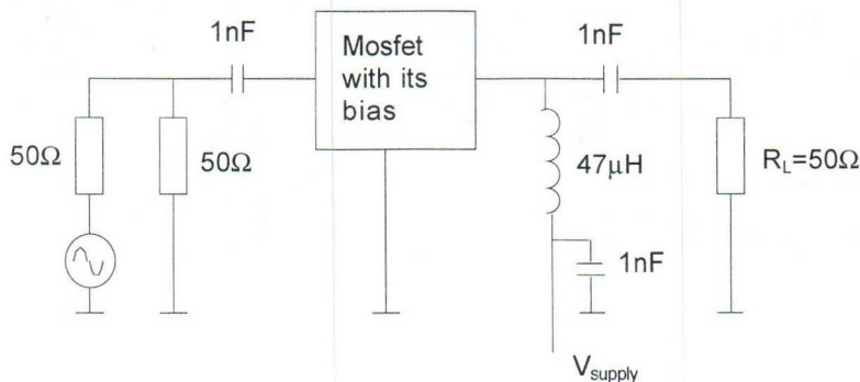
Fig. 12: AGC and cross-modulation test circuit
