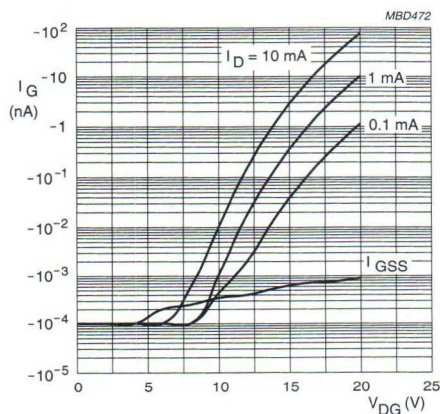
V_{DS} = 8 V.
