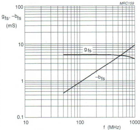
Fig.12 Common source transfer conductance; typical values.
