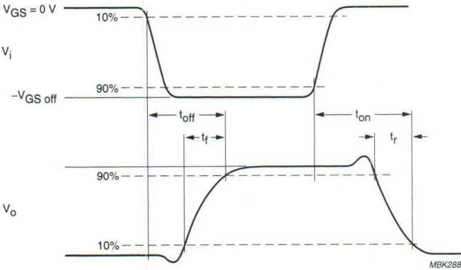
Fig.2 Switching times waveforms.
