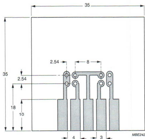
Fig.6 Standard mounting conditions for SOT54.
