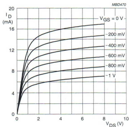
BF861C V_{DS} = 8 V.
