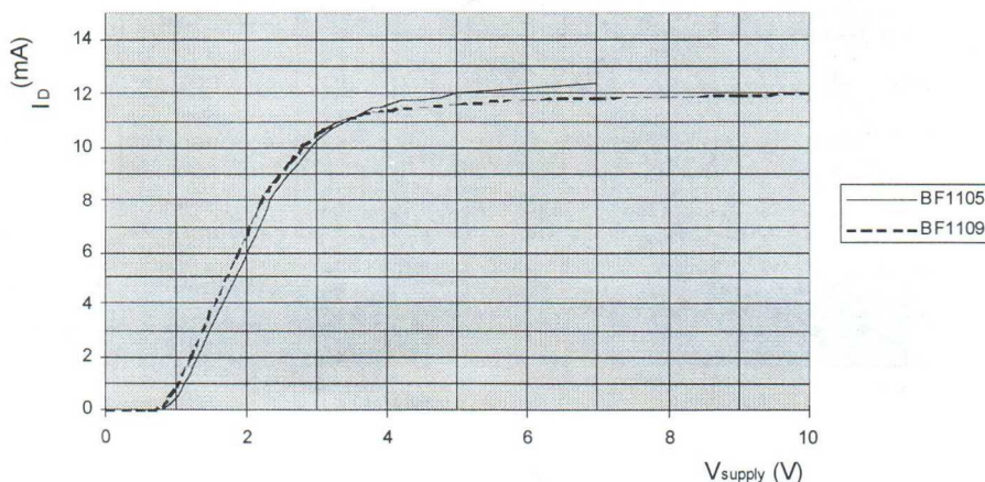
Self Biasing drain Current as a function of the supply voltage
