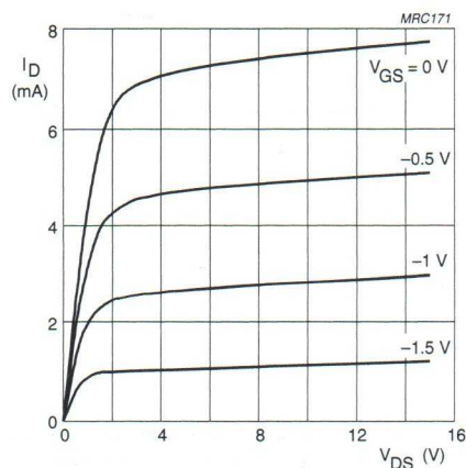
Fig.6 Typical output characteristics.
