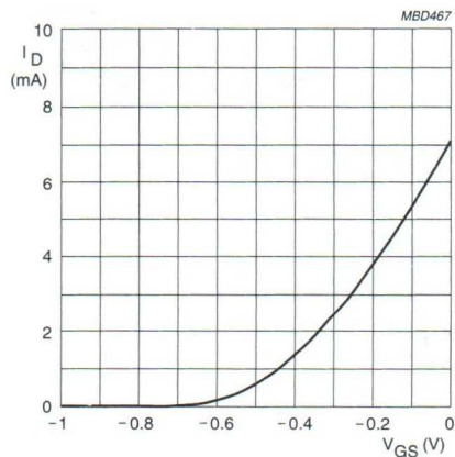
BF861B V_{DS} = 8 \text{ V.}
