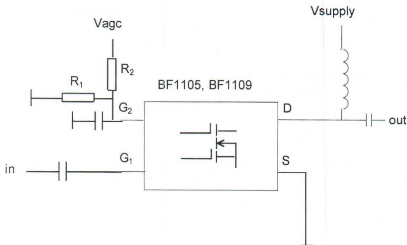
Fig. 3: Principle of the bias circuit for Mosfets with fully integrated bias.
