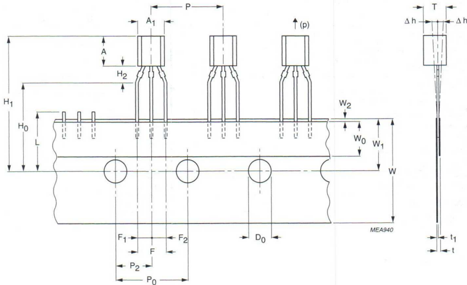
Fig.1 TO-92 transistors on tape.
