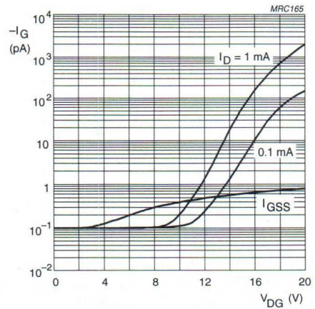
Fig.9 Gate current as a function of drain-gate voltage, typical values.
