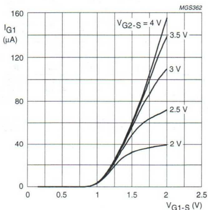
Fig.5 Gate 1 current as a function of gate 1 voltage; typical values.
