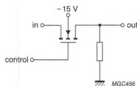
Fig.8 MOS-FET analog switch.
