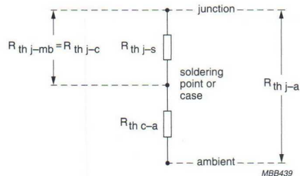
Fig.2 Representation of thermal resistance paths of a device mounted on a substrate or printed board.
