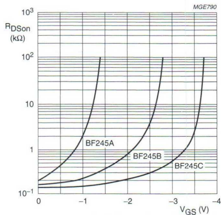
Fig.20 Drain-source on-state resistance as a function of gate-source voltage; typical values.
