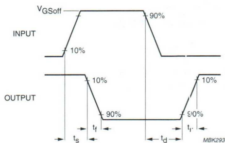
Fig.3 Input and output waveforms; t_d + t_r = t_{on} ; t_s + t_f = t_{off} .
