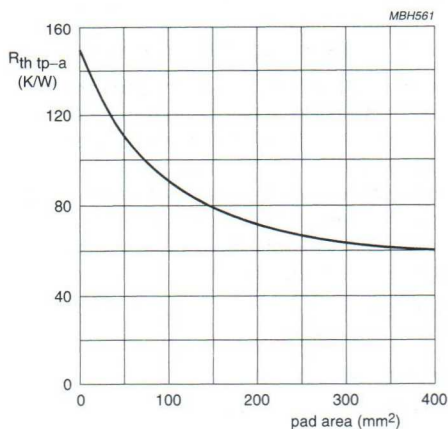
Fig.3 Thermal resistance ( R_{th(tp-a)} ) as a function of FR4 printed-circuit board pad area.
