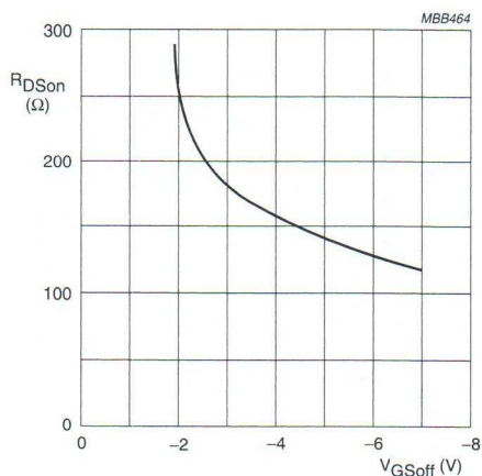
Fig.6 Drain-source on-resistance as a function of gate-source cut-off voltage; typical values.
