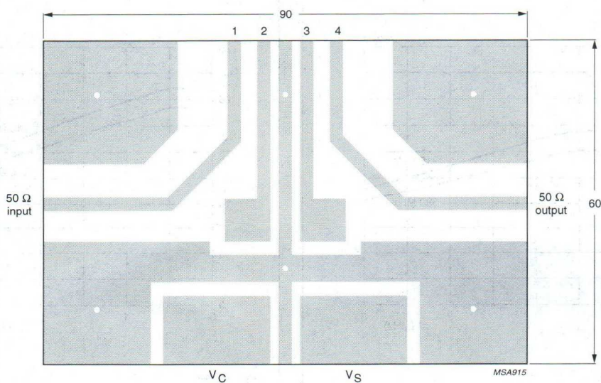
Fig.15 Printed-circuit board layout.
