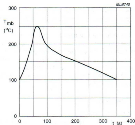
Fig.17 Maximum allowable temperature profile.
