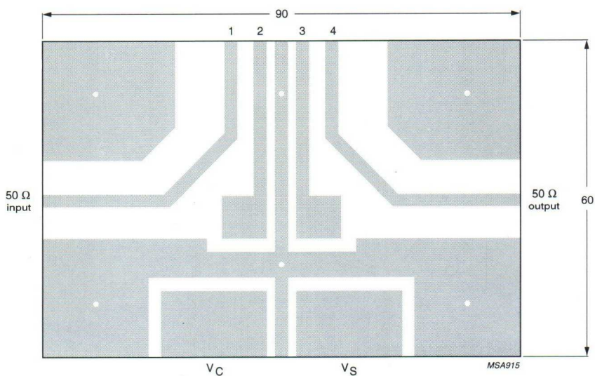
Fig.9 Printed-circuit board layout.
