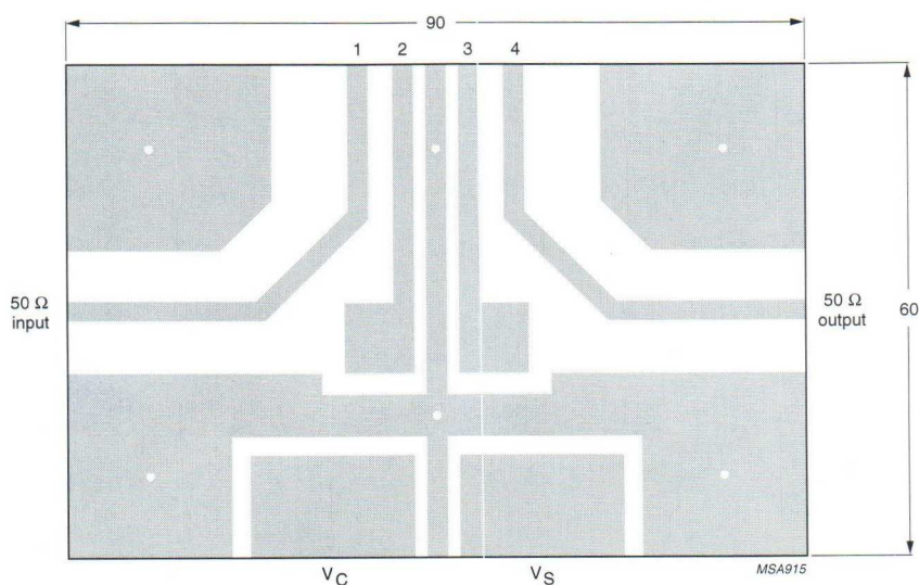
Fig.11 Printed-circuit board layout.
