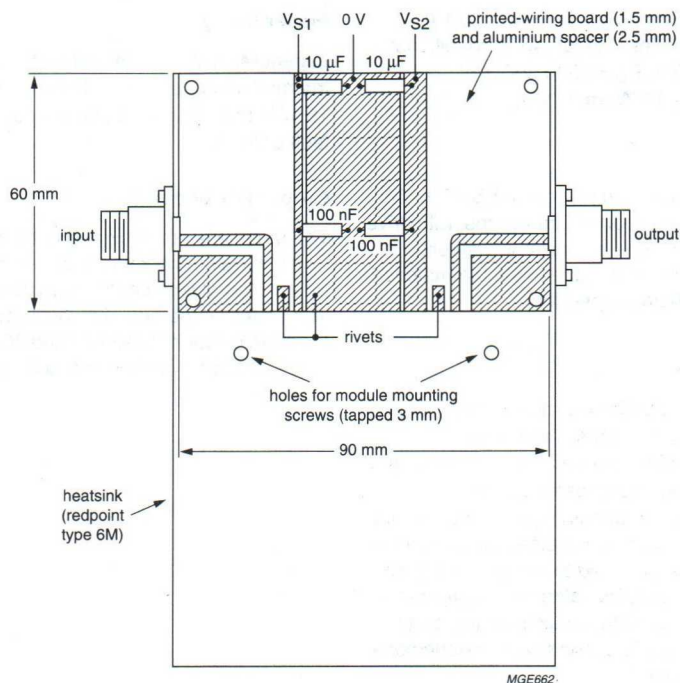
Fig.4 Test jig for VHF modules.
