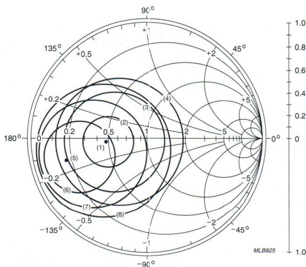
Fig.18 Common emitter noise figure circles; typical values.
