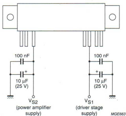
Fig.5 Recommended decoupling arrangement.
