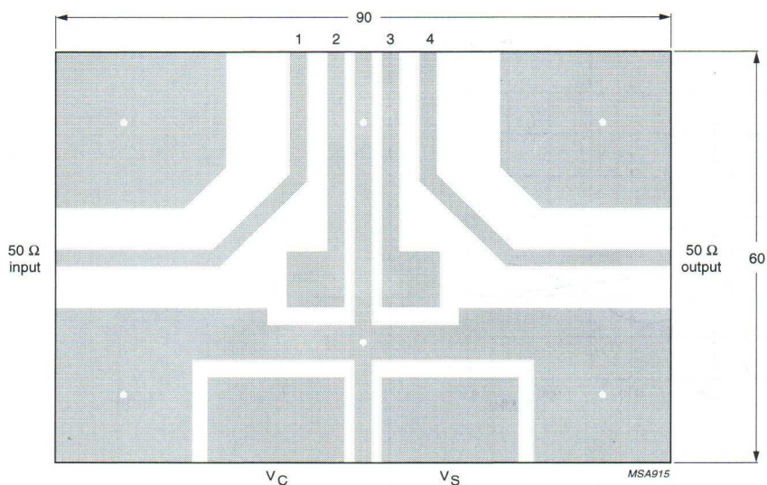
Fig.24 Printed-circuit board layout.
