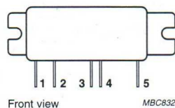
Fig.1 Simplified outline.
