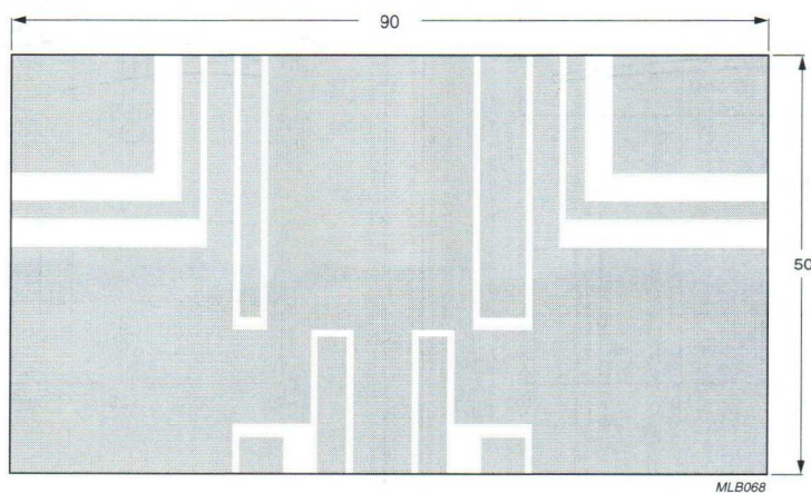
Fig.14 Printed-circuit board layout.
