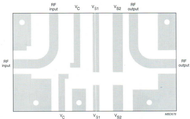
Fig.11 Printed-circuit board layout.
