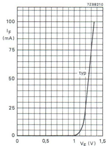
Fig. 11 Forward current as a function of forward voltage; T_{amb} = 25 \text{ }^{\circ}\text{C} .
