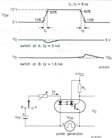
Fig.4 Transient immunity test circuit and waveforms.
