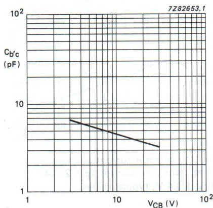
Fig.20 Output capacitance as a function of base-collector voltage; f = 1 MHz; T_{amb} = 25^\circ\text{C} .
