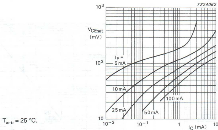
Fig.15 Collector-emitter saturation voltage as a function of collector current, typical values.
