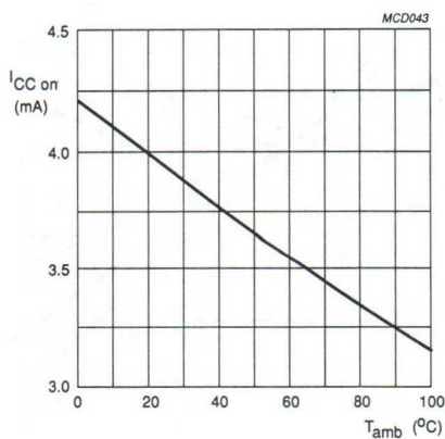
Fig.22 Supply 'on' current ( I_{CC\ on} ) as a function of temperature.
