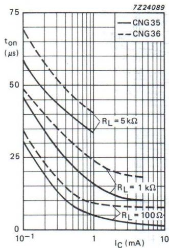
Fig.22 Turn-on time as a function of collector current; I_B = 0 ; V_{CC} = 5 V; T_{amb} = 25 °C; typical values.
