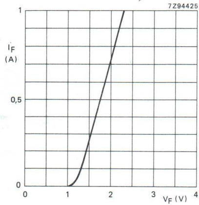
Fig. 6 Forward current as a function of forward voltage; T_{amb} = 25\text{ }^{\circ}\text{C} ; t_{on} = 20\text{ }\mu\text{s} ; \delta = 0.01 ; typical values.
