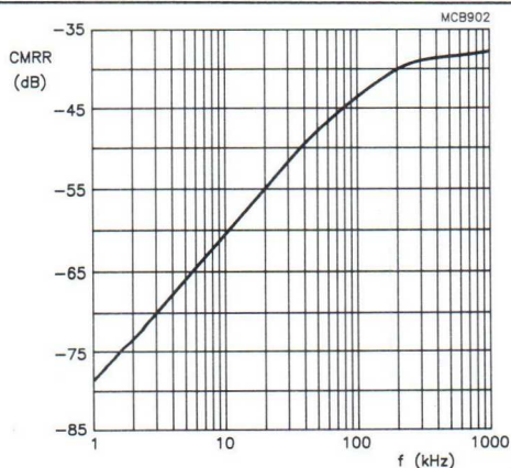
Fig.16 Common mode rejection ratio as a function of frequency, CNW85.
