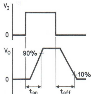
Fig. 23 Switching circuit and waveforms.
