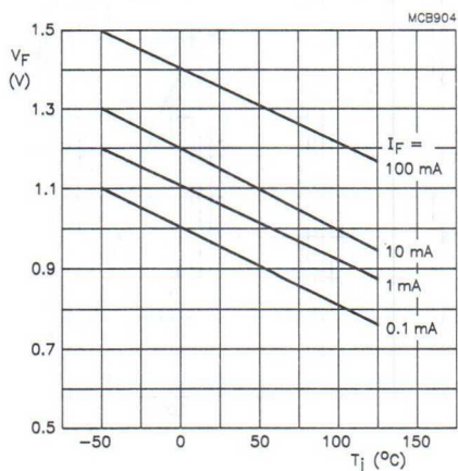
Fig.6 Forward voltage as a function of junction temperature, typical values.
