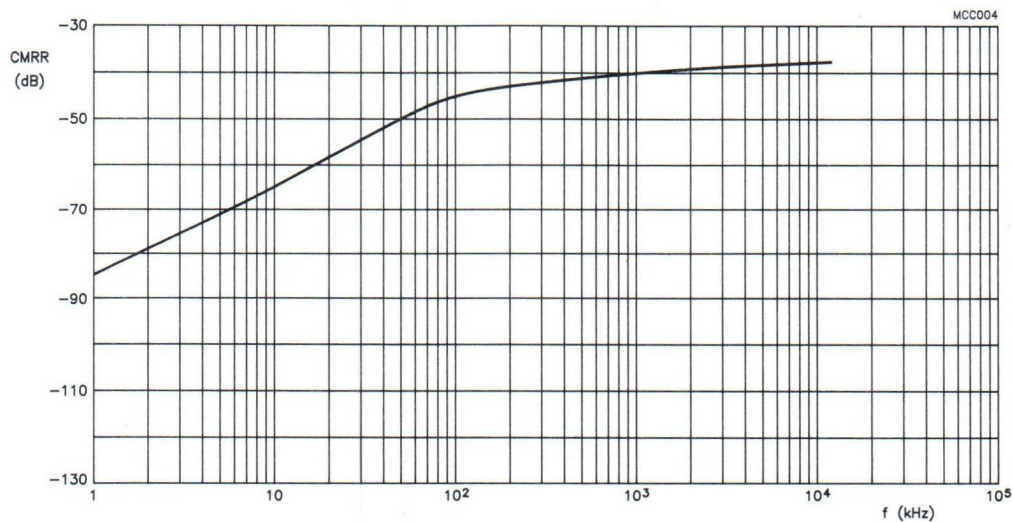
Fig.20 Common mode rejection ratio as a function of frequency.
