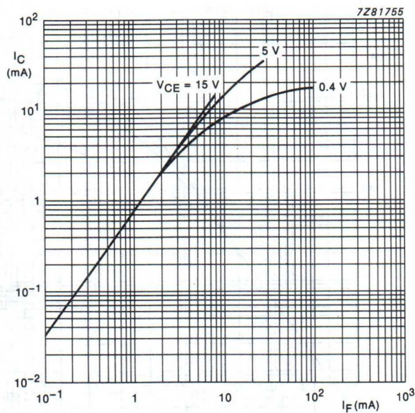
Fig.15 Collector current as a function of forward current, typical values.
