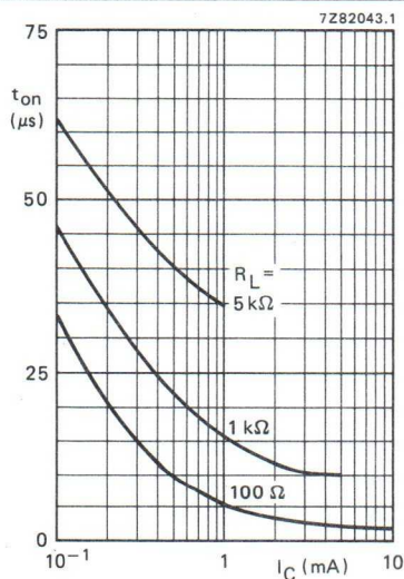
Fig.25 Turn-on time as a function of collector current.
