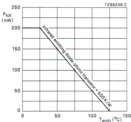
Fig. 10 Power derating curve for diode and transistor as a function of temperature.
