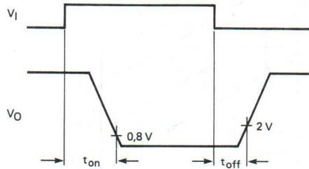
Fig. 2 Measuring circuit and waveforms.
