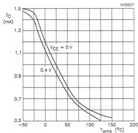
Fig.7 Collector current as a function of ambient temperature.
