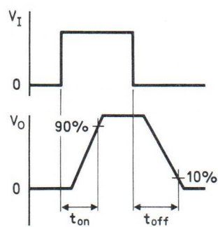
Fig. 4 Waveforms.
