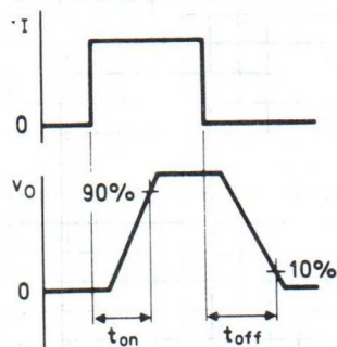
Fig. 3 Waveforms.
