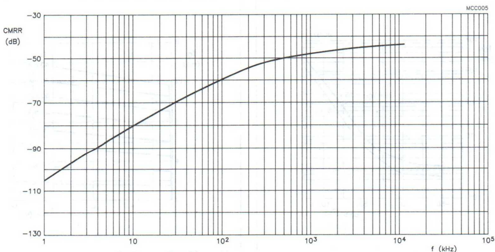
Fig.22 Common mode rejection ratio as a function of frequency.
