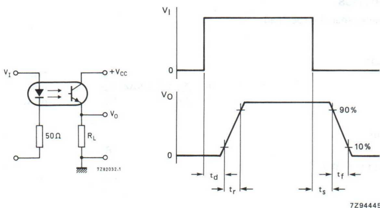
Fig.2 Measuring circuit and waveforms.
