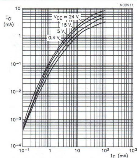
Fig.9 Collector current as a function of forward current.
