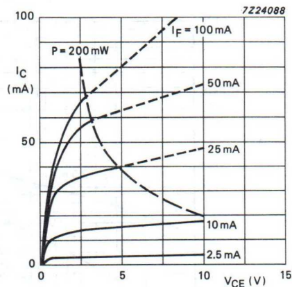
Fig.16 Collector current as a function of collector-emitter voltage; T_{\text{amb}} = 25^\circ\text{C} ; typical values; CNG36.
