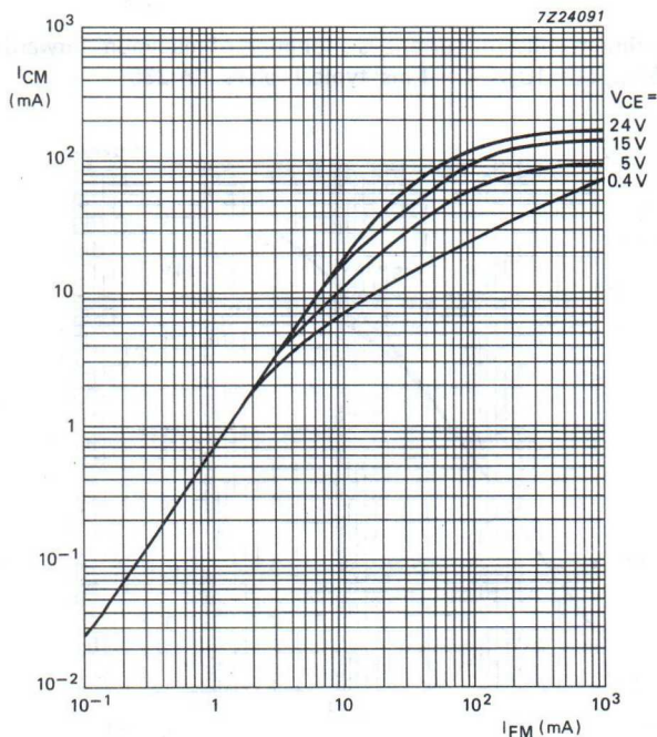
Fig.24 Maximum collector current as a function of maximum forward current; T_{amb} = 25 °C; t_p = 10 \mu s ; T = 1 ms; typical values; CNG35.
