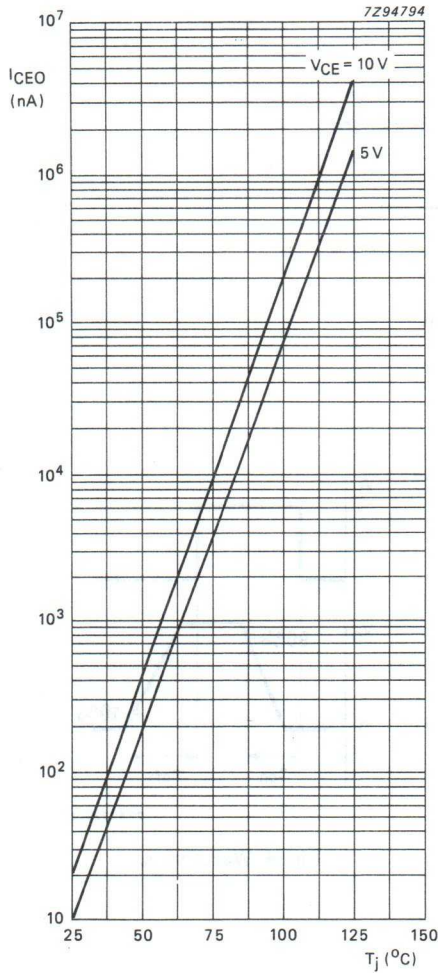
Fig. 5 Collector-emitter voltage as a function of junction temperature; typical values.
