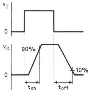
Fig. 25 Switching circuit and waveforms.
