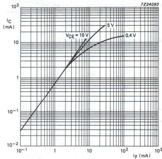
Fig.26 Collector current as a function of forward current; T_{amb} = 25^{\circ}\text{C} ; typical values; CNG35 .
