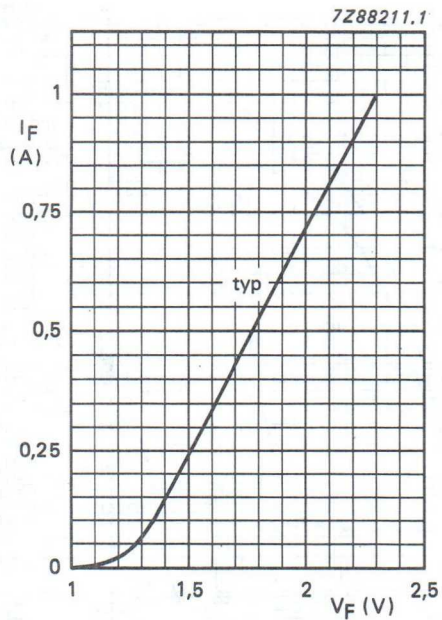
Fig.8 Forward current as a function of forward voltage.
