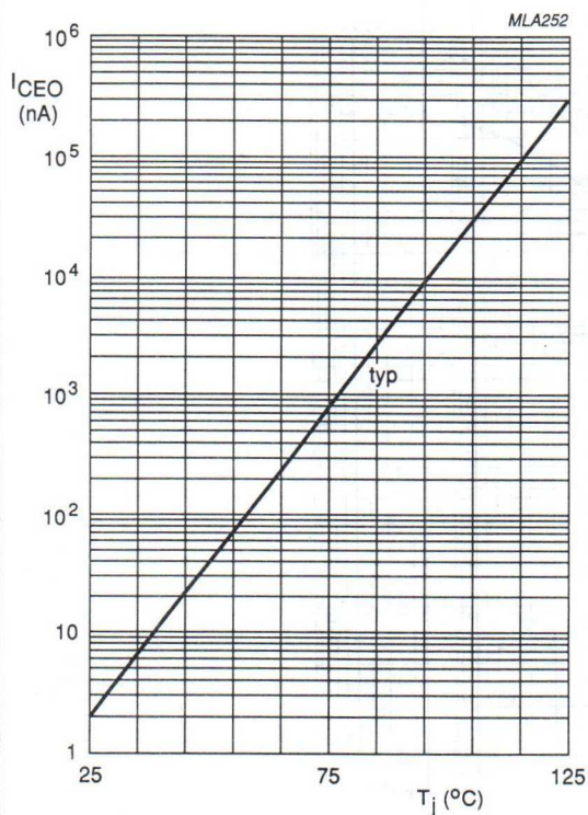
Fig.11 Collector-emitter dark current as a function of junction temperature.
