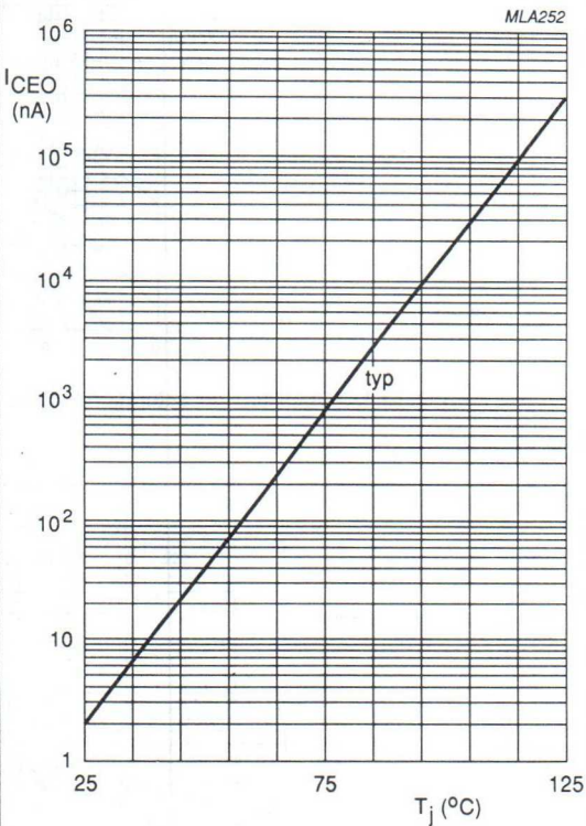
Fig.14 Collector-emitter dark current as a function of junction temperature.
