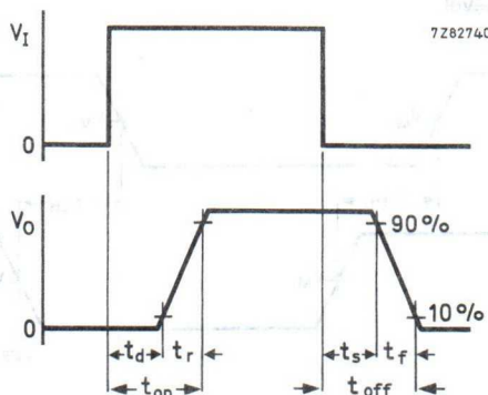
Fig. 4 Waveforms.
