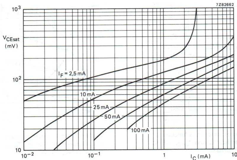
Fig.19 Collector-emitter saturation voltage as a function of collector current; I_B = 0 ; T_{amb} = 25^\circ\text{C} ; typical values.
