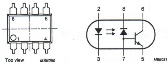
Fig.1 Simplified outline and symbol.
