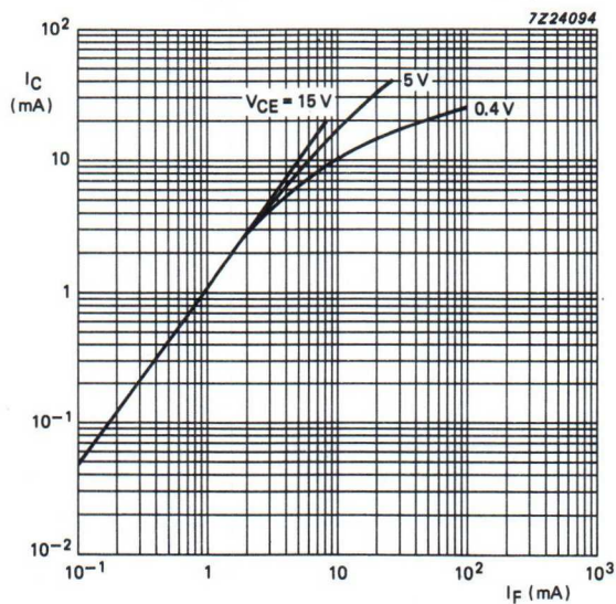
Fig.27 Collector current as a function of forward current; T_{amb} = 25^\circ\text{C} ; typical values; CNG36 .
