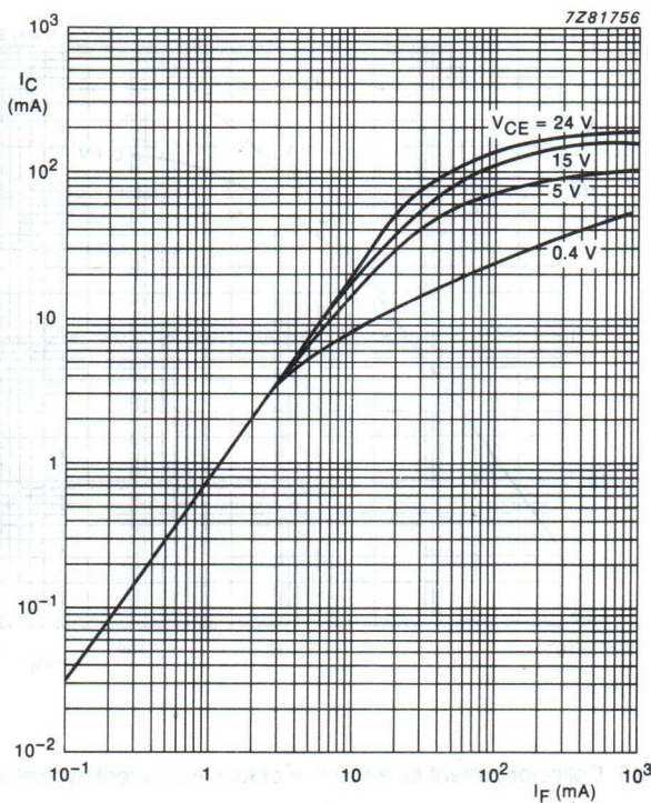
Fig.16 Maximum collector current as a function of maximum forward current, typical values.
