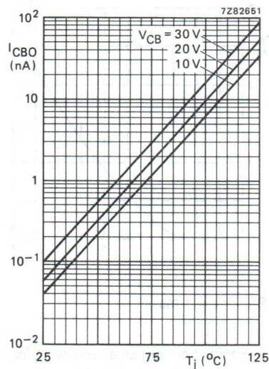
Fig.13 Collector-base cut-off current as a function of junction temperature, CNG83.
