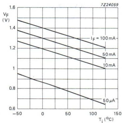
Fig.9 Forward voltage as a function of junction temperature, typical values.
