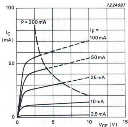
Fig.15 Collector current as a function of collector-emitter voltage; T_{\text{amb}} = 25^\circ\text{C} ; typical values; CNG35.
