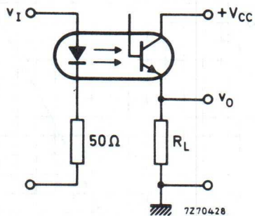
Fig. 2 Switching circuit.
