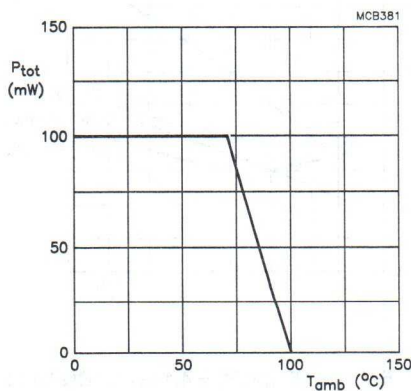
Fig.10 Total power dissipation as a function of ambient temperature.
