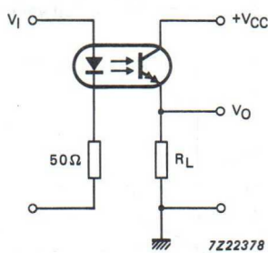
Fig. 3 Switching circuit.
