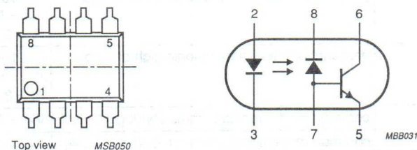
Fig.1 Simplified outline and symbol.
