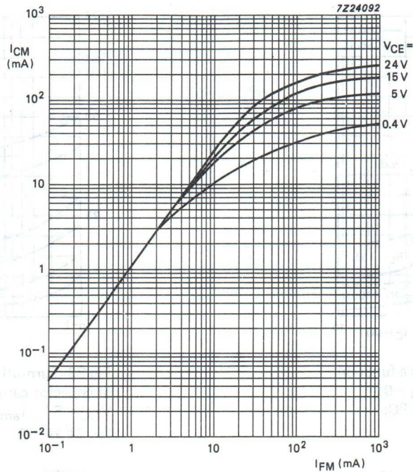
Fig.25 Maximum collector current as a function of maximum forward current; T_{amb} = 25^{\circ}\text{C} ; t_p = 10 \mu\text{s} ; T = 1 \text{ ms} ; typical values; CNG36 .
