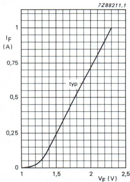
Fig.8 Forward current as a function of forward voltage, typical values.
