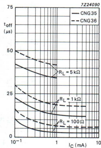
Fig.23 Turn-off time as a function of collector current; I_B = 0 ; V_{CC} = 5 V; T_{amb} = 25 °C; typical values.
