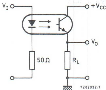
Fig. 23 Switching circuit and waveforms.
