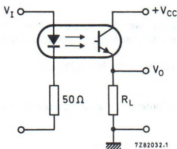
Fig. 1 Switching circuit.
