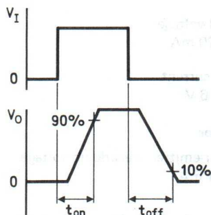
Fig. 3 Waveforms.
