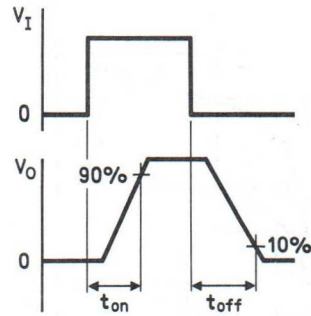
Fig. 3 Waveforms.
