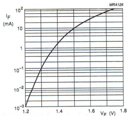
Fig.11 Forward current as a function of forward voltage; typical values.
