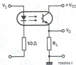
Fig. 2 Measuring circuit and waveforms.
