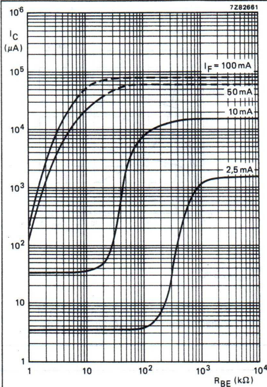
Fig. 18 Collector current as a function of base-emitter resistance, CNG83; typical values.
