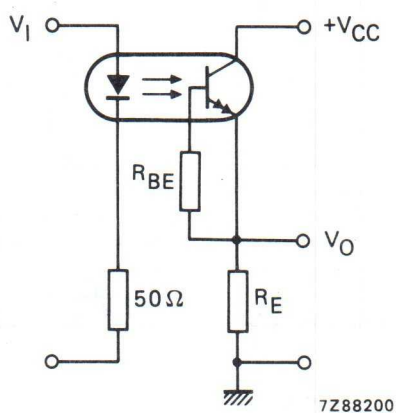
Fig. 3 Switching circuit.
