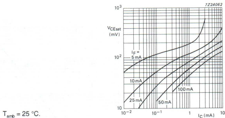
Fig.15 Collector-emitter saturation voltage as a function of collector current, typical values.
