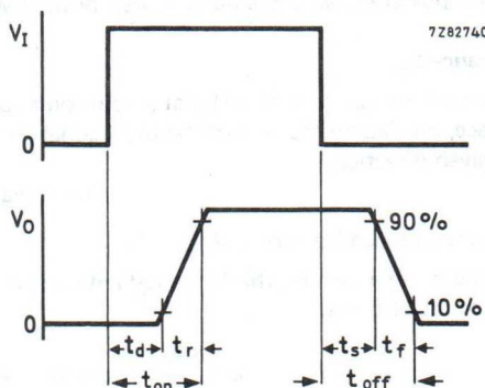
Fig. 2 Waveforms.
