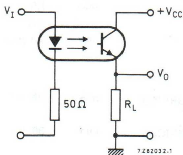
Fig. 2 Switching circuit.
