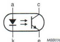
Fig.2 Symbol, CNX82A.
