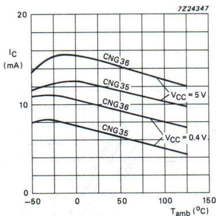
Fig.17 Collector current as a function of ambient temperature; I_F = 10 \text{ mA} ; typical values.
