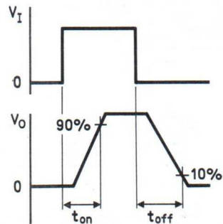
Fig. 4 Waveforms.
