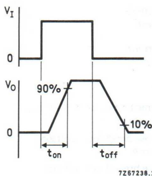
Fig. 3 Waveforms.
