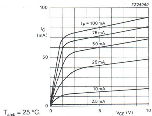
Fig.10 Collector current as a function of collector-emitter voltage, typical values.
