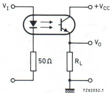
Fig. 2 Switching circuit.
