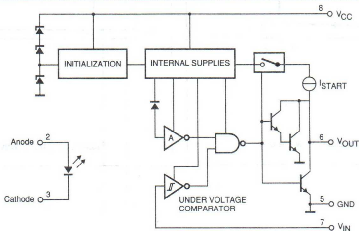
Fig.2 Functional diagram.
