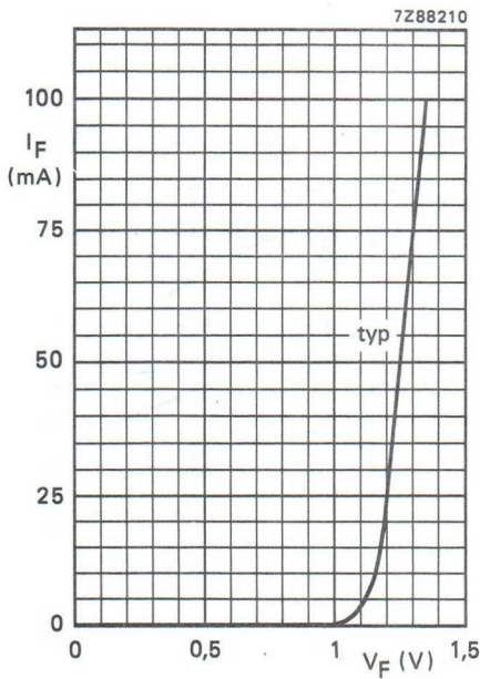
Fig.7 Forward current as a function of forward voltage, typical values.
