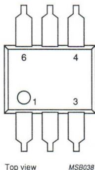
Fig.1 Simplified outline.
