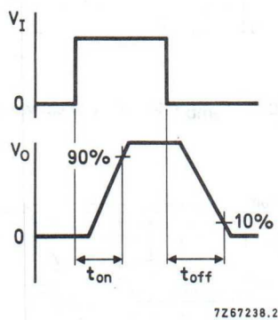
Fig. 4 Waveforms.
