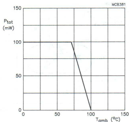
Fig.6 Total power dissipation as a function of ambient temperature.
