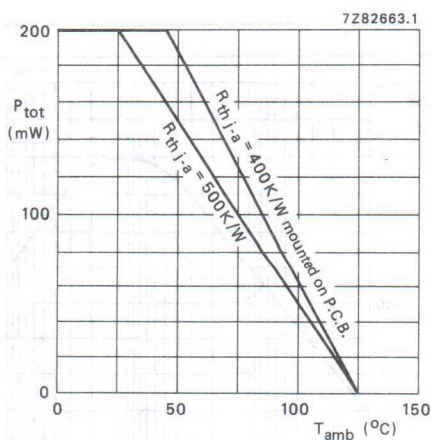
Fig.20 Total power dissipation as a function of ambient temperature.
