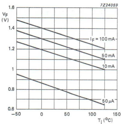
Fig.9 Forward voltage as a function of junction temperature.
