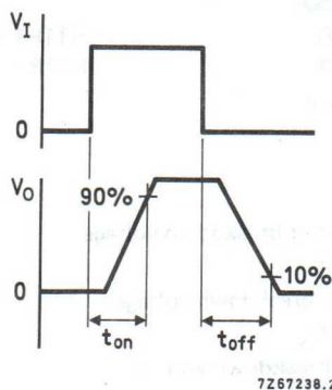
Fig. 3 Waveforms.
