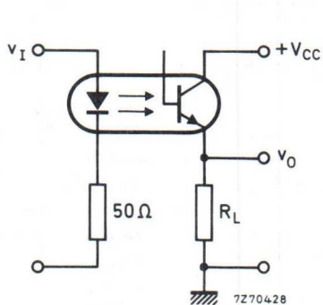
Fig. 2 Switching circuit.
