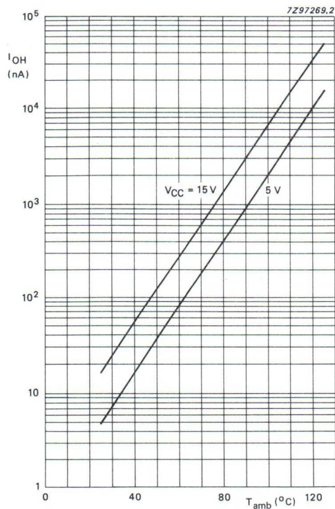
Fig.14 Logic high output current as a function of ambient temperature, typical values.
