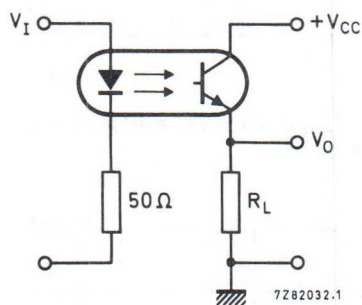
Fig. 3 Switching circuit.
