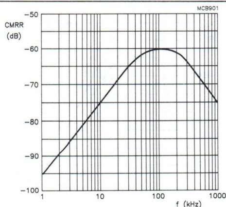
Fig.17 Common mode rejection ratio as a function of frequency, CNW84.
