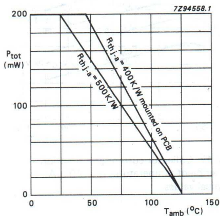
Fig.21 Total power dissipation as a function of ambient temperature.
