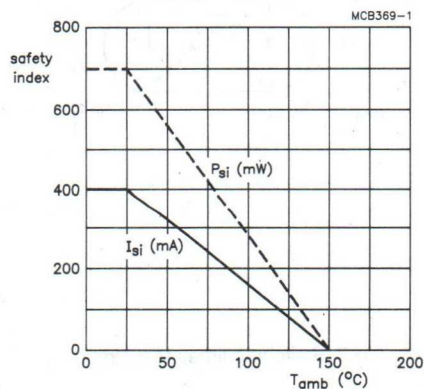
Fig.6 Dependence of maximum safety ratings with ambient temperature.
