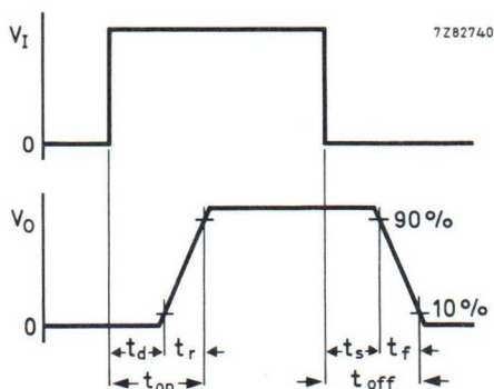
Fig. 13 Switching circuit and waveforms.
