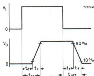
Fig. 2 Measuring circuit and waveforms.
