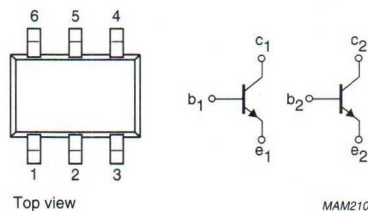
Fig.1 Simplified outline and symbol.
