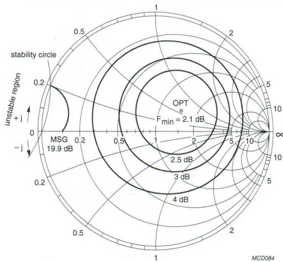
Fig.13 Common emitter noise figure circles; typical values.
