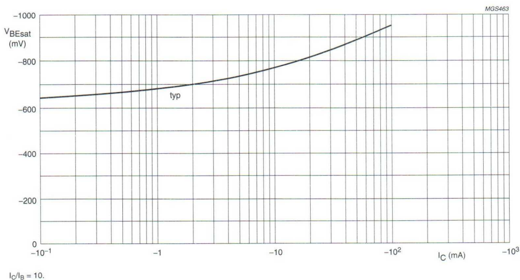
Fig.5 Base-emitter saturation voltage as a function of collector current; typical values.
