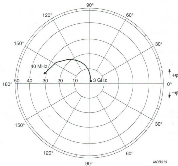
Fig.17 Common emitter forward transmission coefficient ( S_{21} ).
