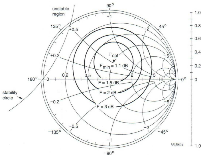
Fig.16 Common emitter noise figure circles; typical values.
