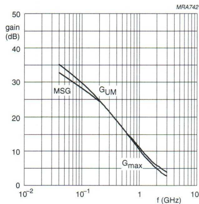
Fig.11 Gain as a function of frequency.
