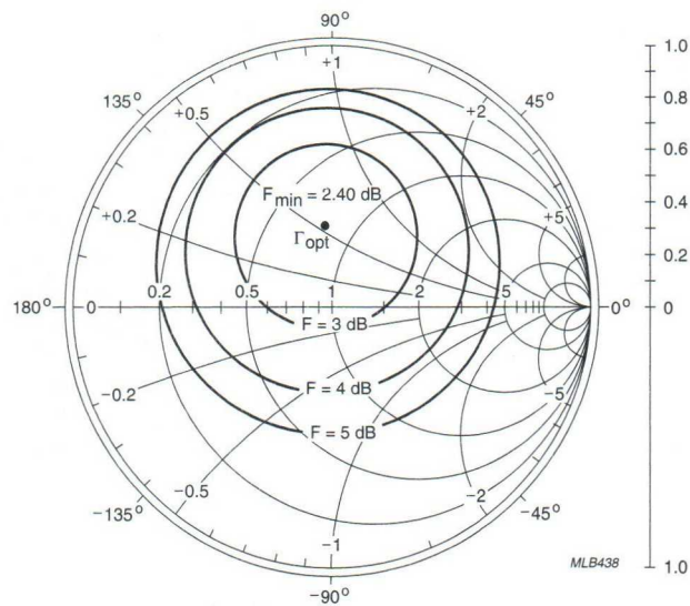
Fig.16 Common emitter noise figure circles, typical values.
