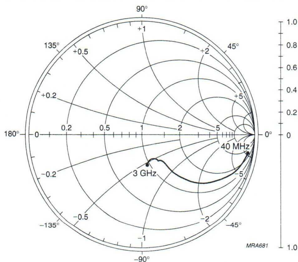
Fig.20 Common emitter output reflection coefficient ( S_{22} ).
