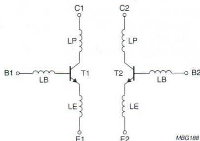
Fig.14 Package equivalent circuit SOT363A (inductance only).
