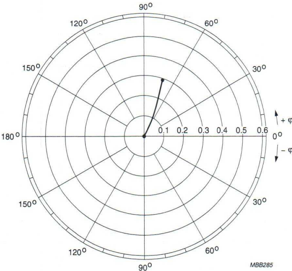
Fig.24 Common emitter reverse transmission coefficient ( S_{12} ).
