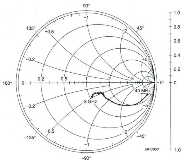
Fig.15 Common emitter output reflection coefficient ( S_{22} ).
