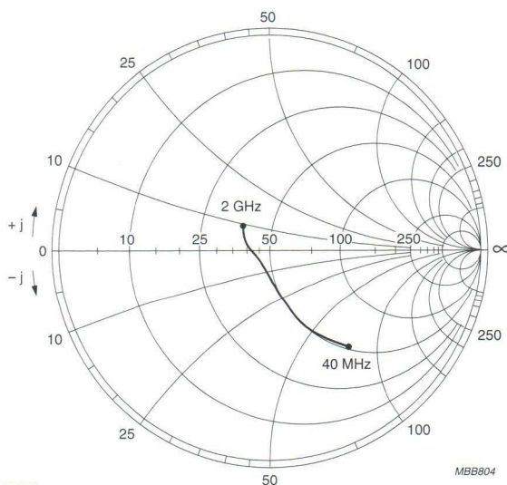
Fig.25 Common emitter output reflection coefficient ( S_{22} ).
