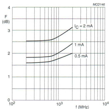
Fig.11 Minimum noise figure as a function of frequency.
