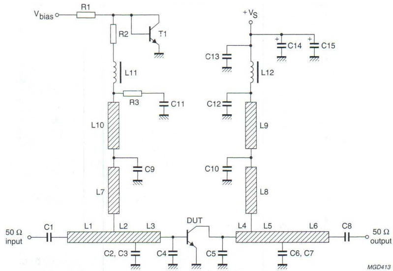
Fig.5 Common-emitter test circuit for class-AB operation at 1.9 GHz.
