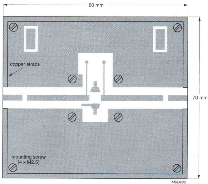
Fig.3 Intermodulation test circuit printed circuit board.
