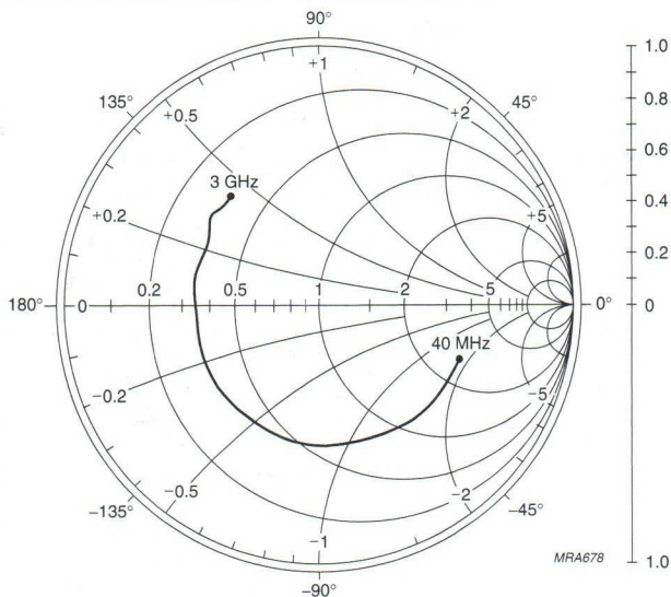
Fig.17 Common emitter input reflection coefficient ( S_{11} ).
