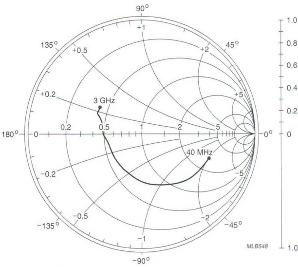
Fig.10 Common emitter input reflection coefficient ( s_{11} ), typical values.
