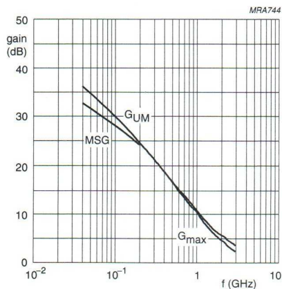
Fig.10 Gain as a function of frequency.
