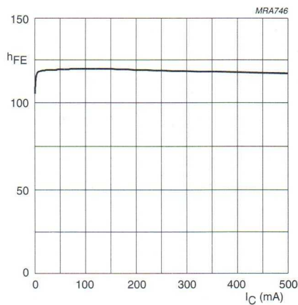
Fig.5 DC current gain as a function of collector current.
