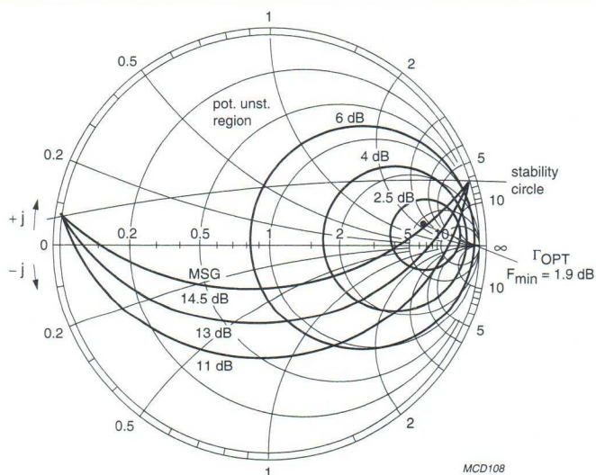
Fig.12 Noise circle figure.
