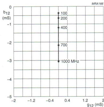
Fig.7 Common base reverse transfer admittance ( Y_{12} ).
