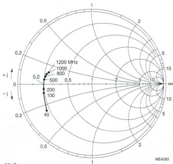
Fig.10 Common emitter output reflection coefficient ( S_{22} ).
