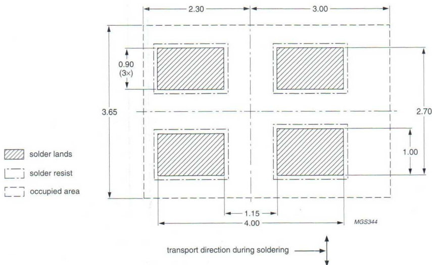
Fig.18 Wave soldering footprint for SOT343; typical dimensions.
