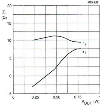
Fig.16 Input impedance as a function of output power.
