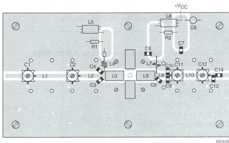
Fig.5 Printed circuit board and component layout for 900 MHz class-B test circuit.
