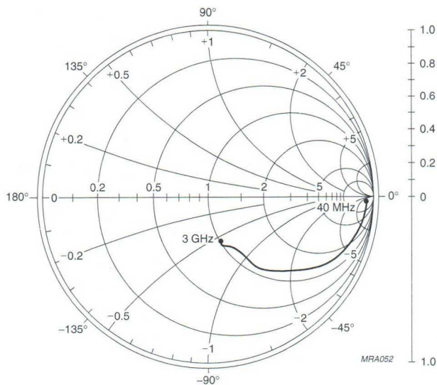
Fig.15 Common emitter input reflection coefficient ( S_{11} ).
