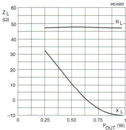
Fig.14 Load impedance as a function of output power.
