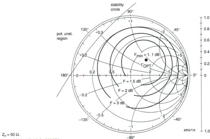
Fig.12 Noise circle figure.
