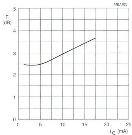
Fig.6 Minimum noise figure as a function of collector current.
