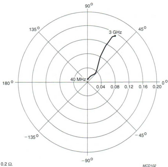
Fig.17 Common emitter reverse transmission coefficient ( S_{12} ).
