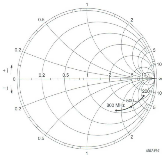
Fig.6 Common emitter input reflection coefficient ( S_{11} ).
