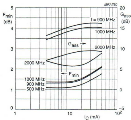
Fig.13 Minimum noise figure and associated available gain as functions of collector current.
