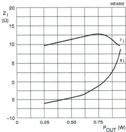
Fig.17 Input impedance as a function of output power.
