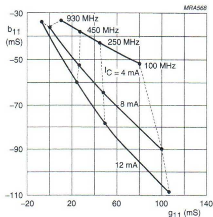
Fig.2 Common base input admittance ( Y_{11} ).
