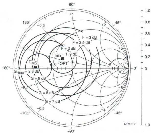
Fig.13 Noise circle figure.
