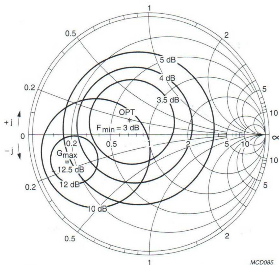
Fig.14 Common emitter noise figure circles; typical values.
