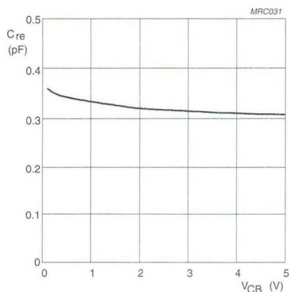
Fig.4 Feedback capacitance as a function of collector-base voltage.
