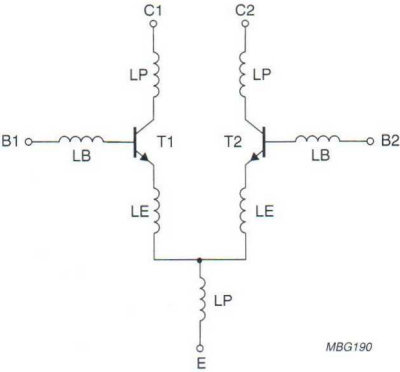
Fig.2 Package equivalent circuit SOT353B (inductance only).
