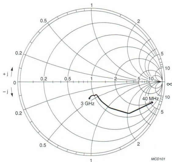
Fig.18 Common emitter output reflection coefficient ( S_{22} ).
