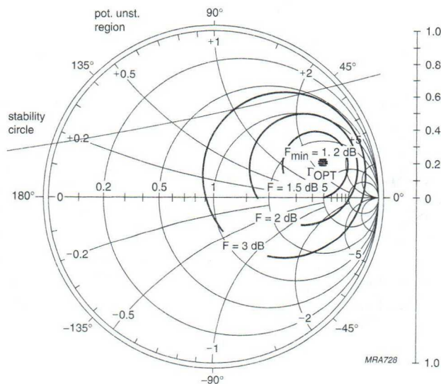
Fig.12 Noise circle figure.
