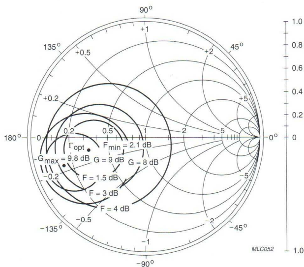
Fig.18 Common emitter noise figure circles; typical values.
