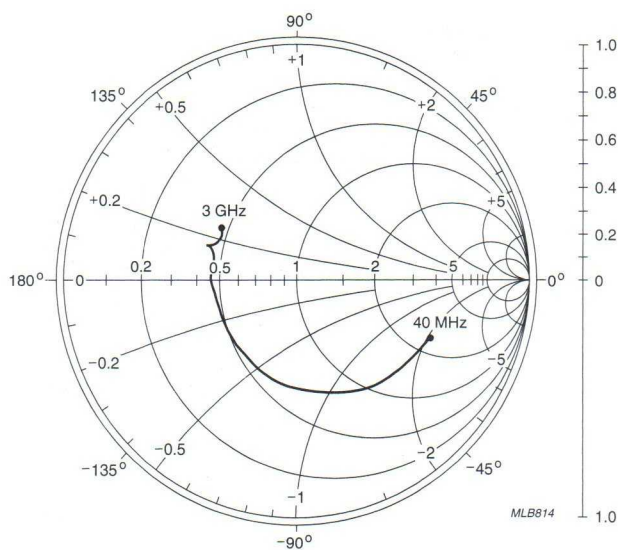
Fig.18 Common emitter input reflection coefficient ( S_{11} ); typical values.
