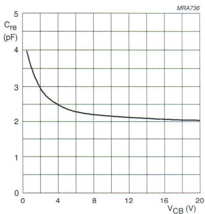
Fig.6 Feedback capacitance as a function of collector-base voltage.
