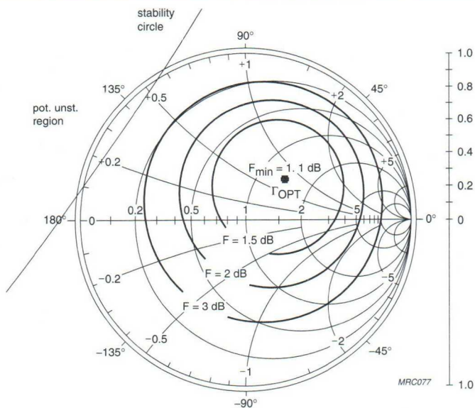
Fig.12 Noise circle.
