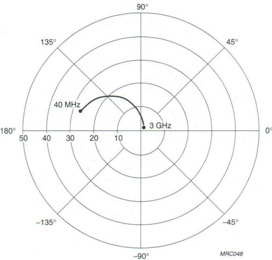
Fig.13 Common emitter forward transmission coefficient ( S_{21} ).
