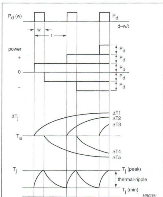
Fig.5 Heating effect of three identical power pulses after thermal stabilization.
