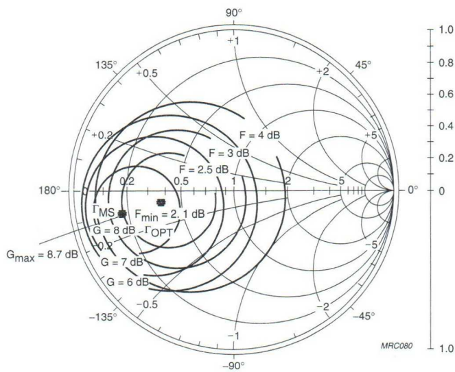
Fig.13 Noise circle.
