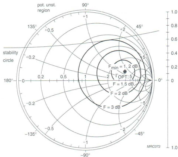
Fig.12 Noise circle.
