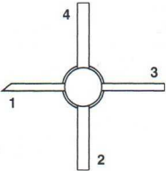
Top view MSA457
