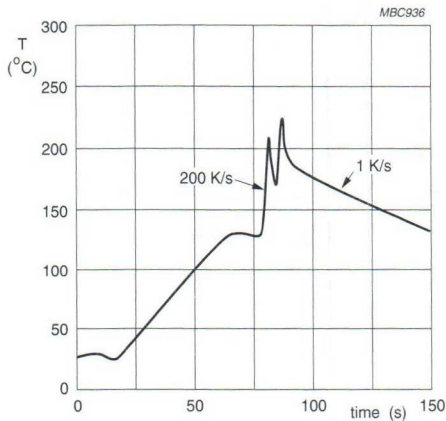
Fig.6 Typical time-temperature curve measured at the soldering site.
