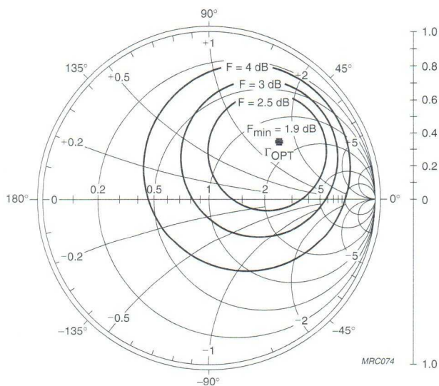
Fig.13 Noise circle.
