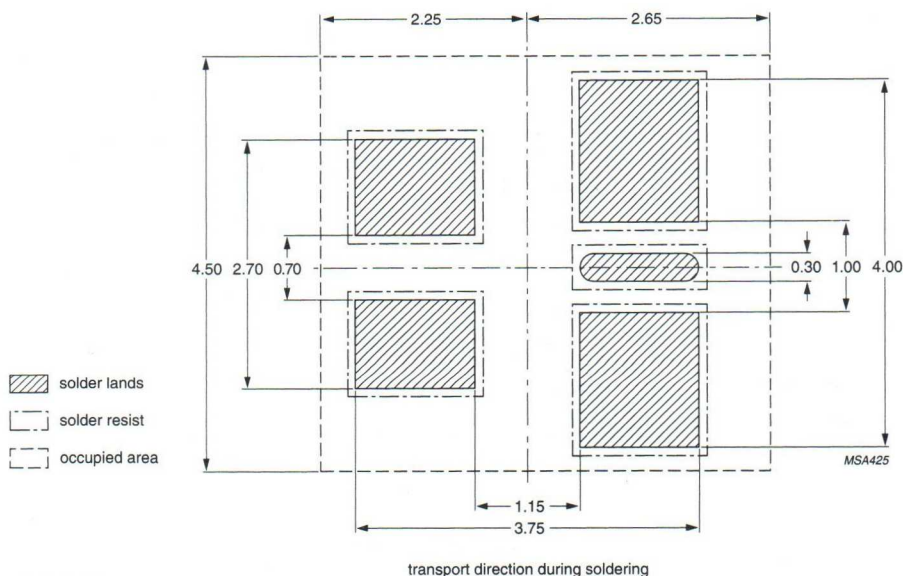
Fig.20 Wave soldering footprint for SOT353 (SC-88A); typical dimensions.
