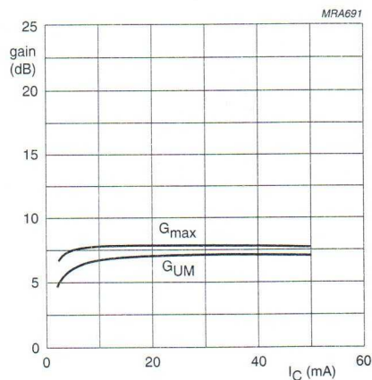
Fig.7 Gain as a function of collector current.
