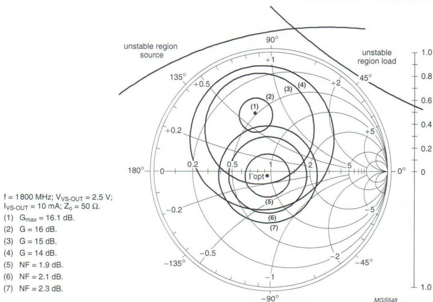
Fig.14 Noise, stability and gain circles; typical values.
