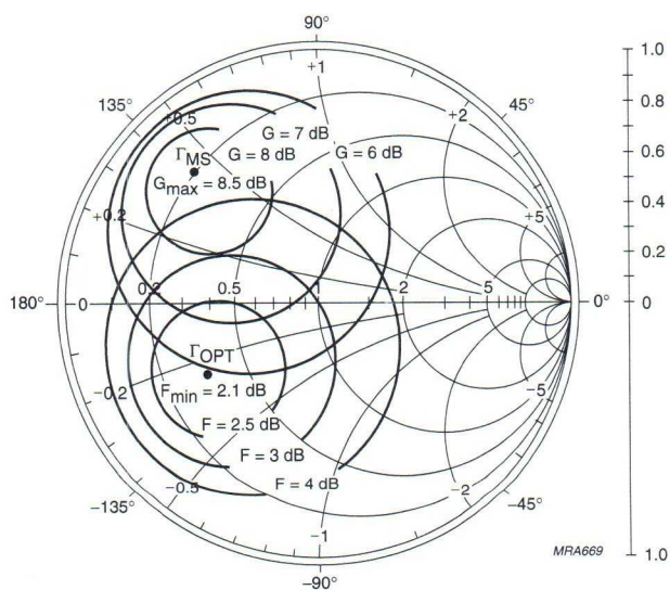
Fig.15 Noise circle figure.
