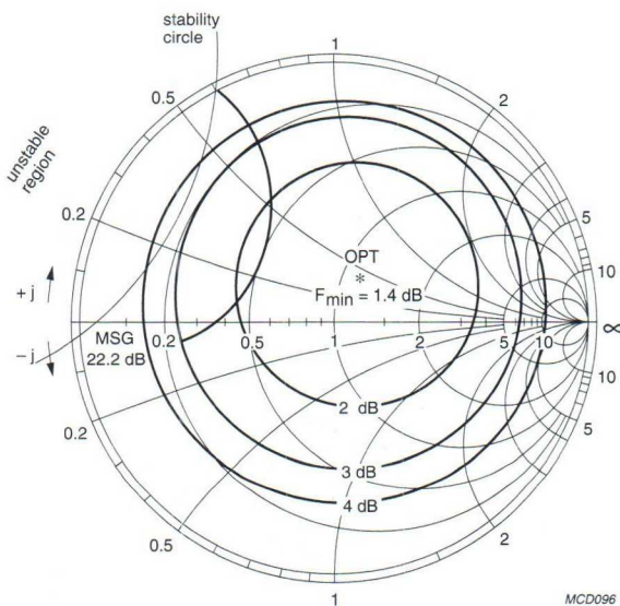
Fig.12 Common emitter noise figure circles; typical values.
