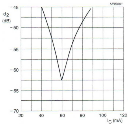
Fig.11 Second order intermodulation distortion as a function of collector current.
