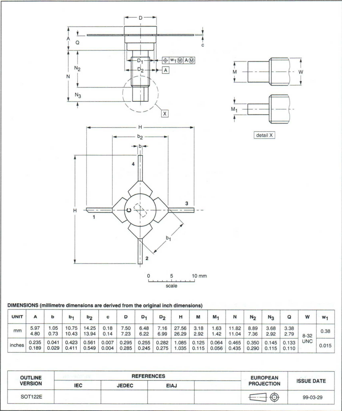
Studded ceramic package; 4 leads
