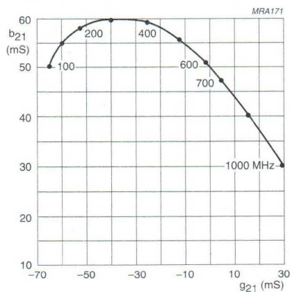
Fig.5 Common base forward transfer admittance ( Y_{21} ).
