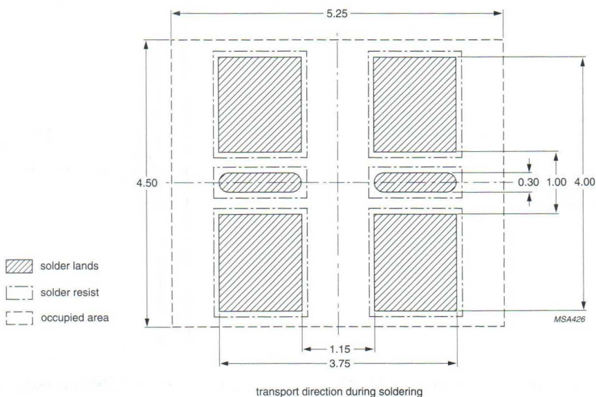
Fig.22 Wave soldering footprint for SOT363 (SC-88); typical dimensions.
