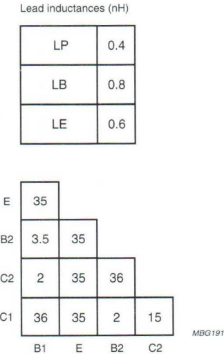
Fig.3 Package capacitance (fF) between indicated nodes.
