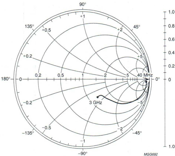
Fig.12 Common emitter output reflection coefficient ( S_{22} ); typical values.
