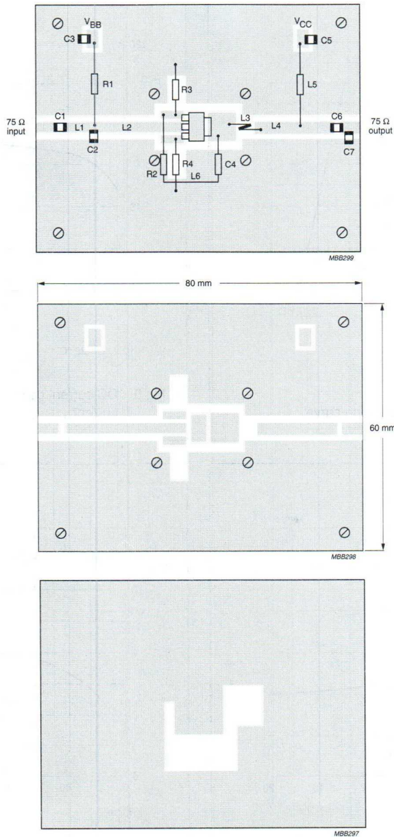
Fig.3 Intermodulation test circuit printed circuit board.
