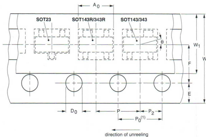
Fig.1 Specification for 8 mm tape (SOT23, SOT143, SOT143R, SOT343 and SOT343R).
