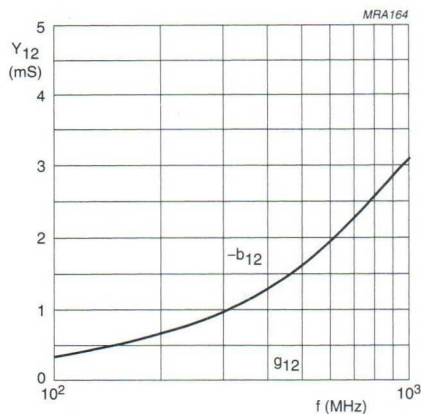
Fig.6 Common base reverse transfer admittance ( Y_{12} ) as a function of frequency.
