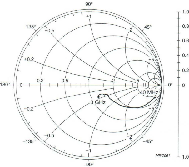
Fig.17 Common emitter output reflection coefficient ( S_{22} ).
