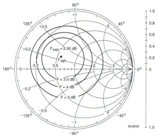
Fig.17 Common emitter noise figure circles, typical values.
