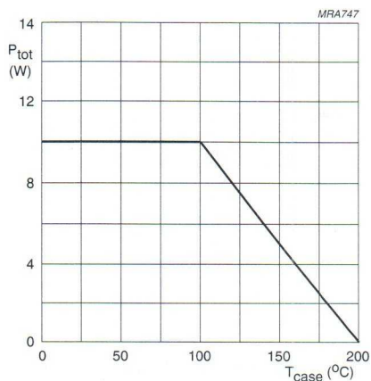
Fig.4 Power derating curve.
