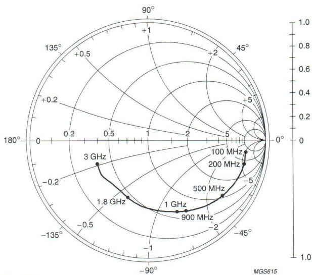
Fig.12 Common emitter input reflection coefficient ( s_{11} ); typical values.
