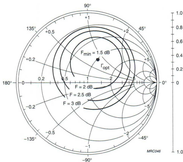
Fig.11 Noise circle.
