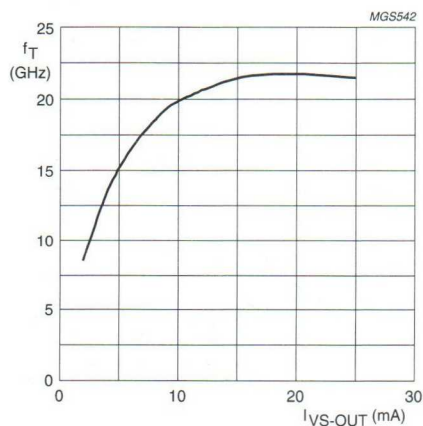
Fig.8 Transition frequency as a function of the bias current ( I_{VS-OUT} ); typical values.
