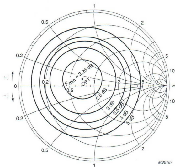
Fig.16 Noise circle.
