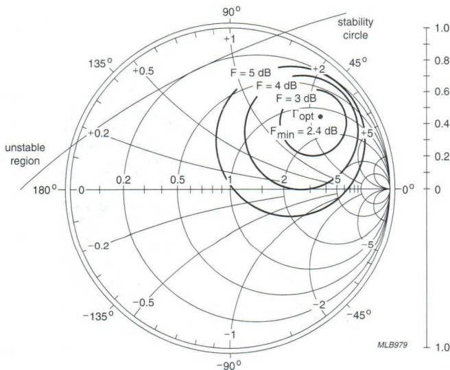
Fig.14 Common emitter noise figure circles; typical values.
