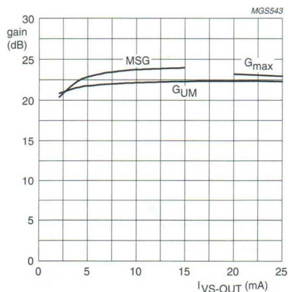
Fig.9 Gain as a function of the bias current ( I_{VS-OUT} ); typical values.
