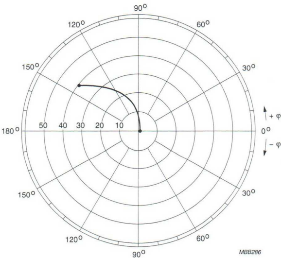
Fig.23 Common emitter forward transmission coefficient ( S_{21} ).
