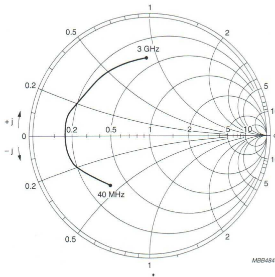
Fig.16 Common emitter input reflection coefficient ( S_{11} ).
