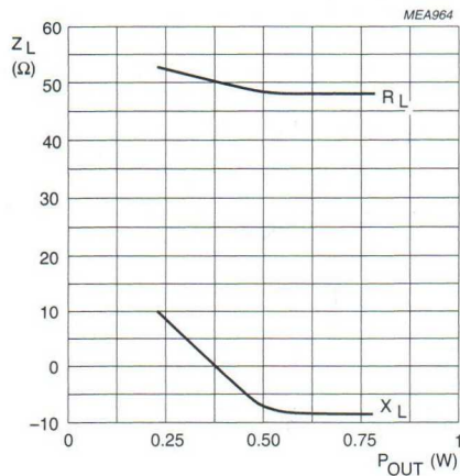
Fig.13 Load impedance as a function of output power.
