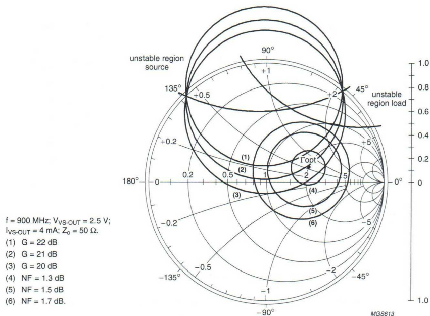
Fig.10 Noise, stability and gain circles; typical values.
