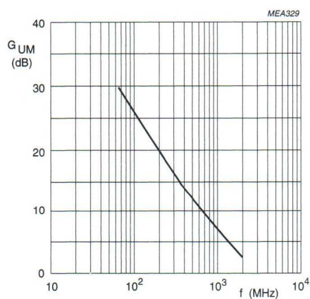
Fig.5 Maximum unilateral power gain as a function of frequency.
