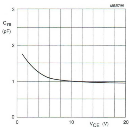
Fig.6 Feedback capacitance as a function of collector-emitter voltage.
