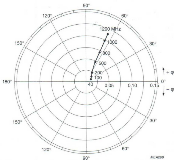
Fig.9 Common emitter reverse transmission coefficient ( S_{12} ).
