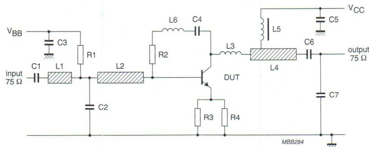
Fig.2 Intermodulation distortion and second order intermodulation distortion test circuit.
