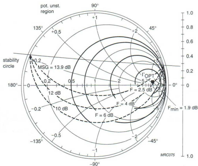
Fig.12 Noise circle.
