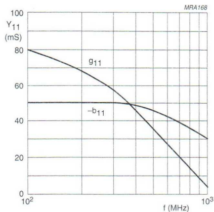
Fig.2 Common base input admittance ( Y_{11} ) as a function of frequency.
