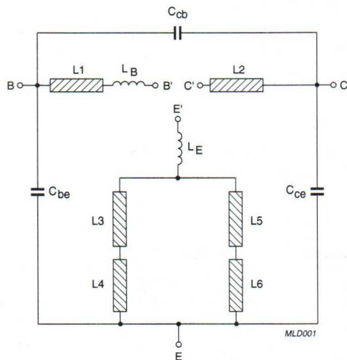
Fig.13 Package equivalent circuit SOT172A2.
