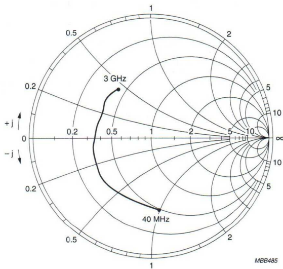
Fig.19 Common emitter output reflection coefficient ( S_{22} ).
