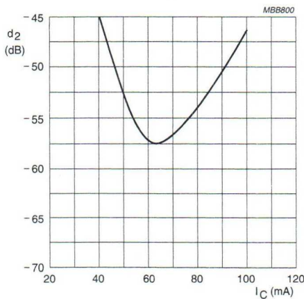
Fig.10 Second order intermodulation distortion as a function of collector current.
