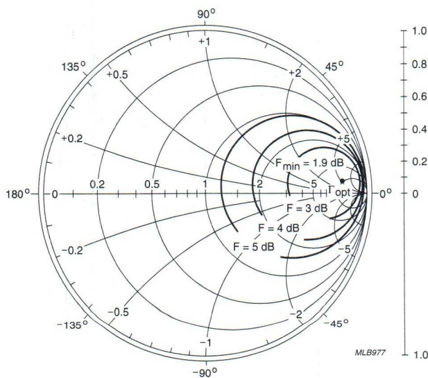
Fig.12 Common emitter noise figure circles; typical values.
