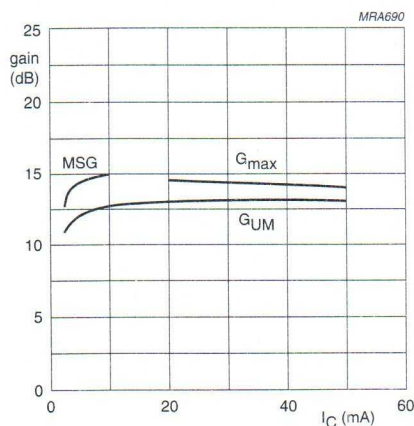
Fig.6 Gain as a function of collector current.
