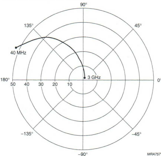
Fig.18 Common emitter forward transmission coefficient ( S_{21} ).
