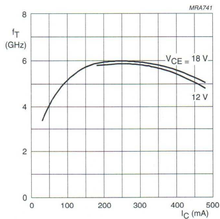
Fig.7 Transition frequency as a function of collector current.
