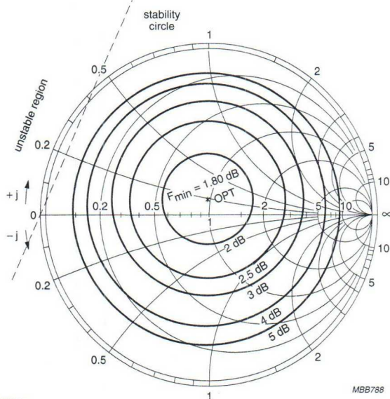
Fig.15 Noise circle.
