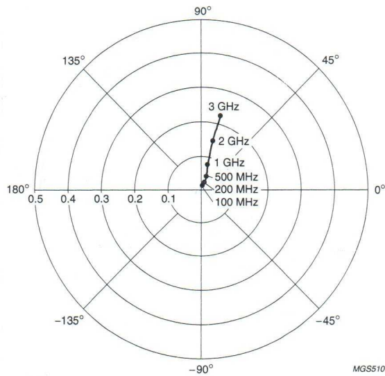
Fig.17 Common emitter reverse transmission coefficient ( s_{12} ); typical values.
