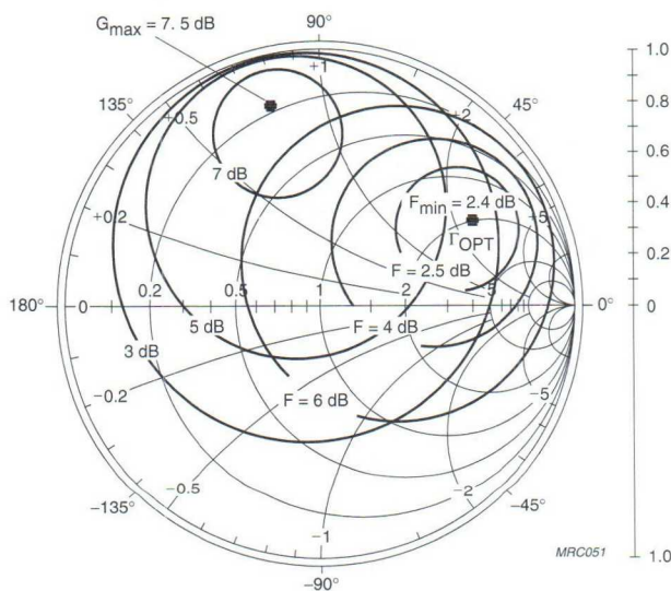
Fig.14 Noise circle.
