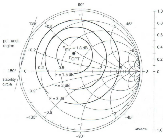
Fig.12 Noise circle figure.
