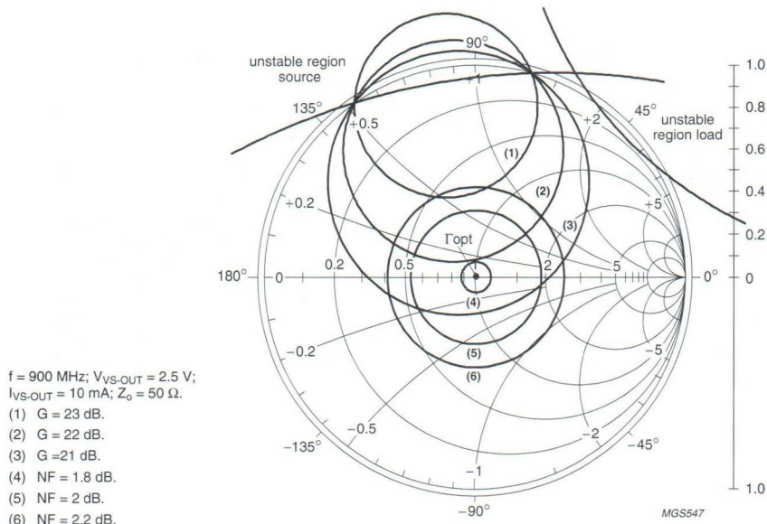
Fig.13 Noise, stability and gain circles; typical values.
