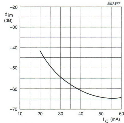
Fig.10 Intermodulation distortion as a function of collector current.
