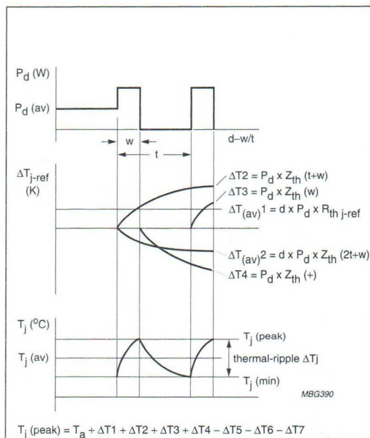
Fig.6 Two-pulse approximation method of finding peak steady-state junction temperature [T_{j(peak)}] .
