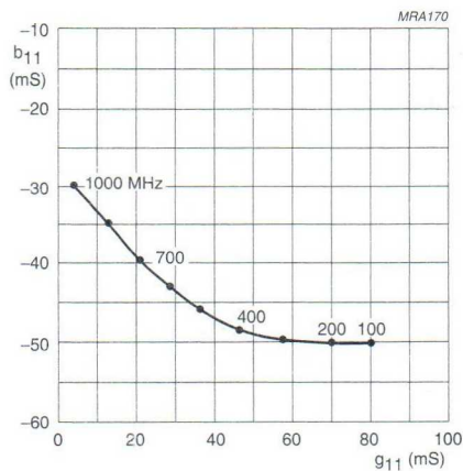
Fig.3 Common base input admittance ( Y_{11} ).
