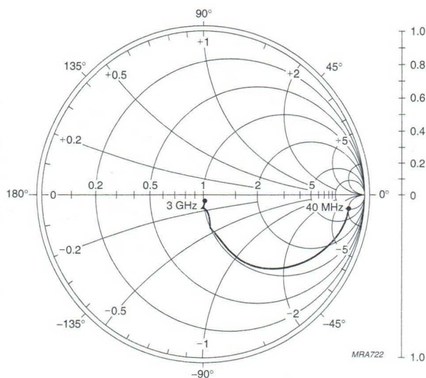
Fig.14 Common emitter input reflection coefficient ( S_{11} ).
