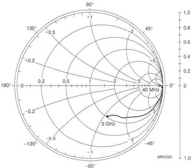
Fig.18 Common emitter output reflection coefficient ( S_{22} ).
