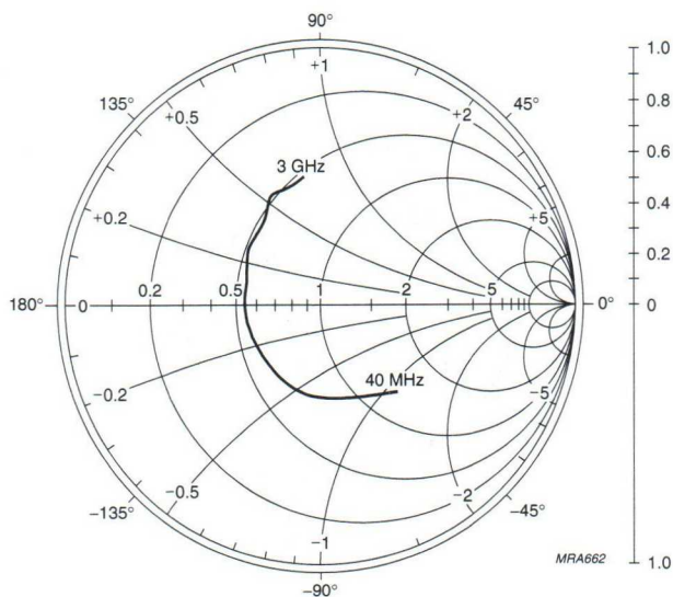
Fig.16 Common emitter input reflection coefficient ( S_{11} ).
