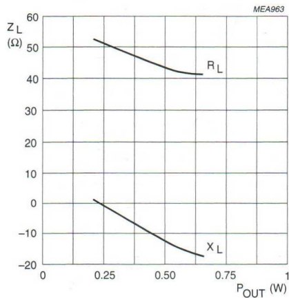
Fig.12 Load impedance as a function of output power.
