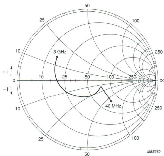
Fig.9 Common emitter output transmission coefficient ( S_{22} ).
