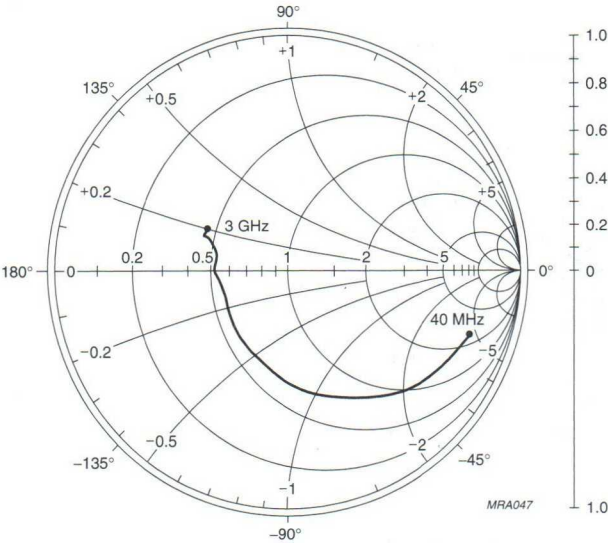
Fig.12 Common emitter input reflection coefficient ( S_{11} ).
