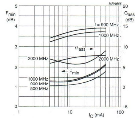
Fig.12 Minimum noise figure and associated available gain as functions of collector current.
