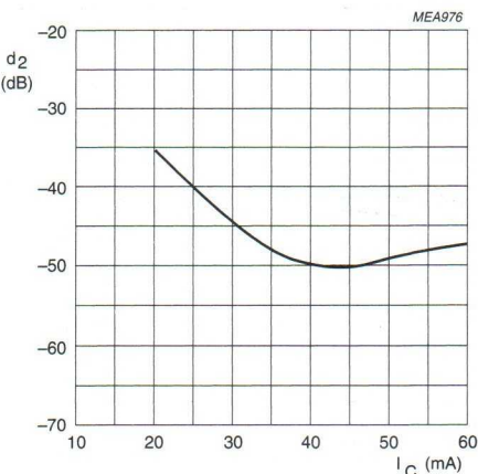
Fig.11 Second order intermodulation distortion as a function of collector current.
