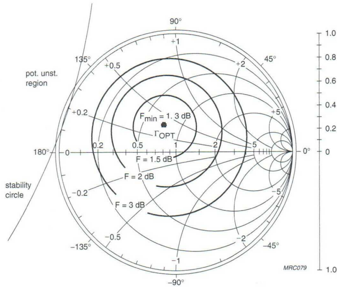
Fig.12 Noise circle.
