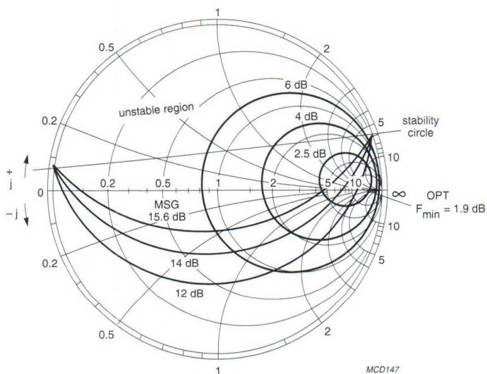
Fig.12 Common emitter noise figure circles; typical values.
