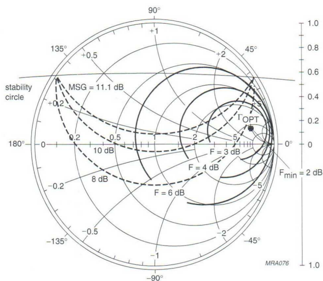
Fig.13 Noise circle.
