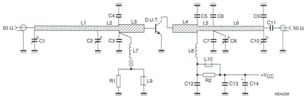
Fig.4 Class-B test circuit at f = 900 \text{ MHz} .
