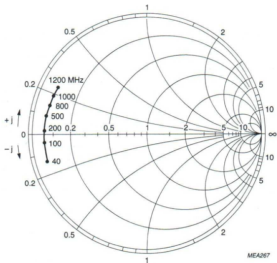
Fig.7 Common emitter input reflection coefficient ( S_{11} ).
