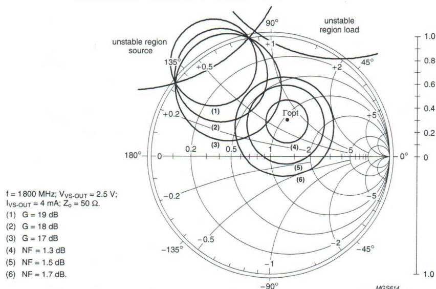
Fig.11 Noise, stability and gain circles; typical values.
