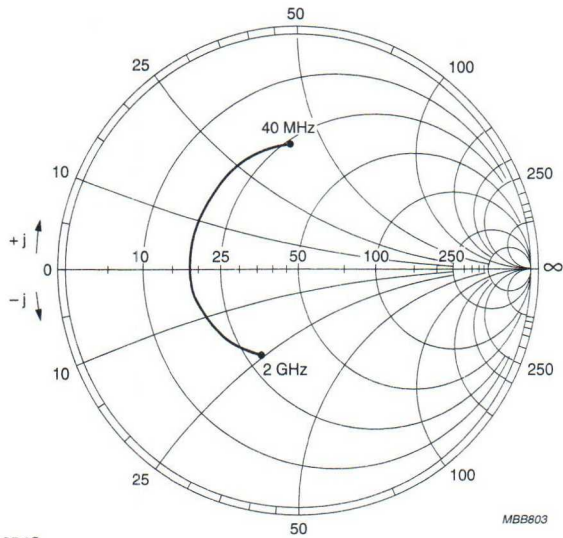
Fig.22 Common emitter input reflection coefficient ( S_{11} ).
