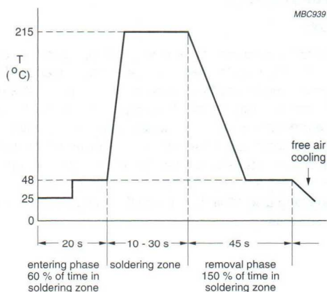
Fig.3 Theoretical time/temperature curve relationship for dual vapour reflow soldering.
