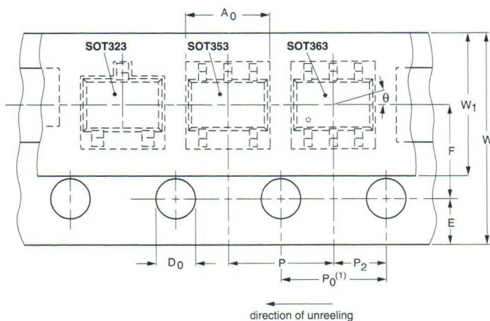
Fig.2 Specification for 8 mm tape (SOT323, SOT353 and SOT363).
