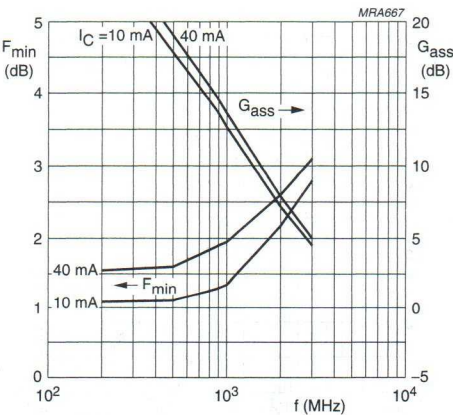
Fig.13 Minimum noise figure and associated available gain as functions of frequency.
