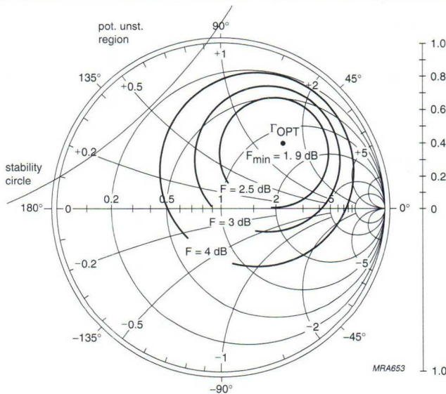
Fig.15 Common emitter noise figure circles; typical values.
