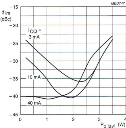
Fig.7 Intermodulation distortion as a function of average output power.
