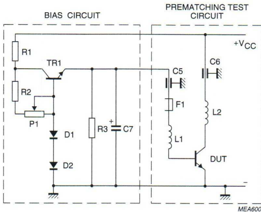
Fig.4 Class AB bias circuit.
