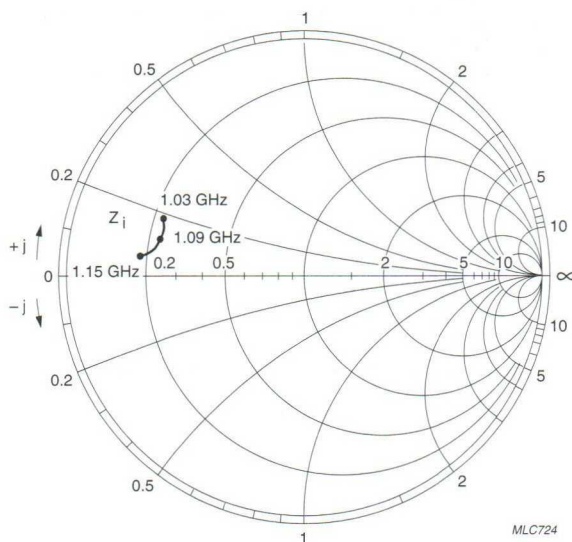
Fig.6 Input impedance as a function of frequency.
