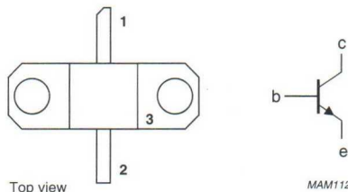
Fig.1 Simplified outline and symbol.
