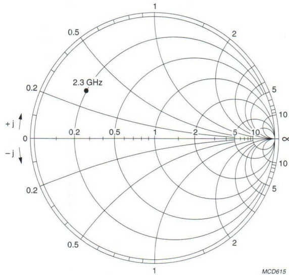
Fig.5 Input impedance as a function of frequency.
