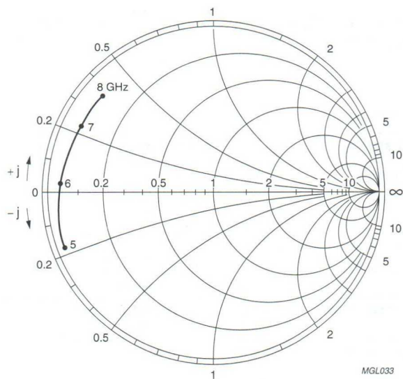
Fig.3 Emitter reflection coefficient.
