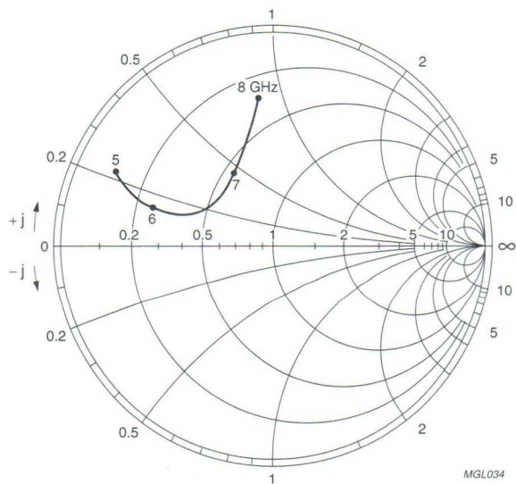
Fig.4 Base reflection coefficient
