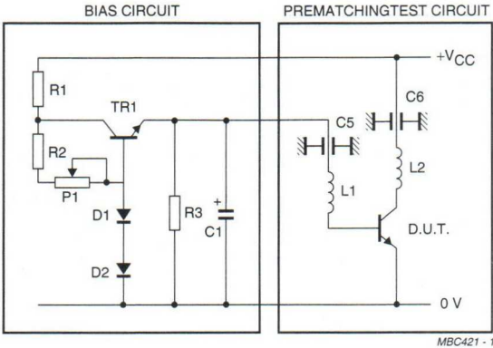
Fig.5 Class AB bias circuit at 1.65 GHz.
