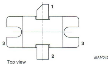
Fig.1 Simplified outline and symbol.
