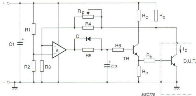
Fig.3 Bias circuit for a class-A linear microwave transistor.
