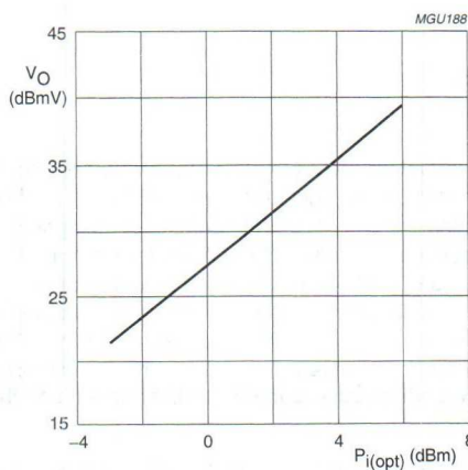
Fig.7 Output voltage as a function of the optical input power P_{i(opt)} .
