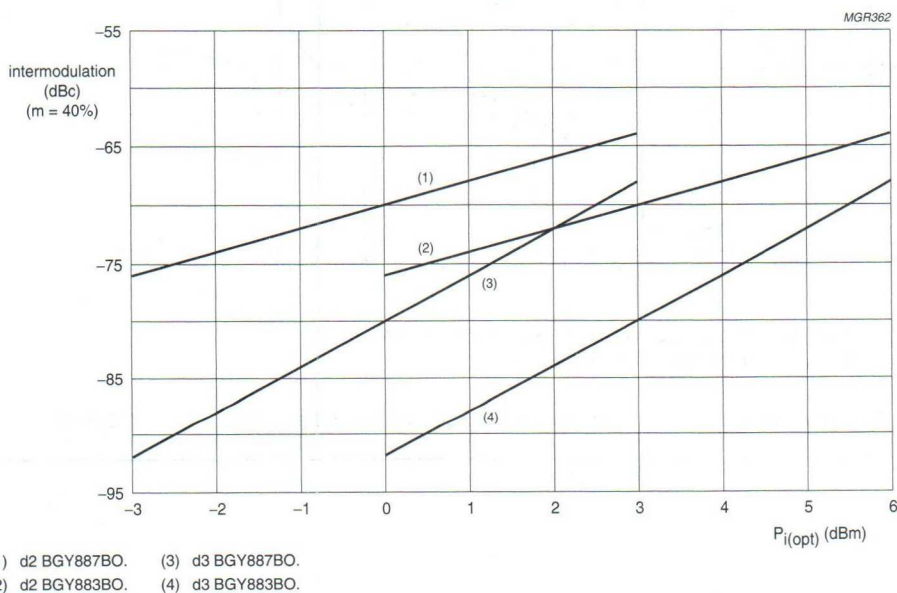
Fig.9 d2 and d3 as a function of the optical input power P_{i(opt)} .
