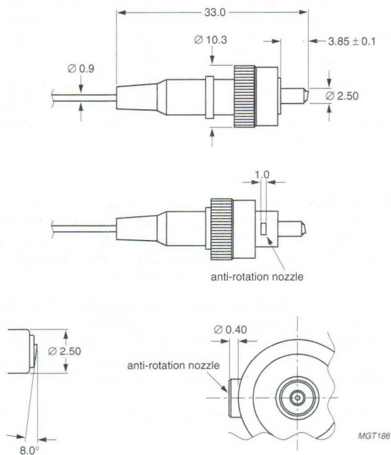
Fig.17 FC0/APC connector.
