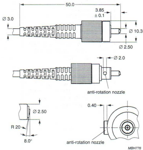
Fig.3 FC/APC connector.
