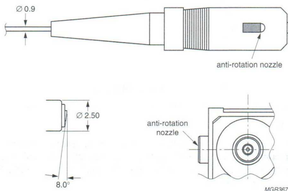
Fig.18 SC0/APC connector.
