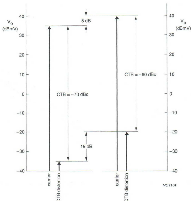
Fig.12 Output voltage of carrier V_O , CTB distortion V_{CTB} and CTB.
