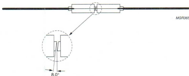
Fig.16 Two mated APC ferrules.
