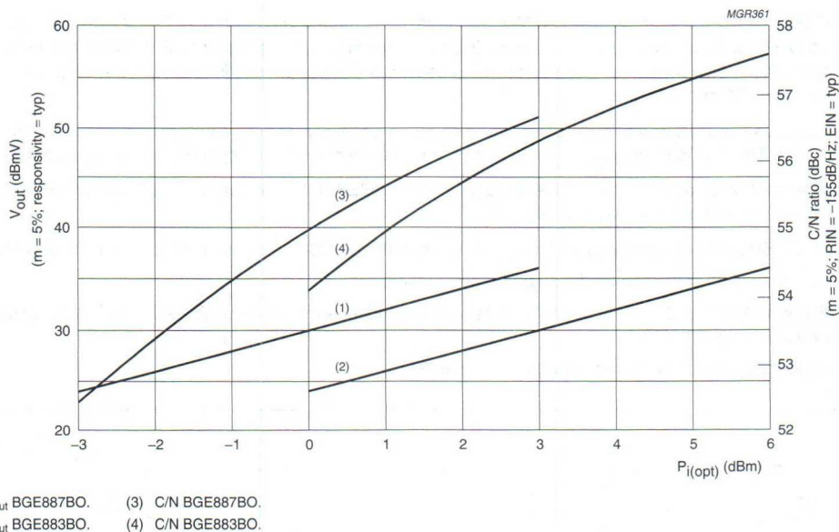
Fig.8 V_{out} and C/N ratio as a function of the optical input power P_{i(opt)} .
