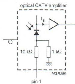
Fig.4 The diode current monitor pin.
