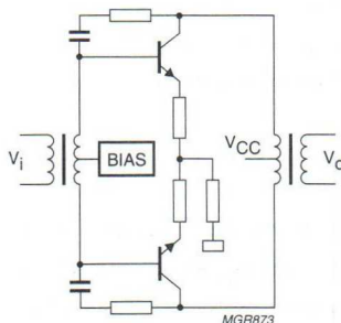
Fig.1 Simplified wideband module.
