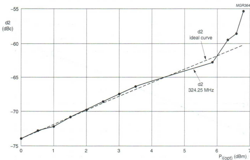
Fig.15 d_2 as a function of the optical input power P_{i(opt)} .
