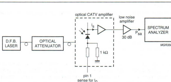
Fig.2 Equivalent input noise measurement set-up.
