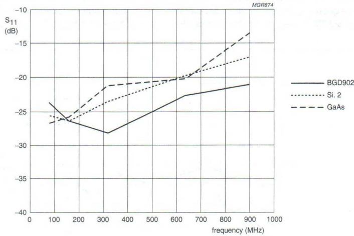
Fig.5 S_{11} as function of frequency, mean values.
