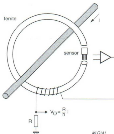
Fig.44 Current measurement using a compensating coil.
