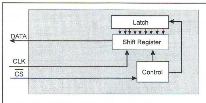
Figure 15: Slave-SPI Block Diagram
