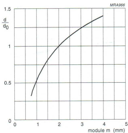
Fig.12 Normalized maximum sensing distance as a function of gear wheel module; typical values.
