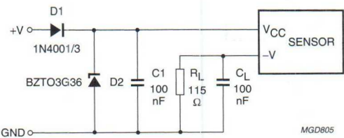
Fig.11 Test/application circuit for the KMI20/1.
