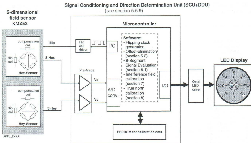
Figure 28 8-segment compass with microcontroller
