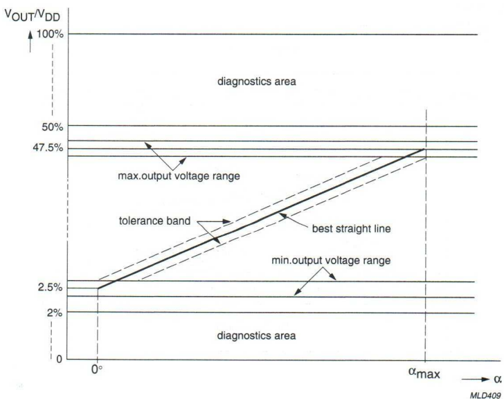
Fig.5 Half range analog output mode (Mode 2).
