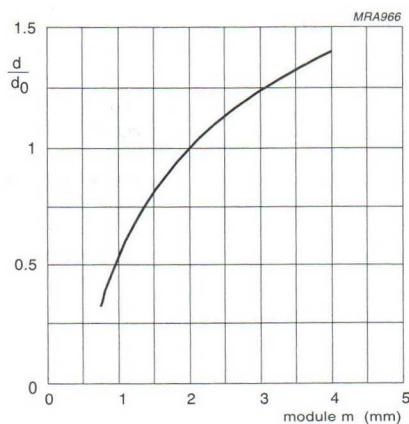
Fig. 14 Normalized maximum sensing distance as a function of gear wheel module; typical values.
