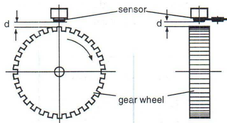
Figure 14: Definition of the sensing distance d
