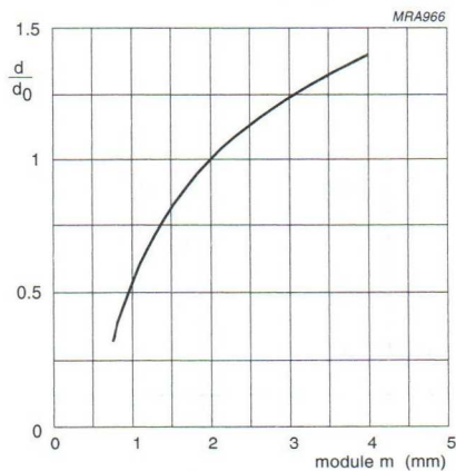
Fig.10 Normalized maximum sensing distance as a function of gear wheel module; typical values.
