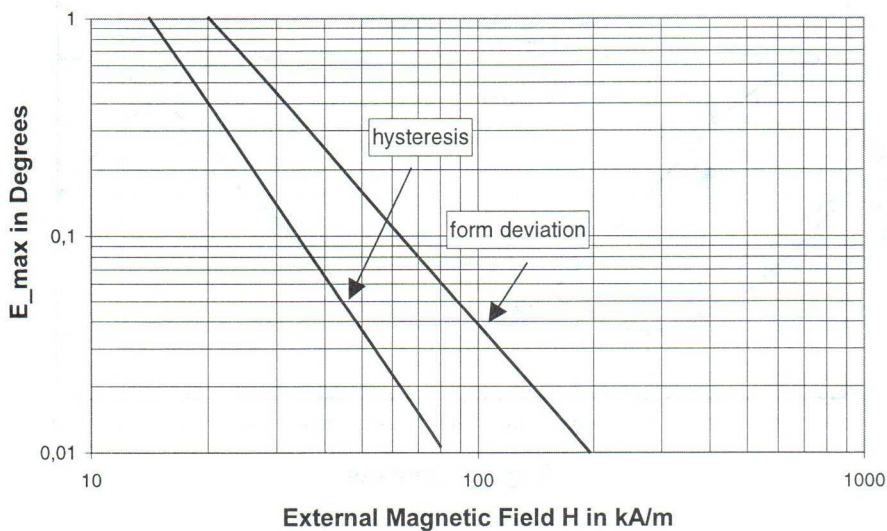
Figure 24: Maximum measurement error caused by signal form error and hysteresis
