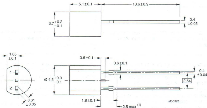
Fig.6 Outline of the KTY81 (SOD70).
