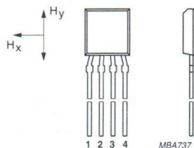
Fig.1 Simplified outline.
