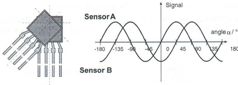
Figure 4 Output signal from a double Wheatstone bridge sensor (KMZ41)
