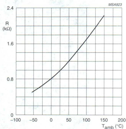
Fig.2 Characteristic of KTY81.
