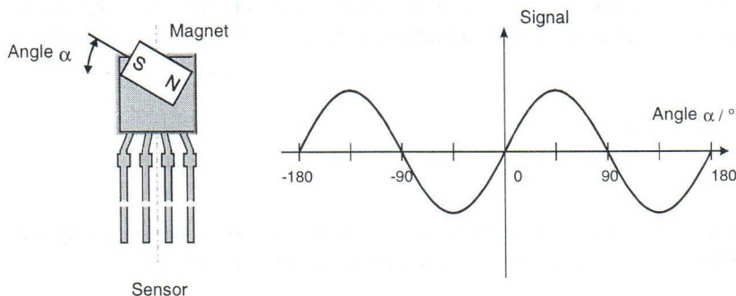
Figure 3: Output signal from a single Wheatstone bridge sensor
