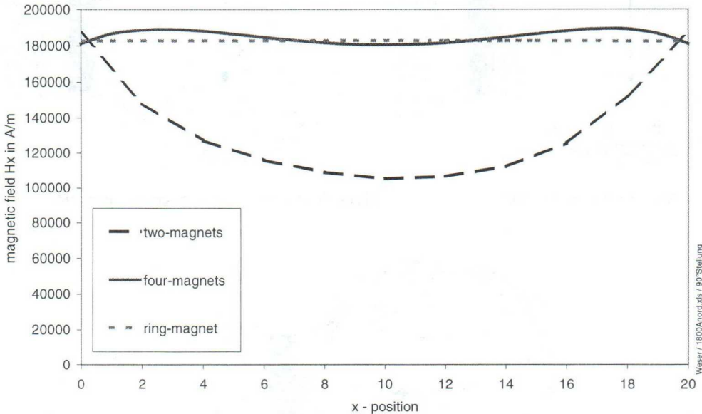
Figure 13: Simulation of the magnetic field strength H_{x_{\text{simulated}}} for different magnet arrangements (two-, four-magnet and ring-magnet arrangement)
