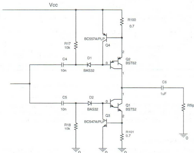
Figure 16 Flip circuit with active current limiting
