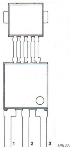
Fig.1 Simplified outline (SOT477A).
