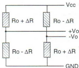
Figure 7 Bridge configuration of barber pole sensors
