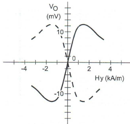
Figure 5: Reversal of sensor characteristic caused by flipping
