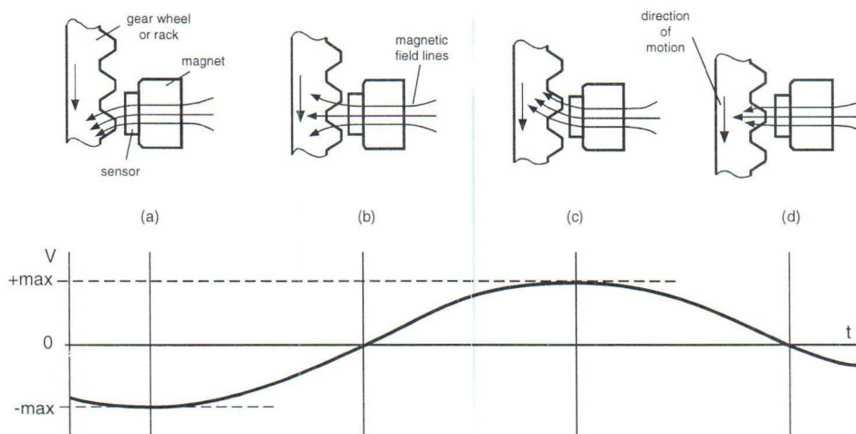
Figure 1: Sensor signal generation in MR-sensors
