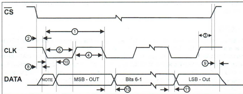
Figure 17: UZZ9001 SPI Interface Timing
