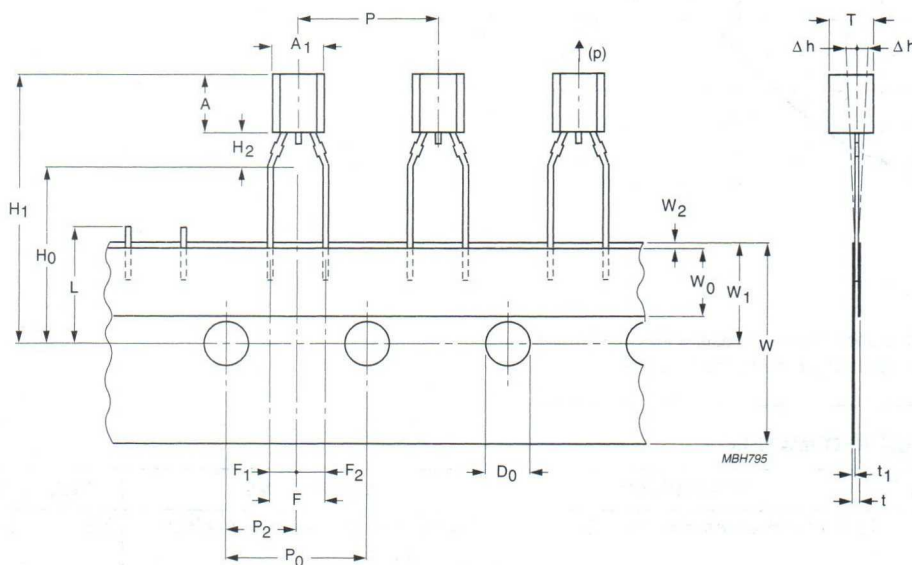
Fig.7 Configuration of bandolier: spread leads.
