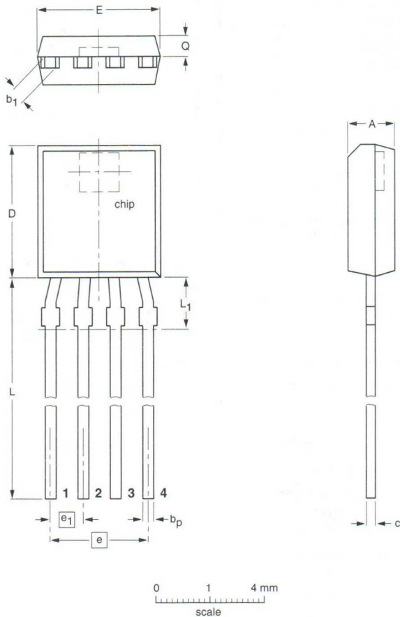
DIMENSIONS (mm are the original dimensions)
