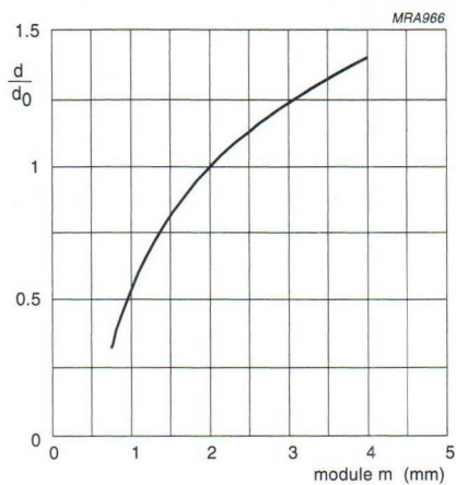
Fig.16 Normalized maximum sensing distance as a function of gear wheel module; typical values.
