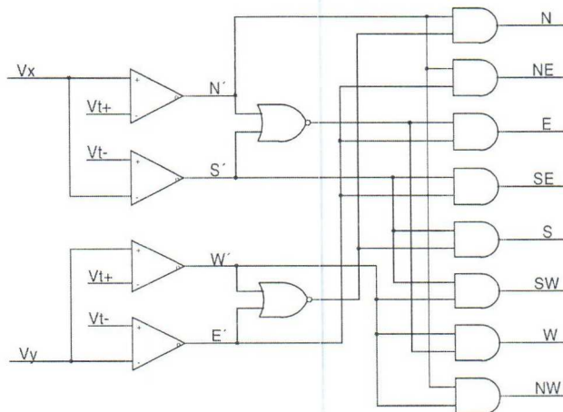
Figure 19 Circuit for 8-segment compass
