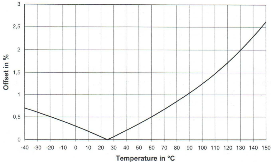
Figure 30: Offset drift at different maximum temperatures assuming the data defined in the text.
