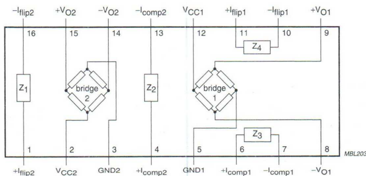
Fig.3 Simplified circuit diagram.
