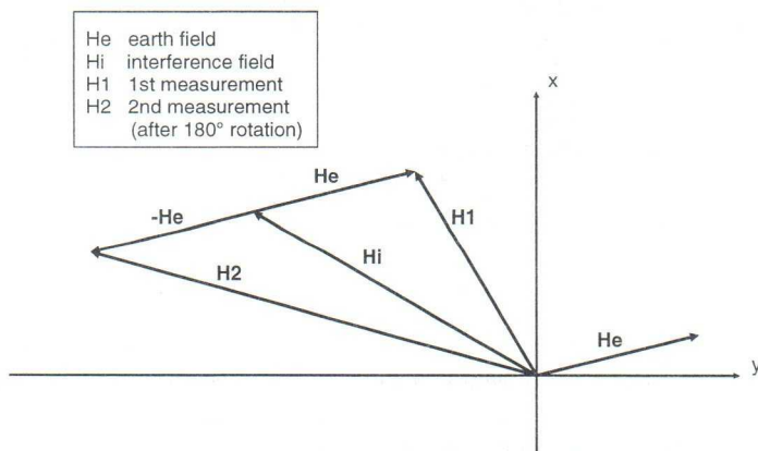
Figure 21 Principle of bidirectional calibration
