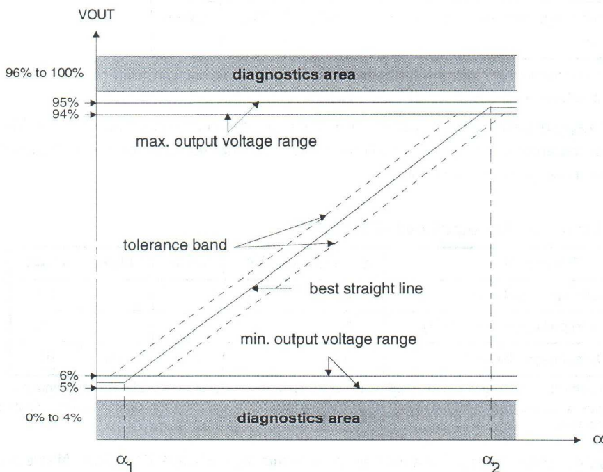
Figure 12: Detailed output curve characteristic of the UZZ9000
