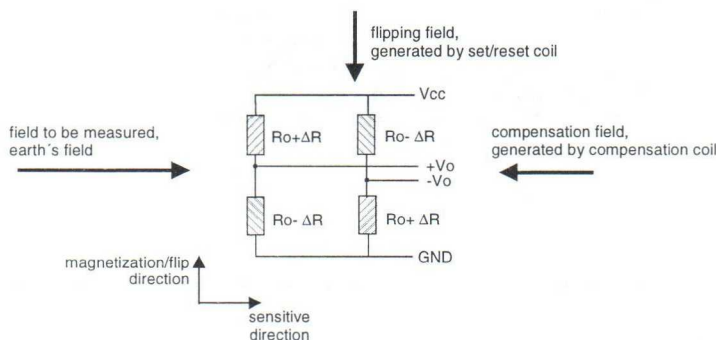
Figure 8 Fields generated by set/reset and compensation coil
