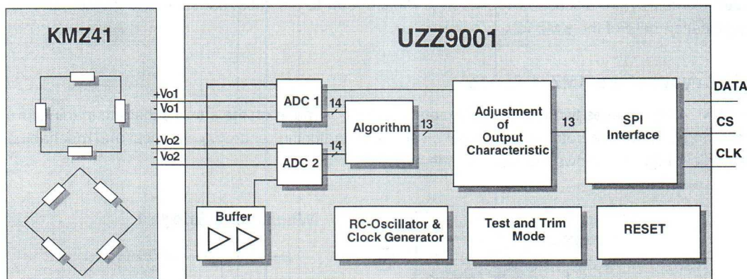
Figure 5: Block diagram of the two-chip measurement system
