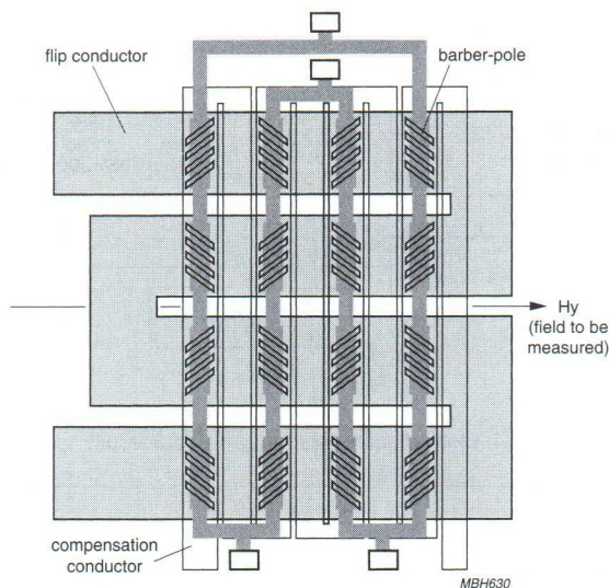
Fig.35 Layout of Philips' KMZ51 magnetoresistive sensor.
