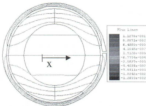
Figure 12: Flux lines of a ring-magnet arrangement
