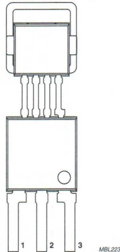
Fig.1 Simplified outline (SOT477C).
