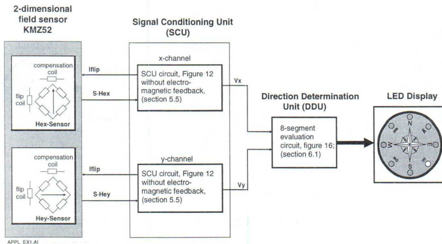
Figure 26 Analog 8-segment compass
