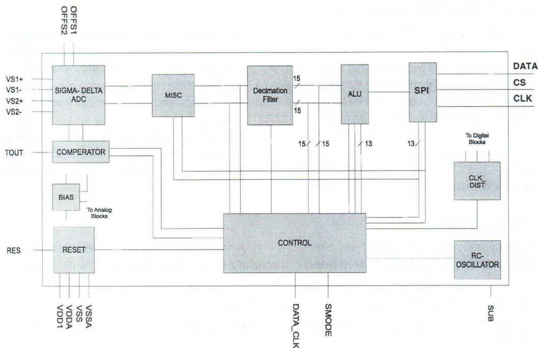
Figure 14: Detailed block diagram of the UZZ9001
