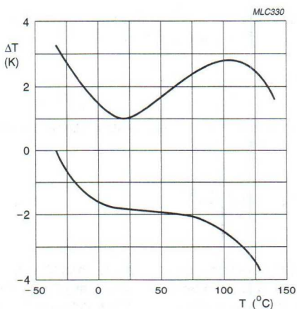
Fig.13 Combined effects of manufacturing tolerances and linearization errors for the KTY81 sensor.
