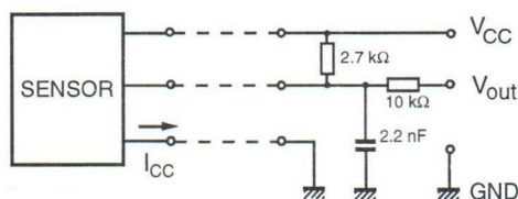
Figure 24: Test Circuit for KMI 16/x
