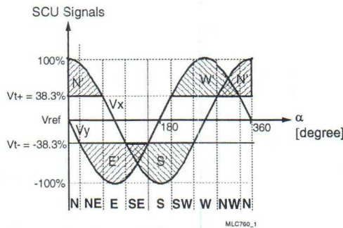
Figure 18 Direction determination for 8-segment compass
