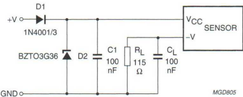
Fig.18 Test/application circuit for the KMI15/1.
