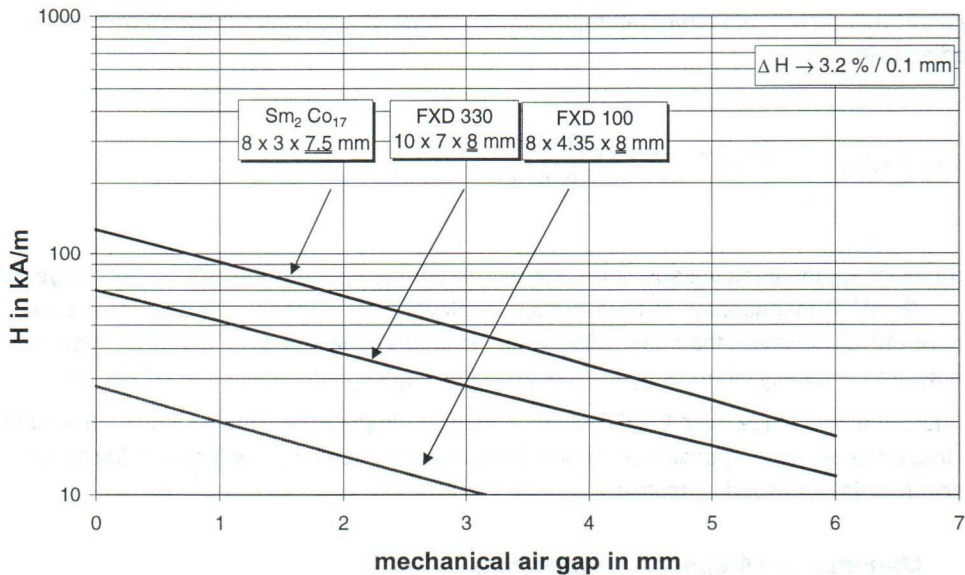
Figure 9: Field strength in the sensitive plane of the KMZ41 in dependence of the air gap between the top of the sensor package and the block magnet. The underlined dimension characterises the direction of magnetization.
