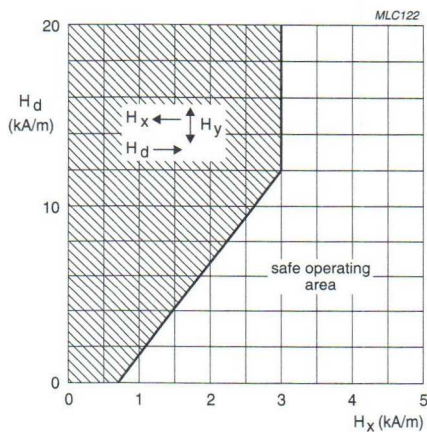
Fig.4 Safe Operating Area (permissible disturbing field H_d as a component of auxiliary field H_x ).
