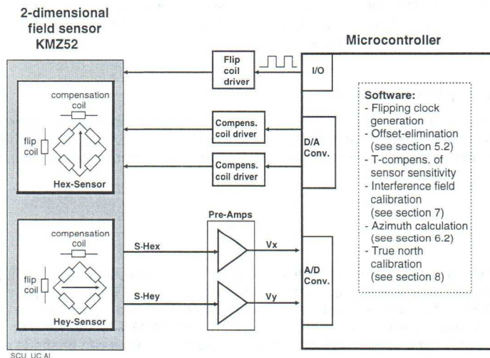
Figure 17 Signal conditioning circuit with microcontroller
