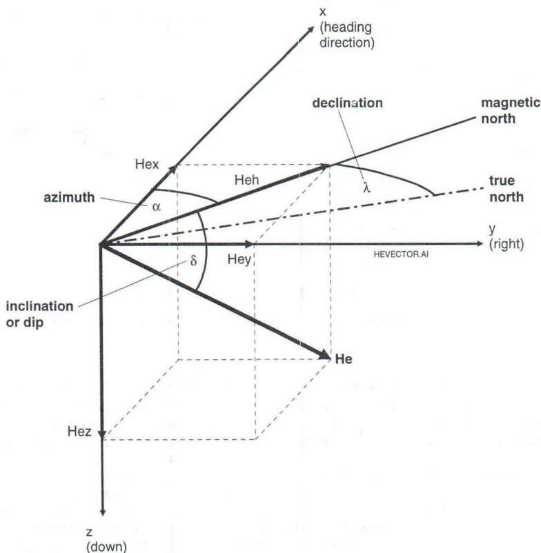
Figure 2 Earth field vector
