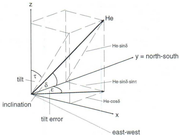
Figure 22 Tilt error
