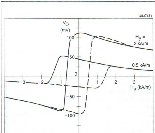
Fig.22 Sensor output ' V_O ' as a function of the auxiliary field H_x .
