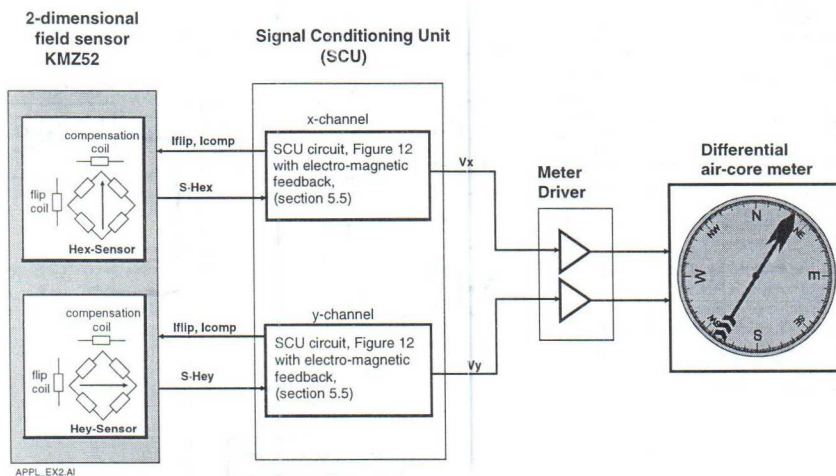
Figure 27 Analog high resolution compass
