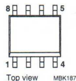
Fig.1 Simplified outline SOT96-1.
