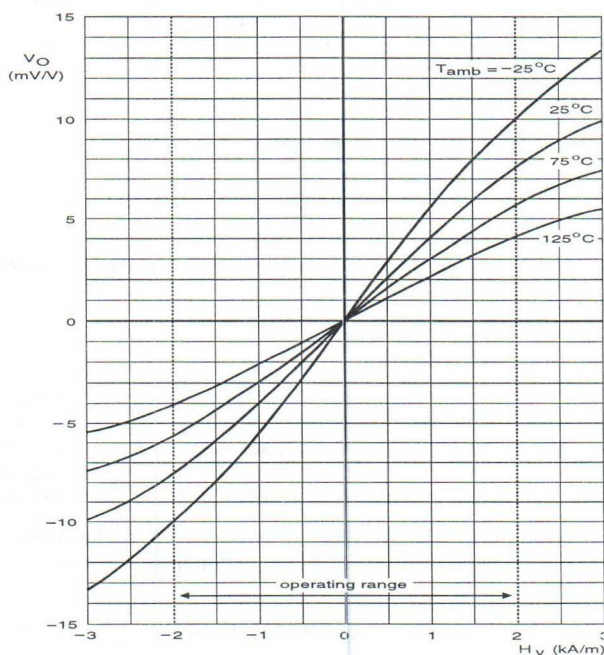
Figure 13 Typical MR sensor output characteristic (KMZ10)
