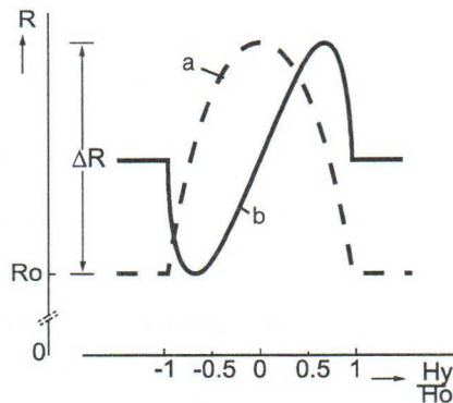
Figure 4: a) R-H characteristic of a standard sensor, b) R-H characteristic of barber pole sensors
