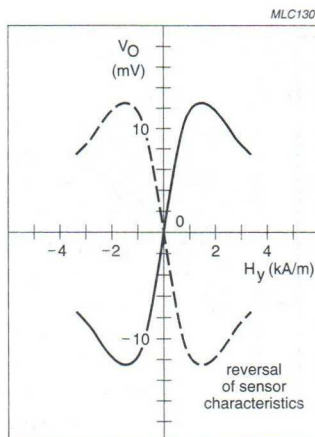
Fig.21 Sensor characteristics.
