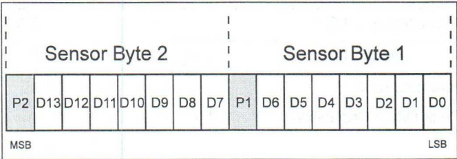
Figure 16: Coding of the digital output
