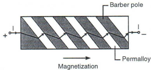
Figure 3: Linearization of the magnetoresistive effect
