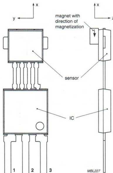
Fig.2 Component detail and coordinate system.
