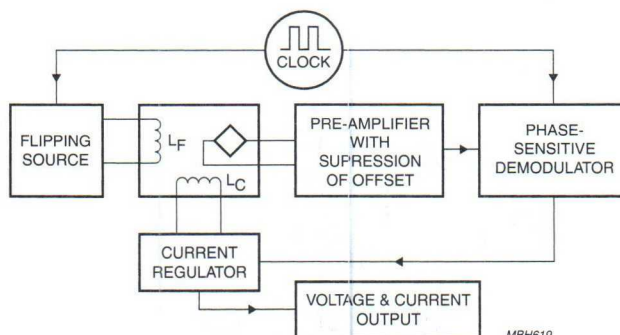
Fig.34 Block diagram of compensation circuit.
