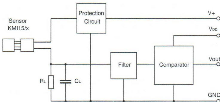
Figure 26: Block diagram of a suitable application circuit
