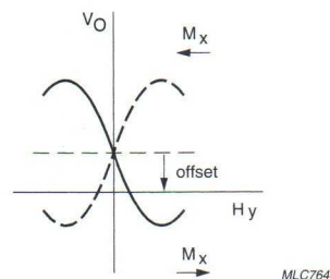
Fig.27 Butterfly curve including offset.
