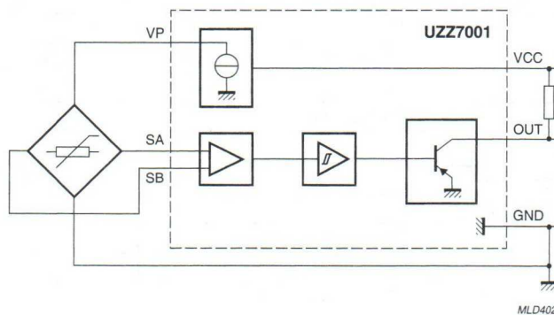
Fig.4 Circuit block diagram.
