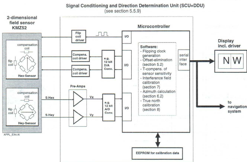
Figure 29 High-end compass with microcontroller
