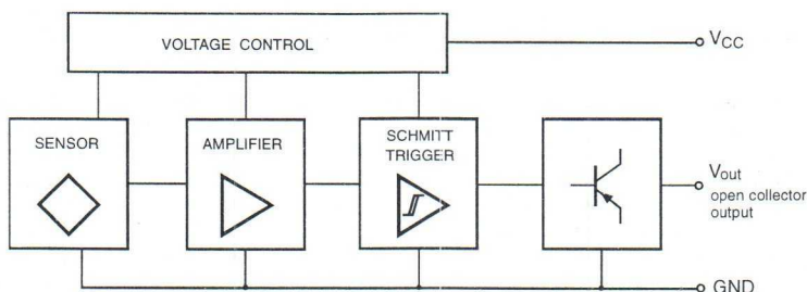
Figure 12: Block diagram of the KMI16/x sensors with open collector output.
