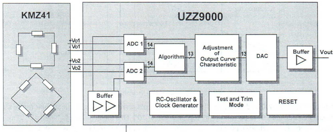
Figure 5: Block diagram of the two-chip measurement system
