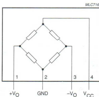
Fig.2 Simplified circuit diagram.
