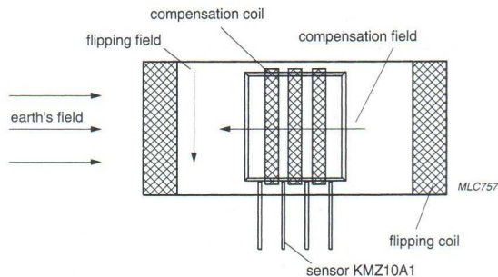
Fig.33 Magnetic field directions and the flipping and compensation coils.
