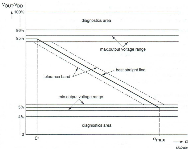
Fig.4 Inverted analog output mode (Mode 1).
