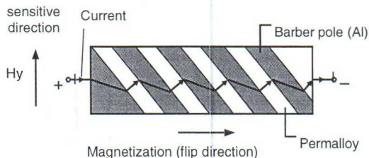
Figure 6 Barber pole sensor
