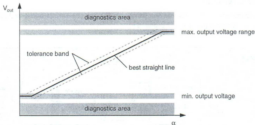
Figure 6: UZZ9000 output characteristic
