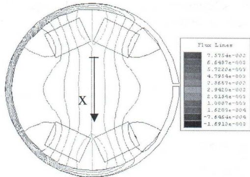
Figure 11: Flux lines of a four-magnet arrangement.
