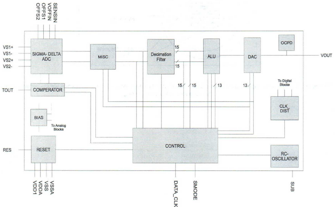
Figure 11: Detailed block diagram of the UZZ9000
