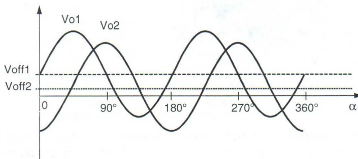
Figure 8: Output signals of the KMZ41
