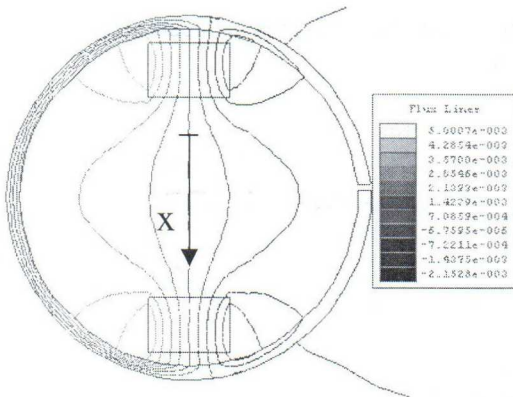
Figure 10: Flux lines of a two-magnet arrangement
