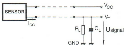
Figure 23: Test circuit for KMI15/x
