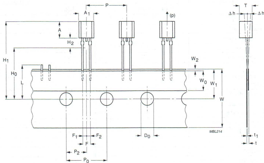
Fig.8 Configuration of bandolier: straight leads.
