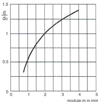
Figure 17: Normalised maximum sensing distance as a function of the module m for the KMI 15/1-sensor module
