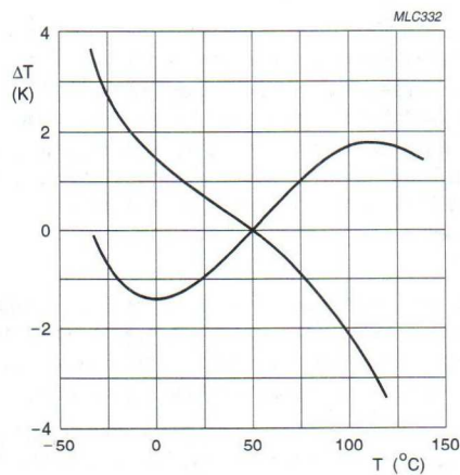
Fig.14 Maximum expected temperature error of a KTY81-1 sensor plus linearization resistor calibrated at 50 °C.
