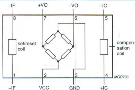
Figure 9 Simplified circuit diagram of KMZ 51
