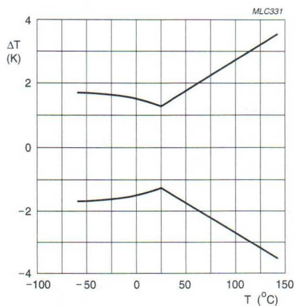
Fig.12 Maximum temperature error 'ΔT' due to manufacturing tolerances expected of a KTY81-1 sensor.
