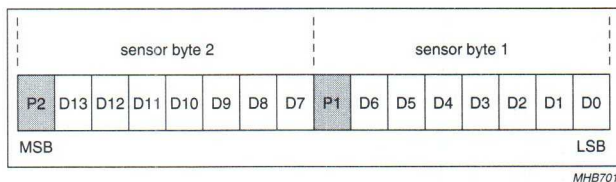
Fig.6 Digital output coding.
