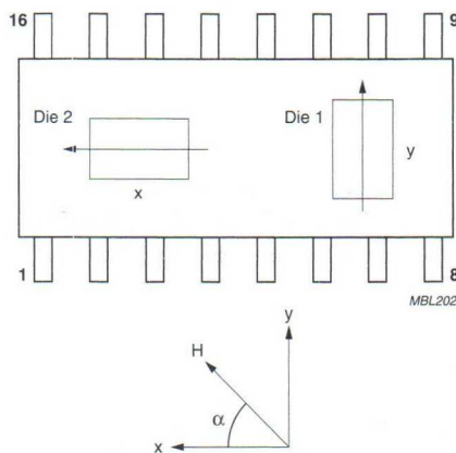
Fig.2 Angular relationship of dice.
