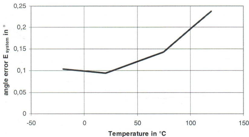
Figure 32: Measured angle error E_{\text{system}} for a typical set-up
