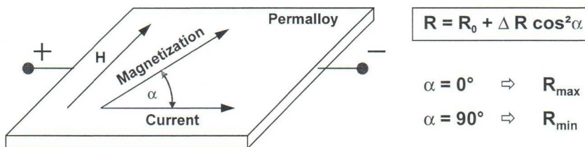
Figure 1: The magnetoresistive effect in permalloy
