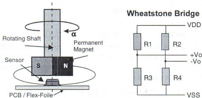
Figure 2 Basic arrangement of sensor and magnet for contactless angle measurement.
