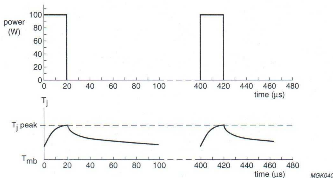
Fig.11 Periodic rectangular pulse.
