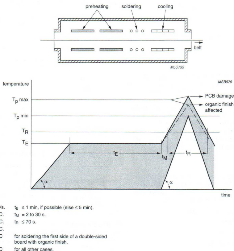
Fig.5 Convection reflow soldering method (top), process requirements for reflow soldering (bottom).
