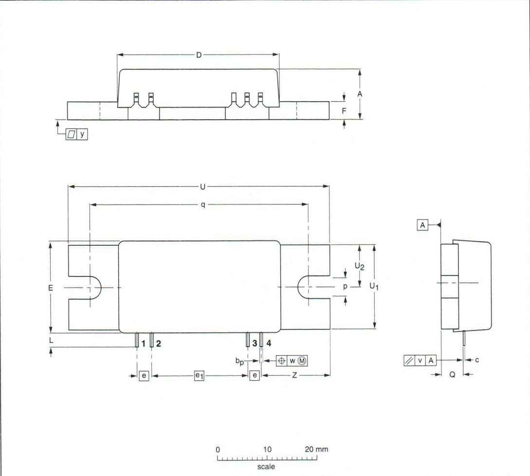
Plastic rectangular single-ended flat package; flange mounted; 2 mounting holes; 4 in-line leads SOT365B
