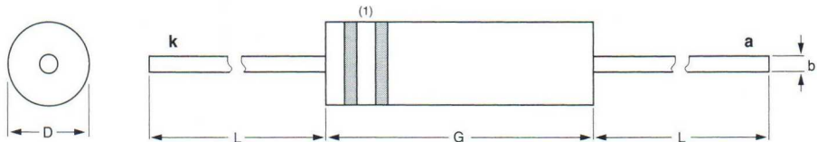
DIMENSIONS (mm are the original dimensions)
