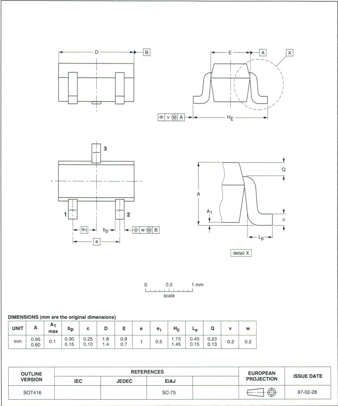
Plastic surface mounted package; 3 leads
