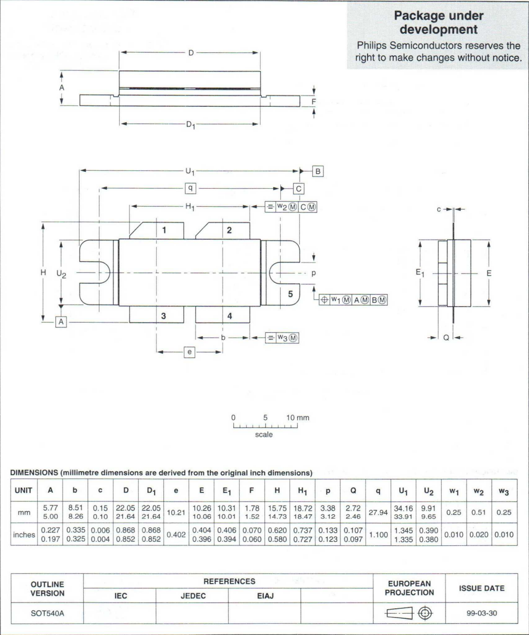
Flanged balanced LDMOST package; 2 mounting holes; 4 leads
