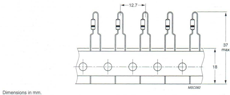
Fig.17 Radial taped components for ammo pack.
