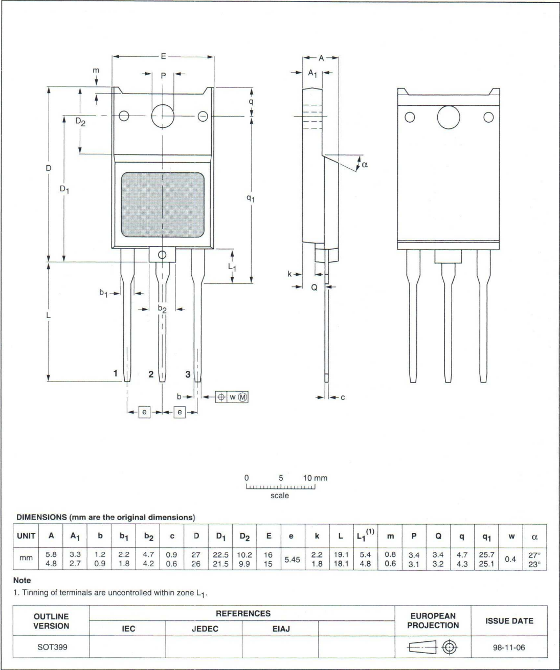
Plastic single-ended through-hole package; mountable to heatsink; 1 mounting hole; 3 in-line leads SOT399
