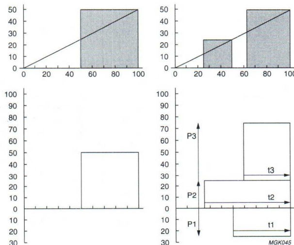
Fig.16 Non-rectangular waveform.
