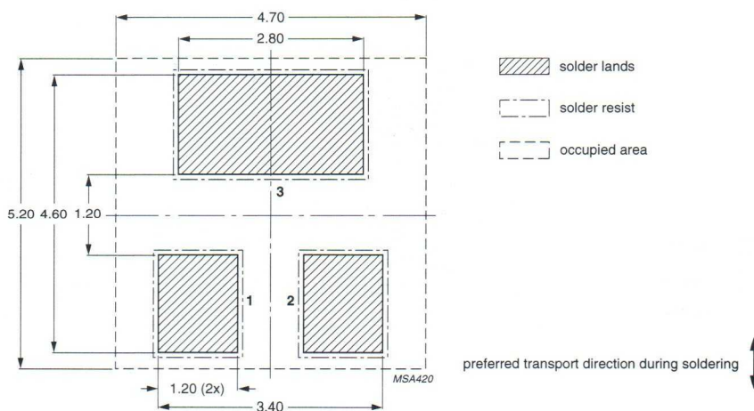
Fig.46 Wave soldering footprint for SOT346 (SC-59).
