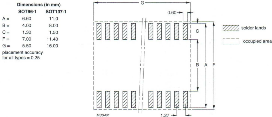
Fig.31 Reflow soldering footprint for SOT96-1 (SO8) and SOT137-1 (SO24).
