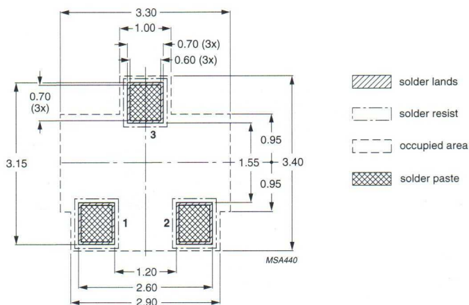
Fig.45 Reflow soldering footprint for SOT346 (SC-59).
