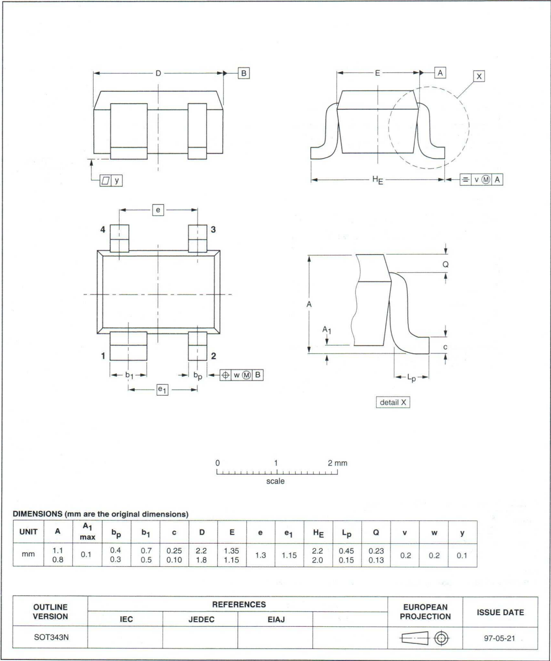
Plastic surface mounted package; 4 leads
