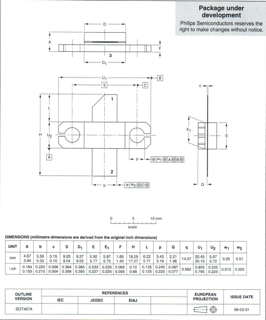
Flanged LDMOST package; 2 mounting holes; 2 leads
