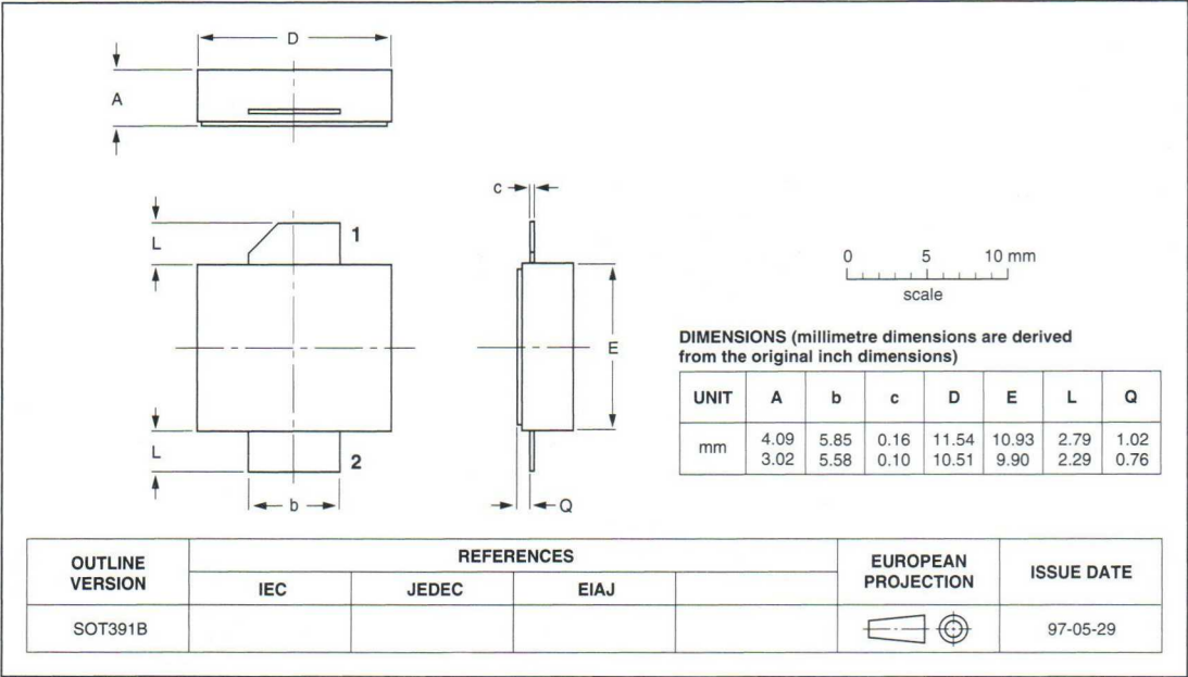
Flangeless ceramic package; 2 leads
