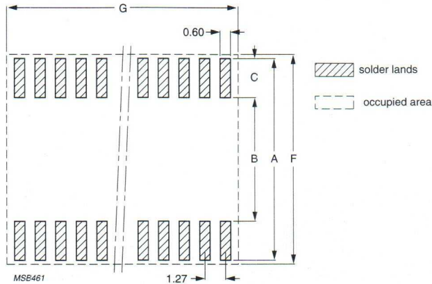
Fig.35 Reflow soldering footprint for SOT163-1 (SO20).
