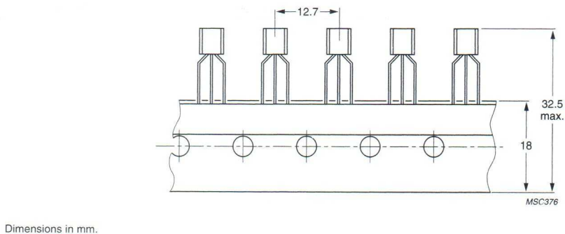
Fig.18 Radial taped components for ammo pack.
