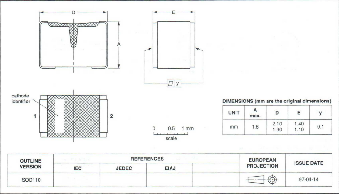
Very small ceramic rectangular surface mounted package
