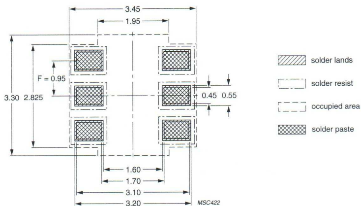
Fig.56 Reflow soldering footprint for SOT457 (SC-74).
