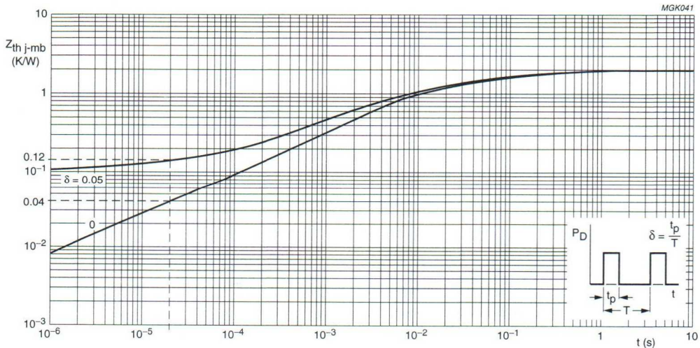
Fig.12 Thermal impedance curves for \delta = 0.05 and \delta = 0 .
