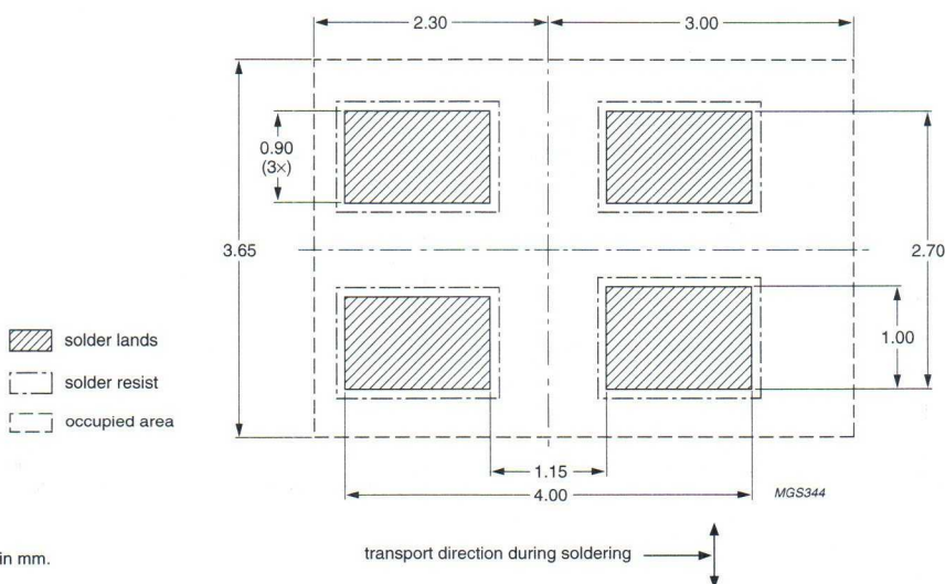
Fig.44 Wave soldering footprint for SOT343N (footprint for SOT343R is mirror image).
