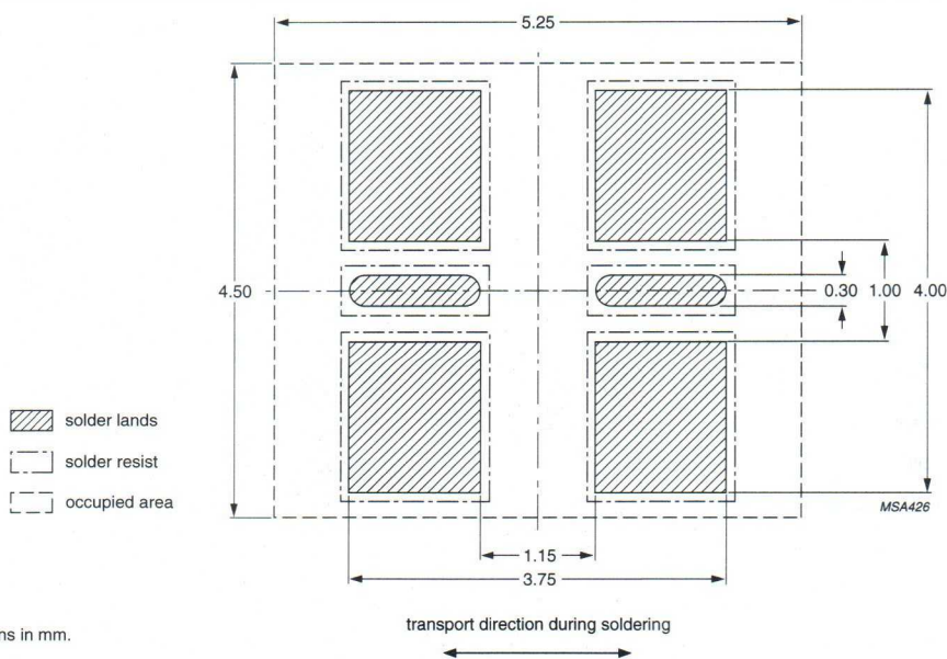
Fig.50 Wave soldering footprint for SOT363 (SC-88).
