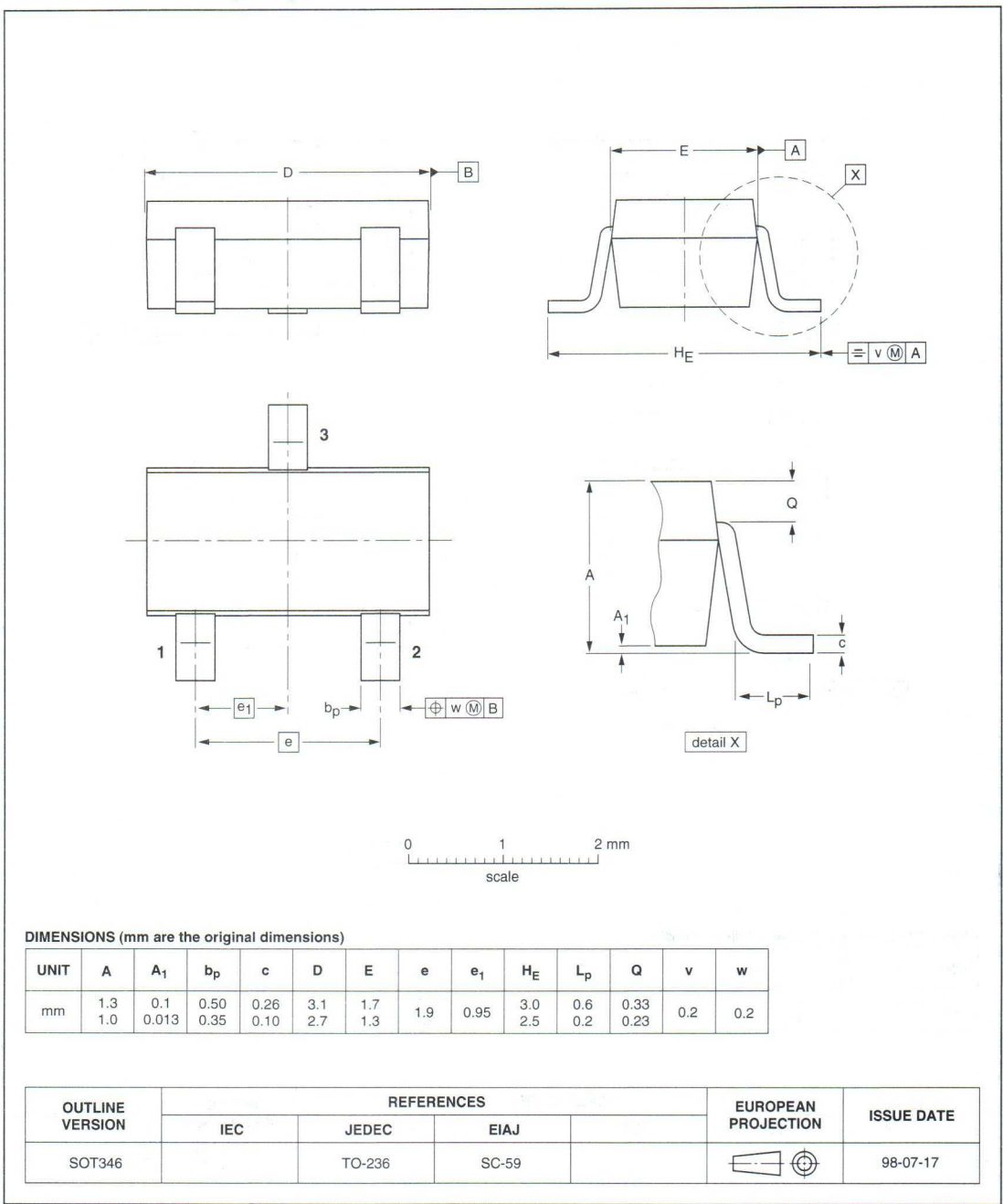
Plastic surface mounted package; 3 leads SOT346
