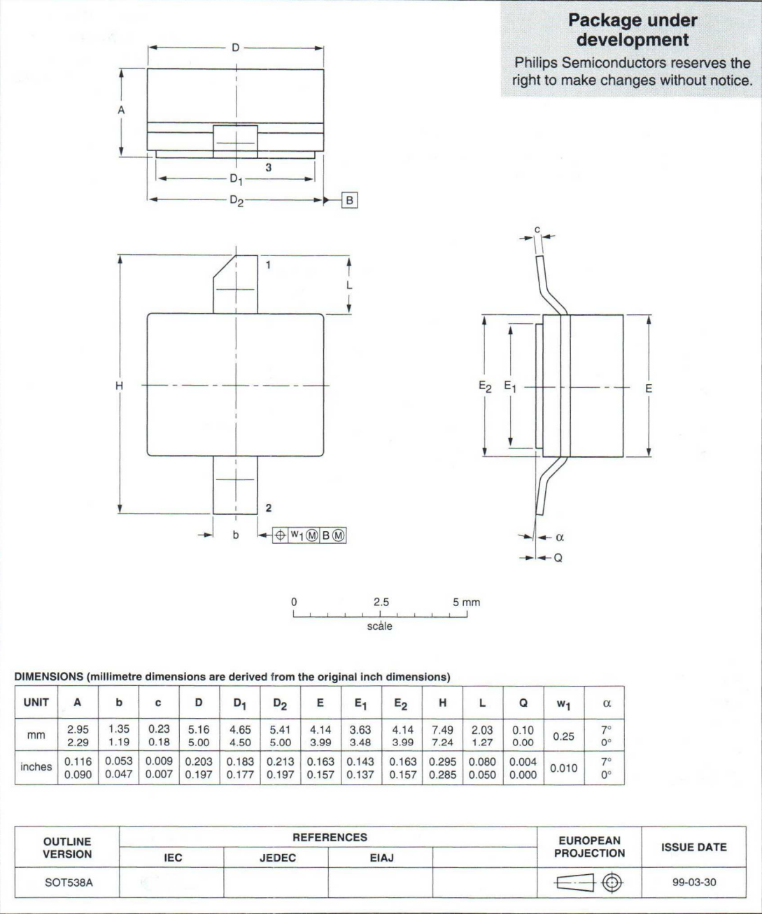
Ceramic surface mounted package; 2 leads
