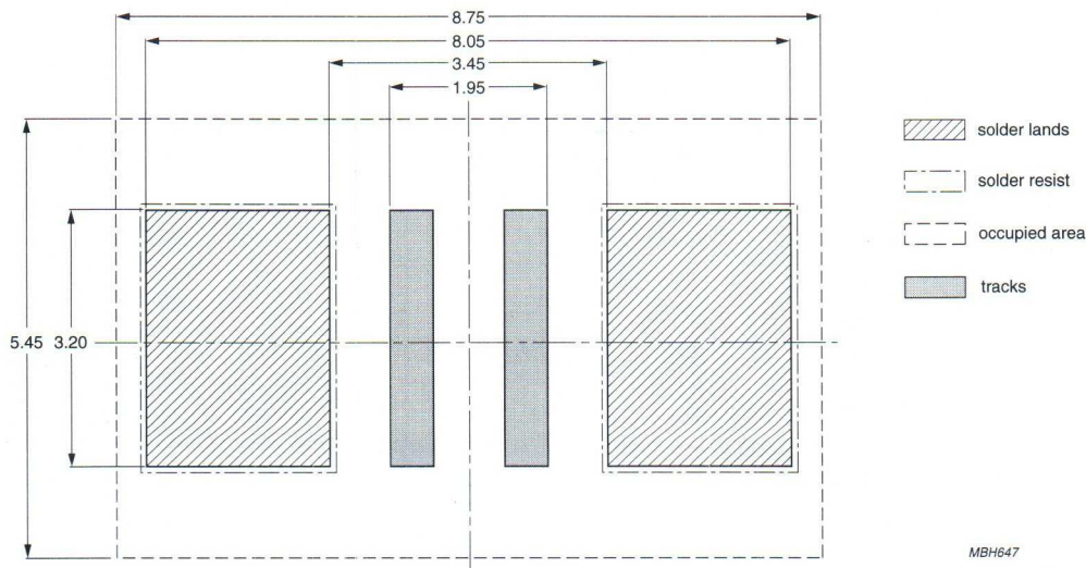
Fig.21 Wave soldering footprint for SOD106.
