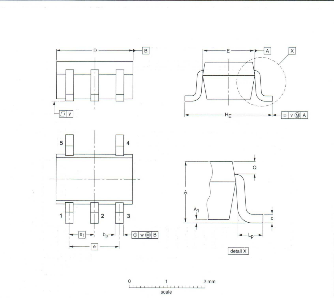
Plastic surface mounted package; 5 leads
