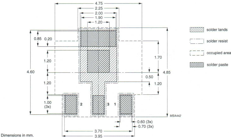
Fig.29 Reflow soldering footprint for SOT89 (SC-62).
