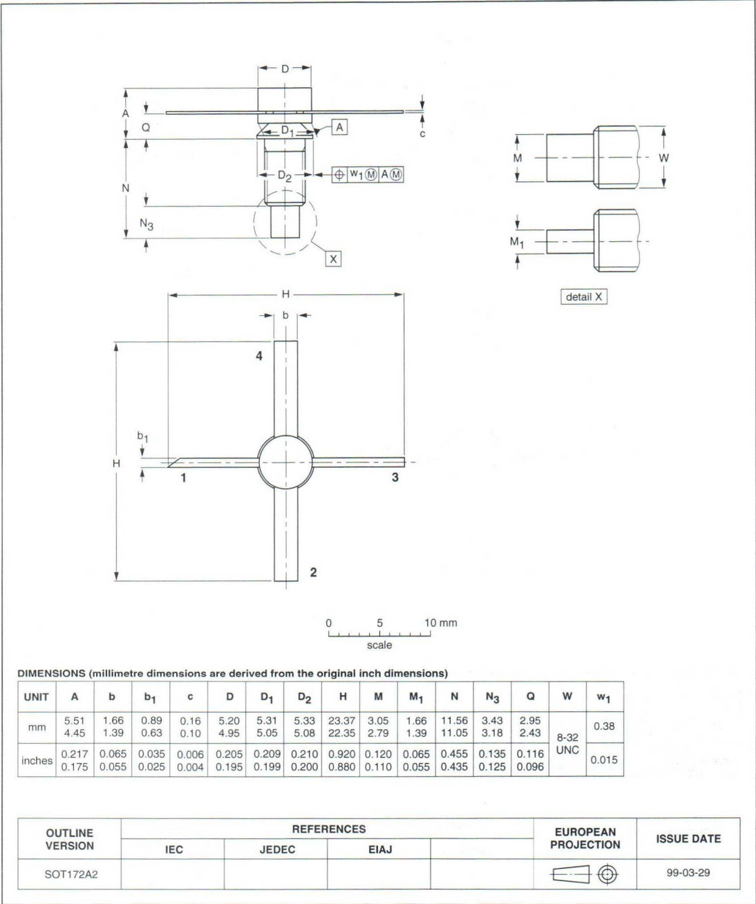
Studded ceramic package; 4 leads
