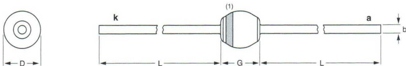
DIMENSIONS (mm are the original dimensions)
