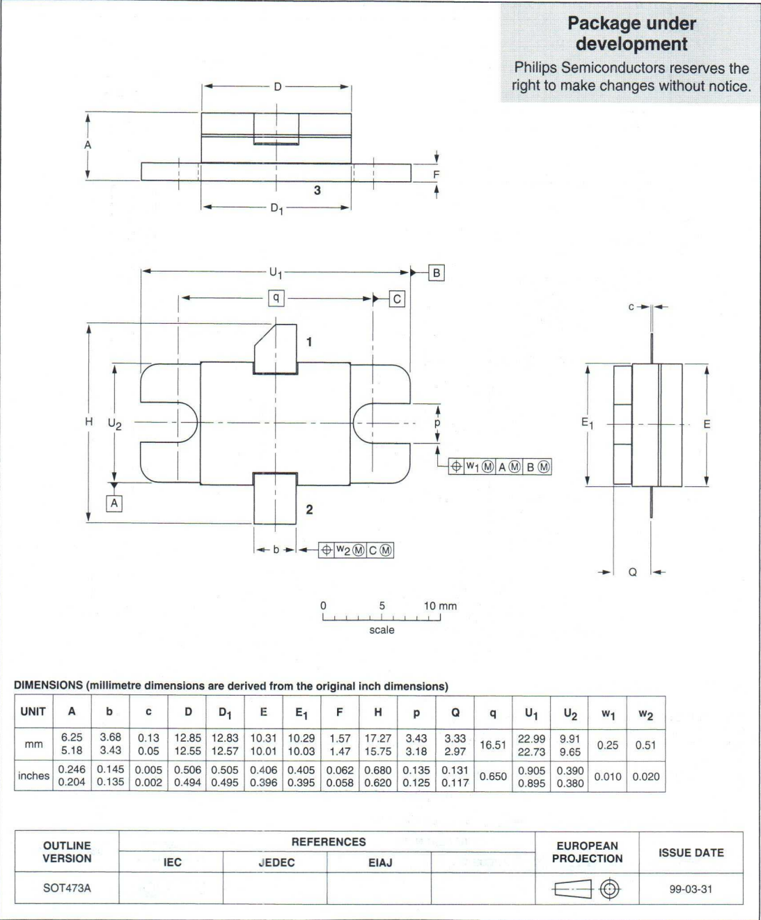
Flanged ceramic package; 2 mounting holes; 2 leads
