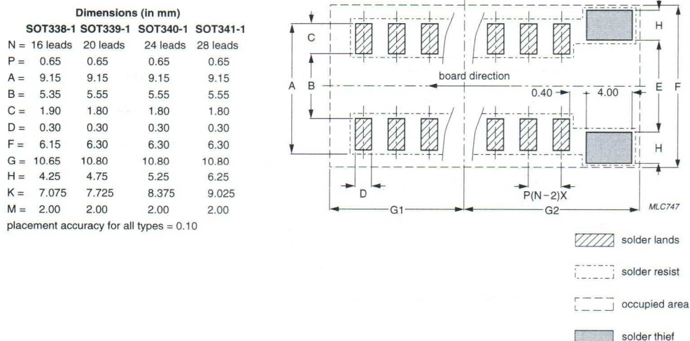
Fig.42 Wave soldering footprint for SOT338-1 (SSOP16), SOT339-1 (SSOP20), SOT340-1 (SSOP24) and SOT34-1 (SSOP28).
