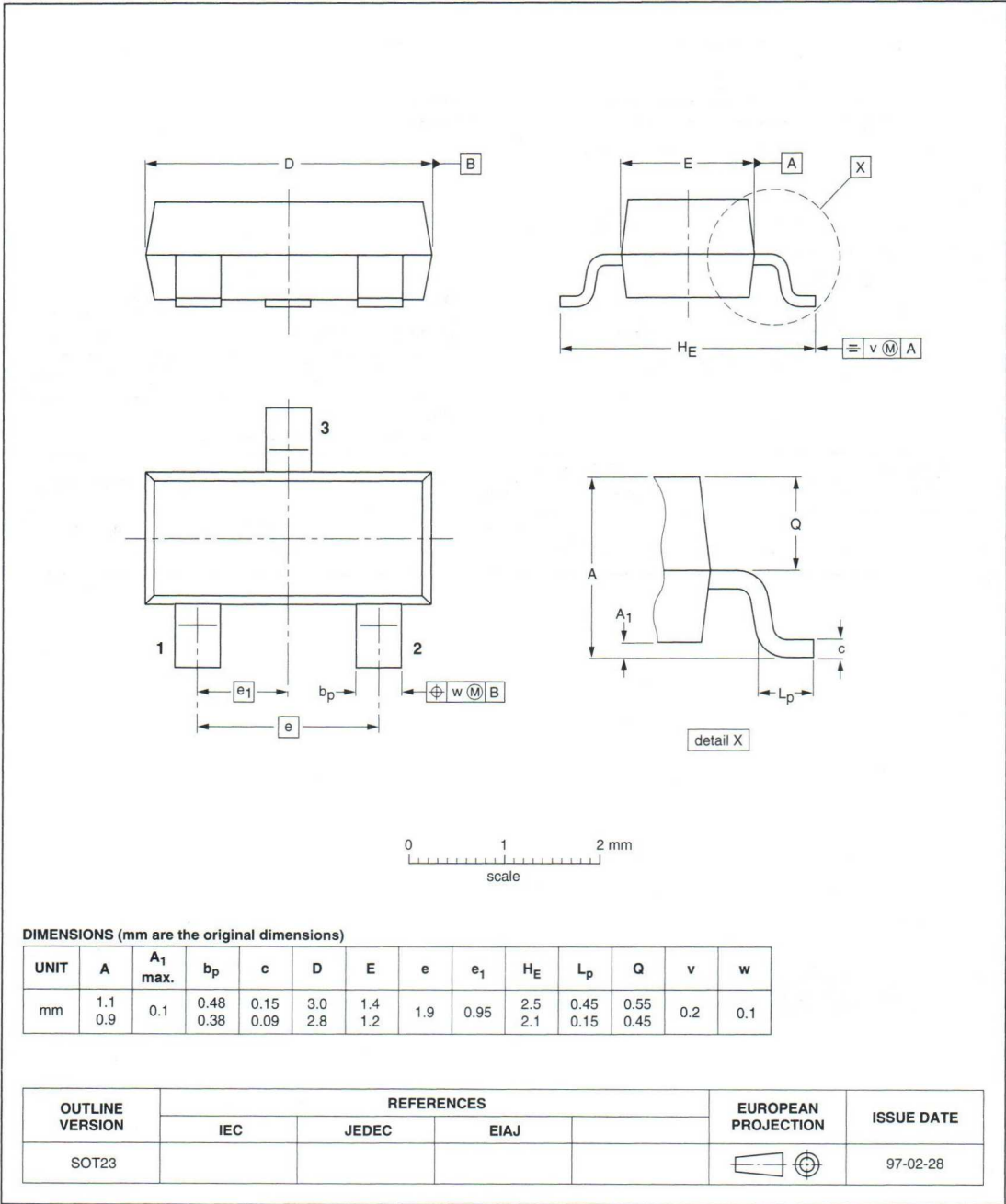
Plastic surface mounted package; 3 leads
