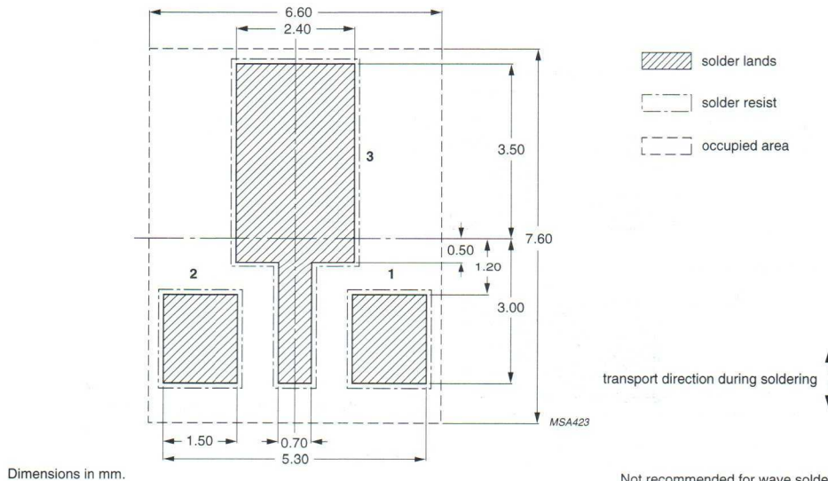
Fig.30 Wave soldering footprint for SOT89 (SC-62).
