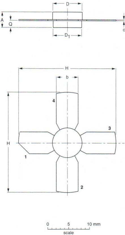
DIMENSIONS (millimetre dimensions are derived from the original inch dimensions)
