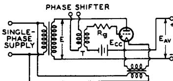
FIG. 3 HALF-WAVE SINGLE-PHASE
