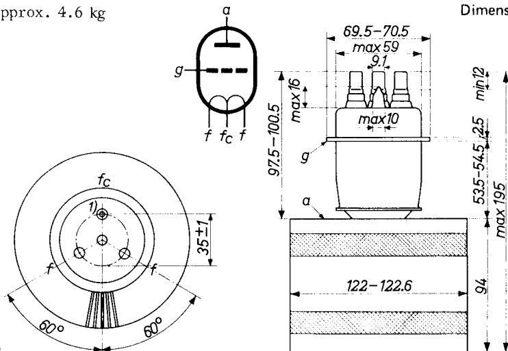
Fig. 1 Mechanical outline.
