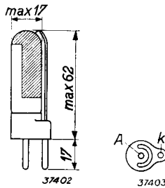
Electrode connections, and maximum dimensions in millimetres.
