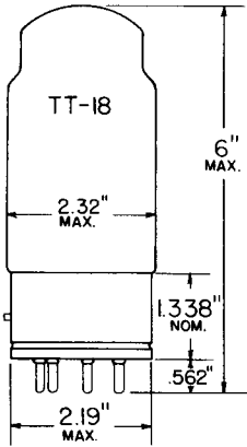
GLASS BULB
