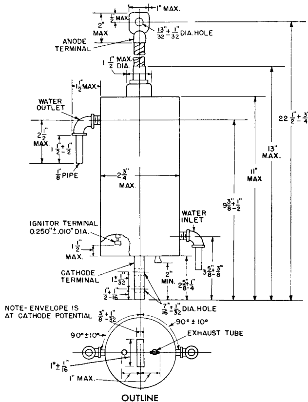
OUTLINE FG-271 IGNITRON
