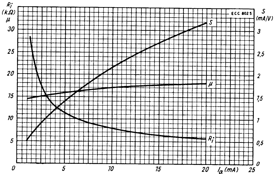
S, R_j, \mu = f(I_a), U_a = 250 \text{ V}
