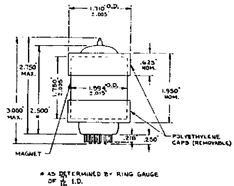
Figure 1 Outline Drawing
