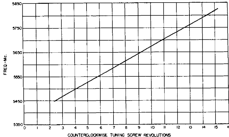
COUNTERCLOCKWISE TUNING SCREW REVOLUTIONS FIG. 10-TUNING CHARACTERISTICS OF TYPICAL RK 7156 MAGNETRON
